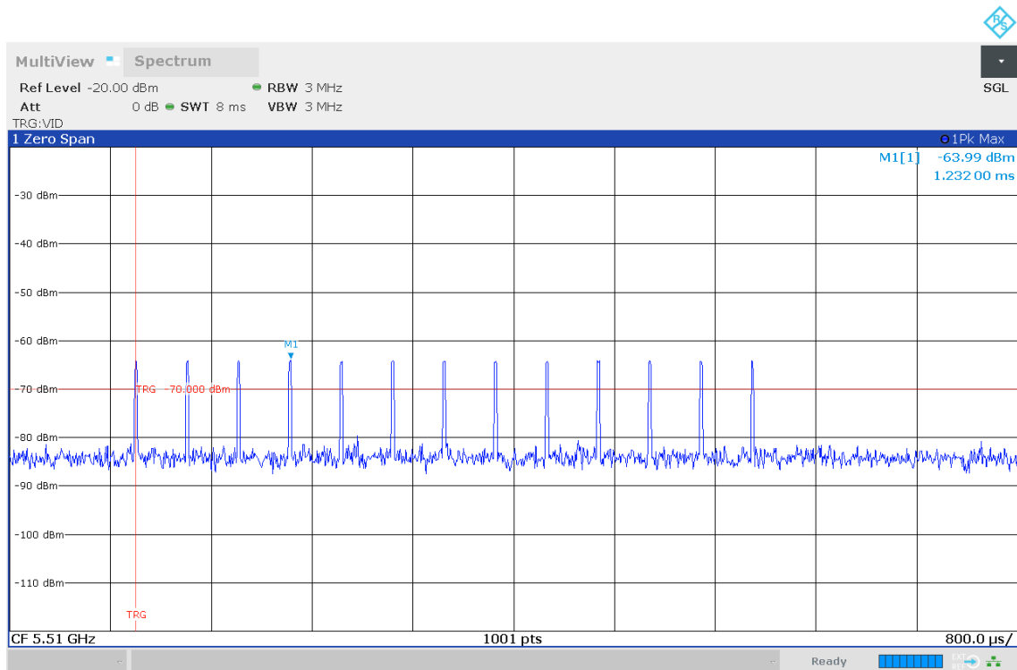
Pulse Type 4
