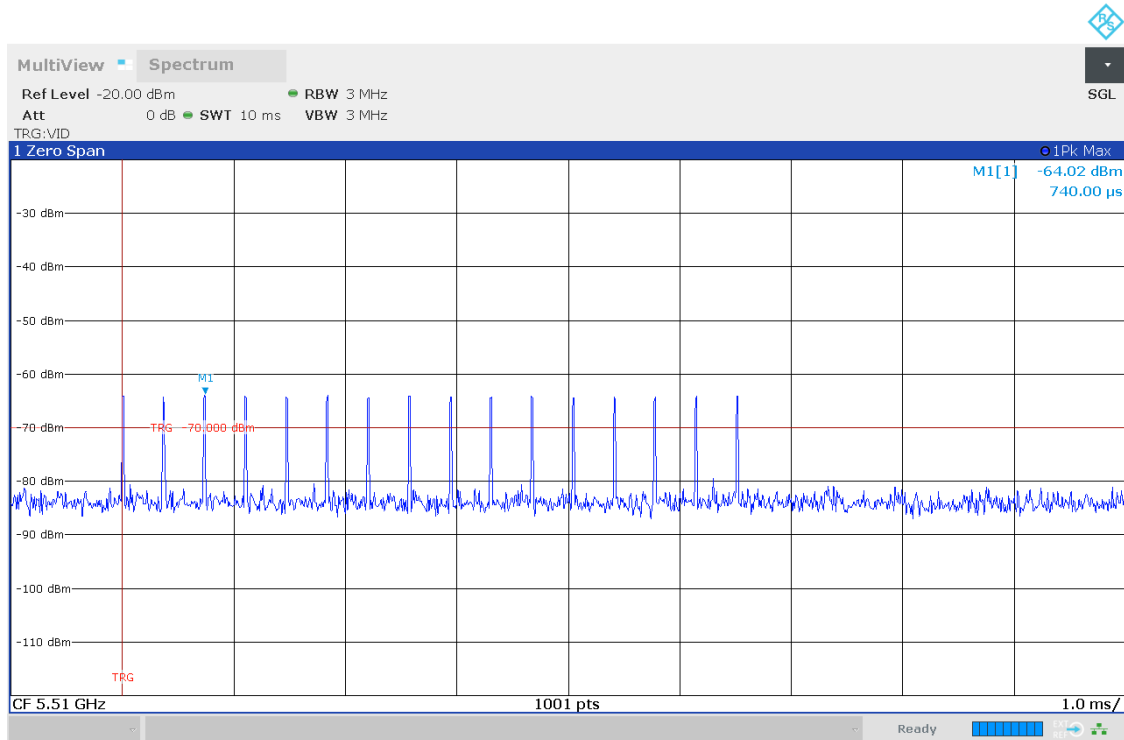
Pulse Type 3
