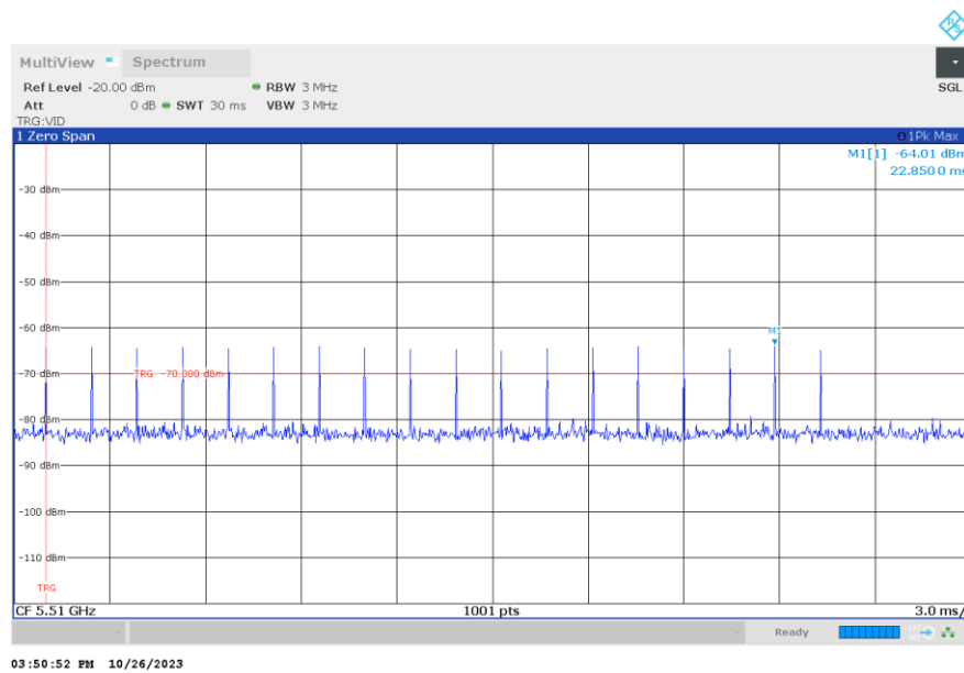
Pulse Type 0
