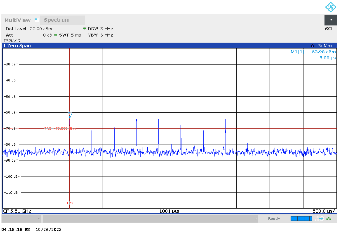
Pulse Type 6
