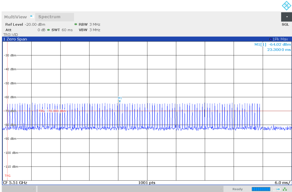
Pulse Type 1
