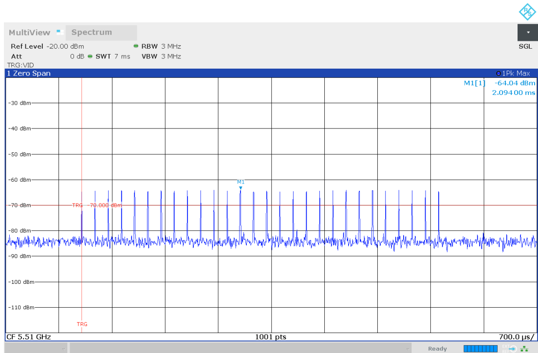
Pulse 2
