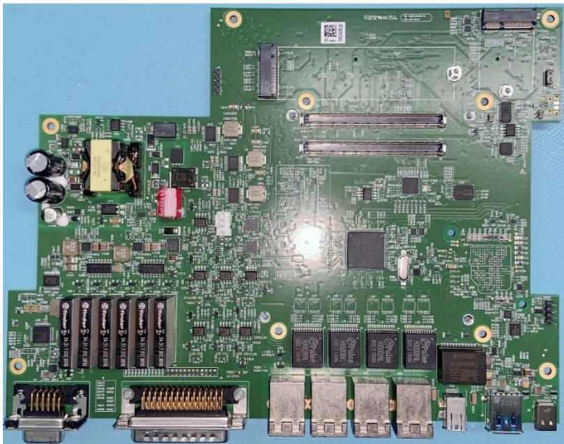
Figure 13: X68 Board PCBA top 3
