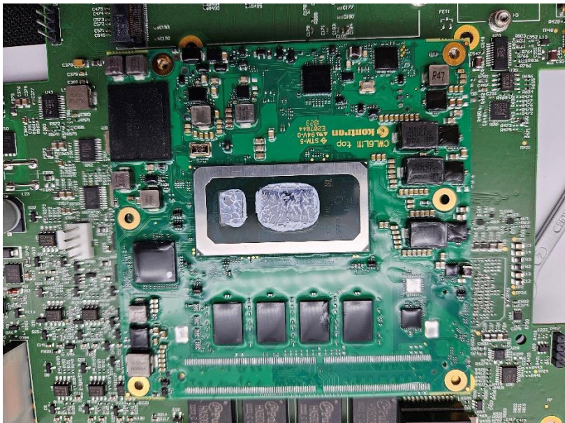
Figure 11: X86 Board PCBA top 2
