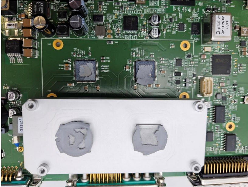
Figure 8: Base board PCBA top 2
