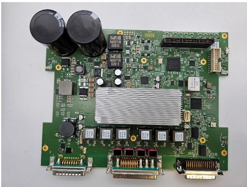
Figure 7: Base board PCBA top
