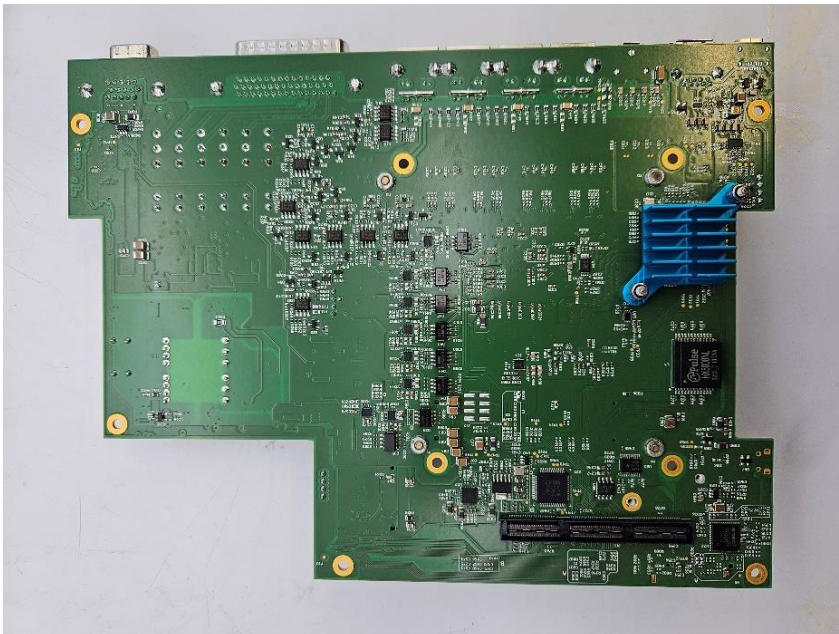
Figure 1817: X86 Board PCBA bottom
