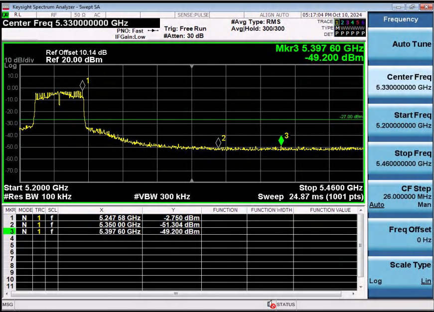
11AC40SISO-Ant1-5230-PASS
