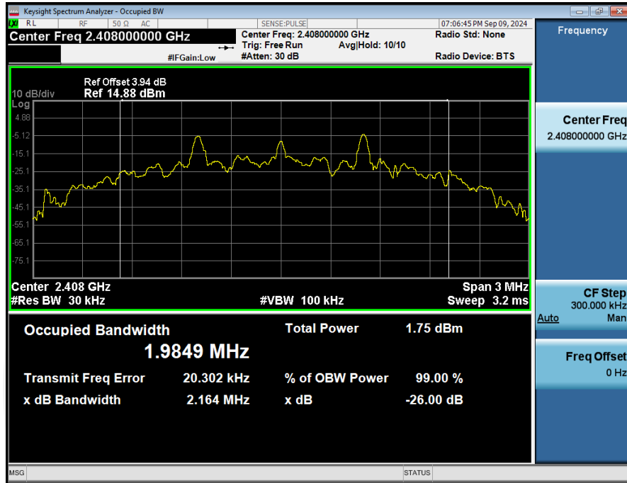
99%_Occupied_Bandwidth_NVNT_ANT1_User_2408_00
