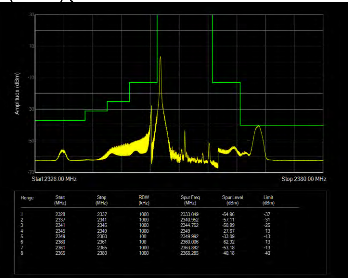
Band40(2350-2360) QPSK BW=10MHz Channel=39200 RB Size=1 Position=#0 Normal
