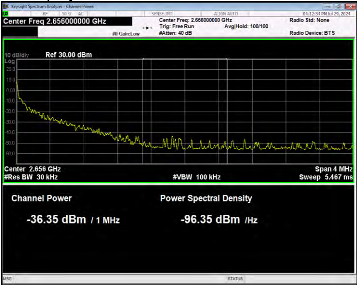
Band41(2535-2655) 16QAM BW=20MHz Channel=41140 RB Size=1 Position=#Max Normal
