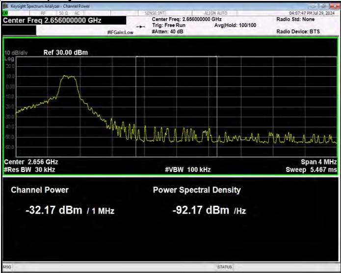
Band41(2535-2655) 16QAM BW=5MHz Channel=41215 RB Size=1 Position=#Max Normal
