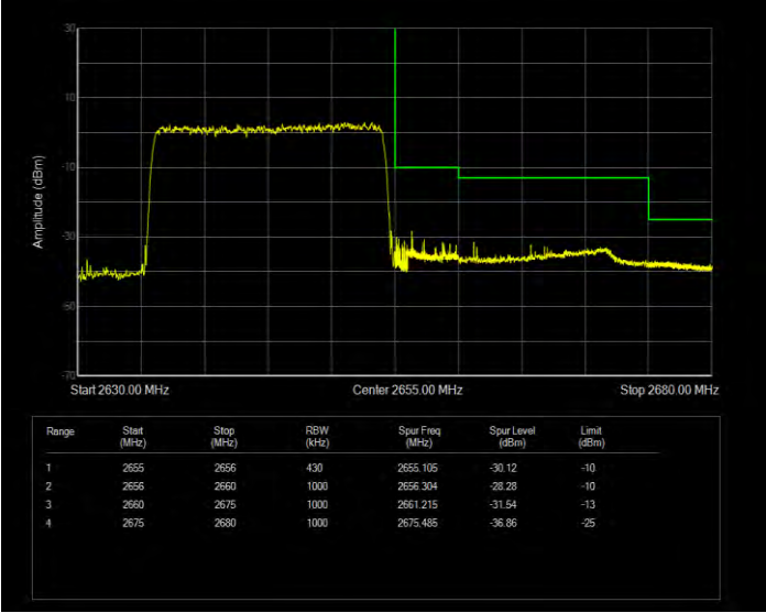
Band41(2535-2655) QPSK BW=5MHz Channel=40065 RB Size=1 Position=#0 Extended
