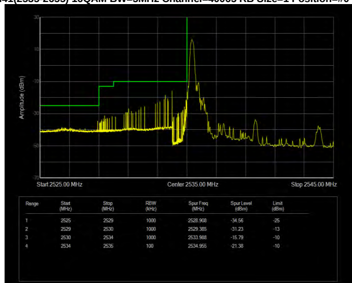
Band41(2535-2655) 16QAM BW=5MHz Channel=40065 RB Size=1 Position=#0 Normal
