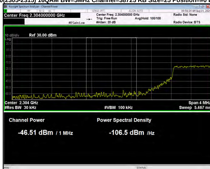
Band40(2305-2315) 16QAM BW=5MHz Channel=38725 RB Size=25 Position=#0 Normal
