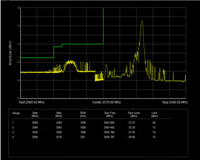
Band38 QPSK BW=5MHz Channel=37775 RB Size=25 Position=#0 Extended
