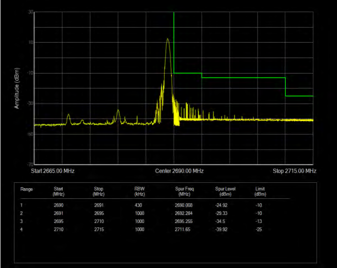
Band41 16QAM BW=20MHz Channel=41490 RB Size=100 Position=#0 Extended
