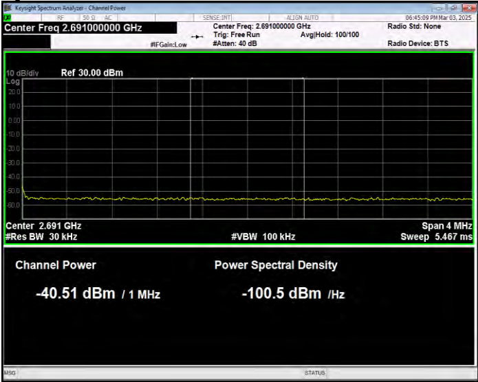
Band41 QPSK BW=20MHz Channel=41490 RB Size=1 Position=#0 Normal
