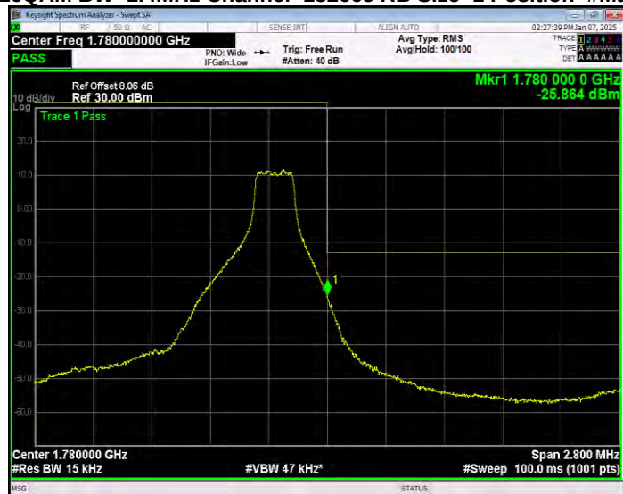
Band66 16QAM BW=1.4MHz Channel=132665 RB Size=6 Position=#0 Extended
