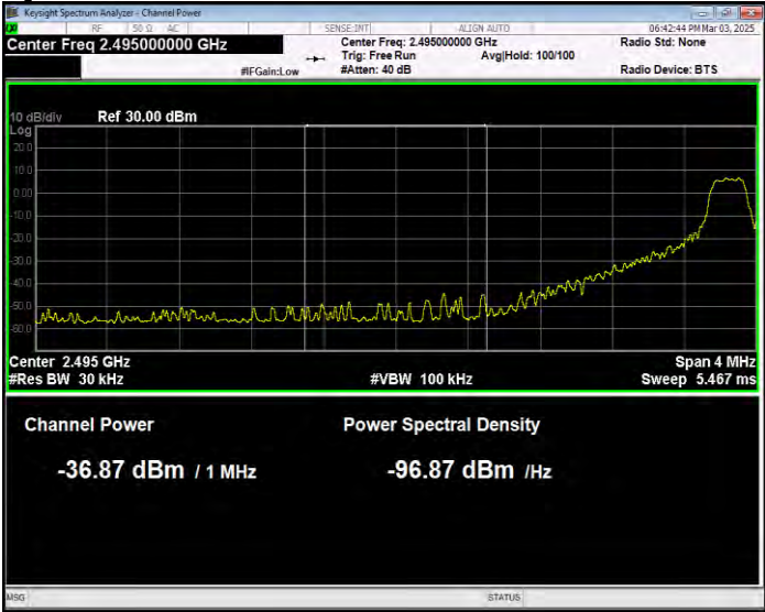
Band41 QPSK BW=15MHz Channel=39725 RB Size=1 Position=#0 Normal
