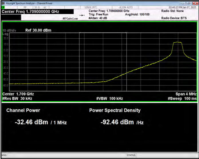
Band66 16QAM BW=10MHz Channel=132022 RB Size=1 Position=#0 Normal
