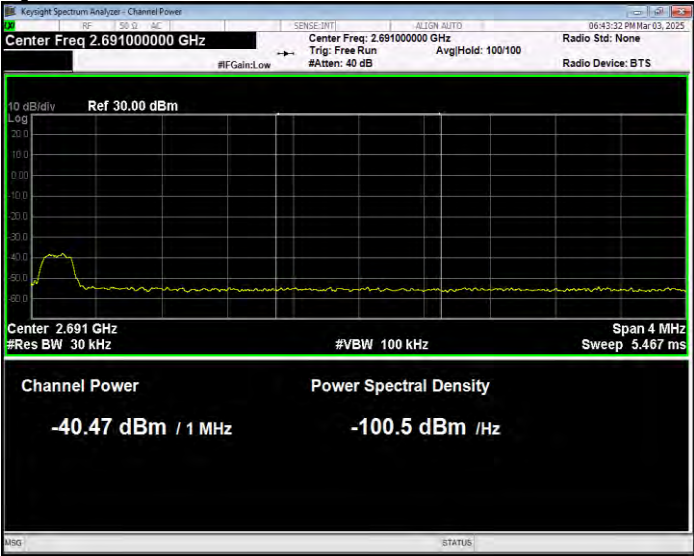
Band41 QPSK BW=15MHz Channel=41515 RB Size=1 Position=#0 Normal
