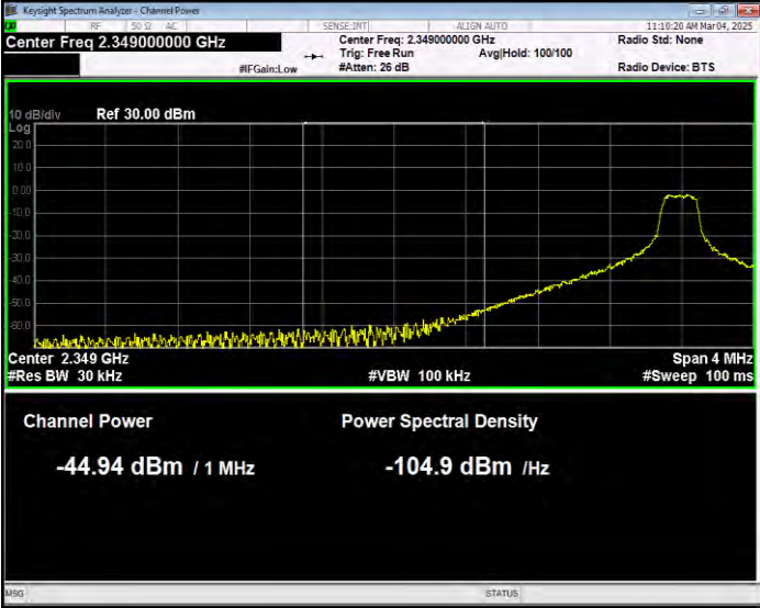
Band40(2350-2360) 16QAM BW=10MHz Channel=39200 RB Size=1 Position=#0 Normal
