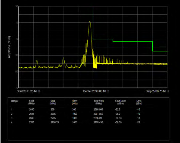
Band41 16QAM BW=15MHz Channel=41515 RB Size=75 Position=#0 Extended
