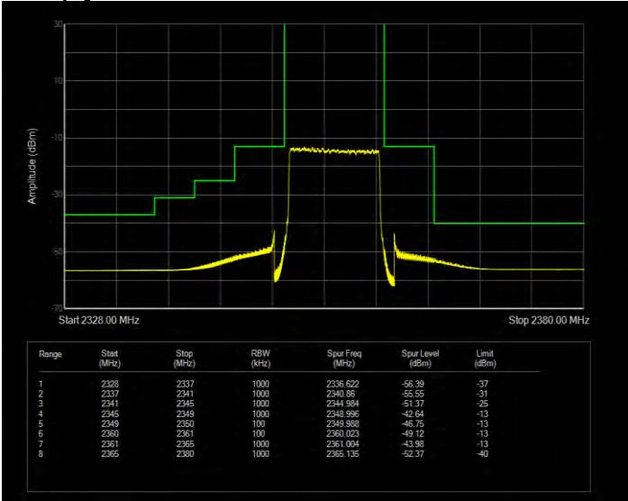
Band40(2350-2360) QPSK BW=5MHz Channel=39175 RB Size=1 Position=#0 Extended
