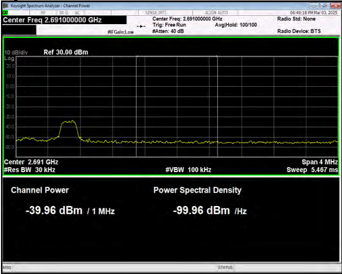
Band41 QPSK BW=5MHz Channel=41565 RB Size=1 Position=#0 Normal
