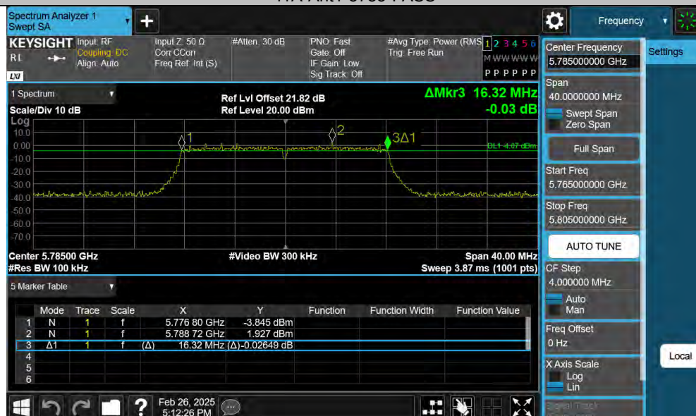
11A-Ant1-5785-PASS
