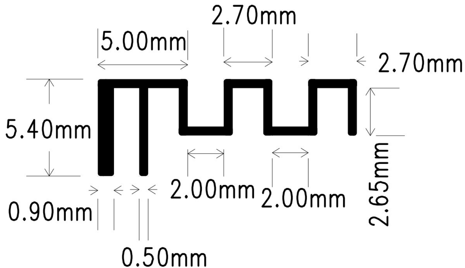
Antenna1 Photo & Length (mm)
