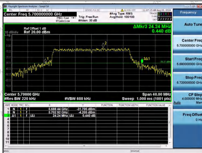
11AC20SISO-Ant1-5700
