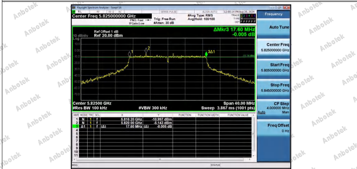
11A-Ant1-5825-PASS
