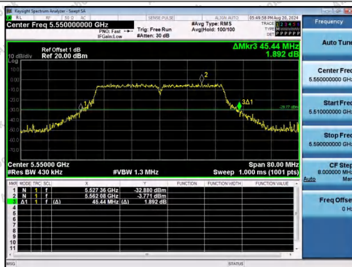
11N40SISO-Ant1-5550
