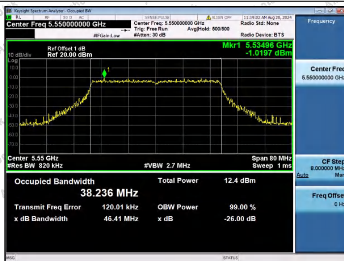
11AC40SISO-Ant1-5550
