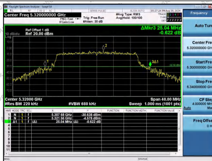
11AC20SISO-Ant1-5320
