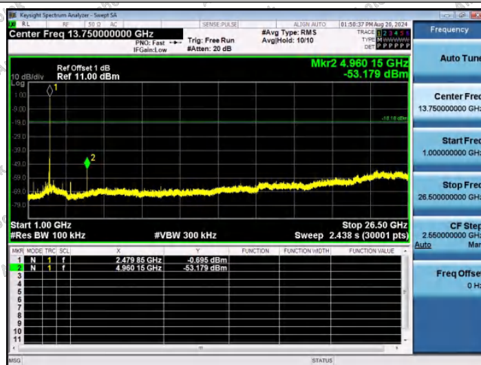
3DH5-Ant1-2480-1000~26500-PASS
