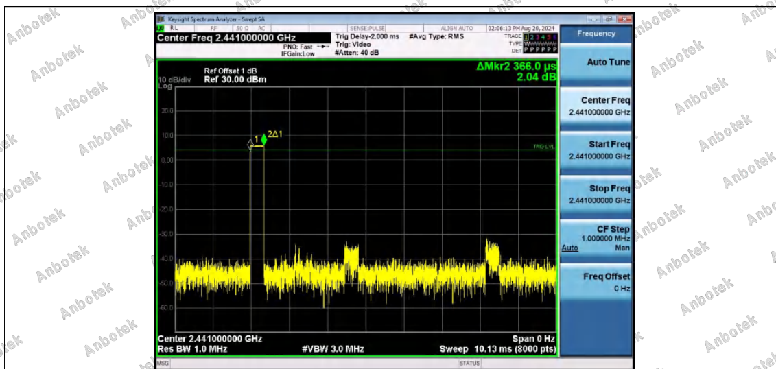
DH1-Ant1-Hop-PASS
