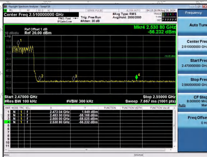
3DH5-Ant1-Hop_2480-PASS
