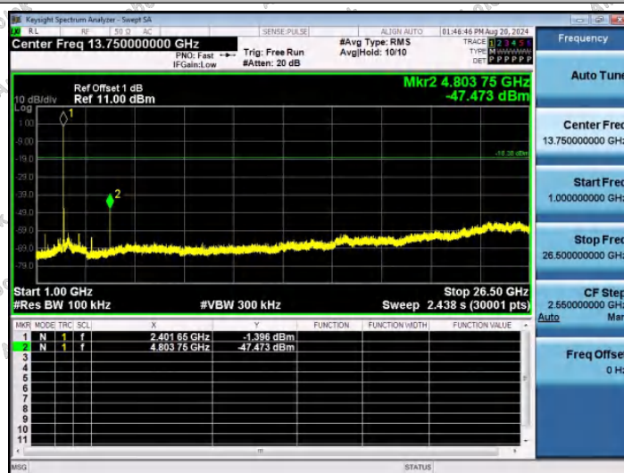
3DH5-Ant1-2402-1000~26500-PASS
