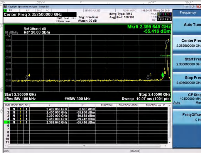
2DH5-Ant1-2402-PASS
