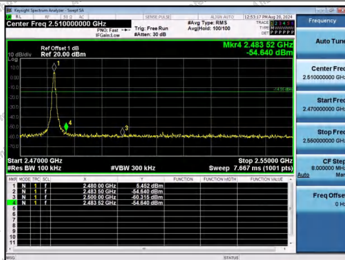
DH5-Ant1-2480-PASS
