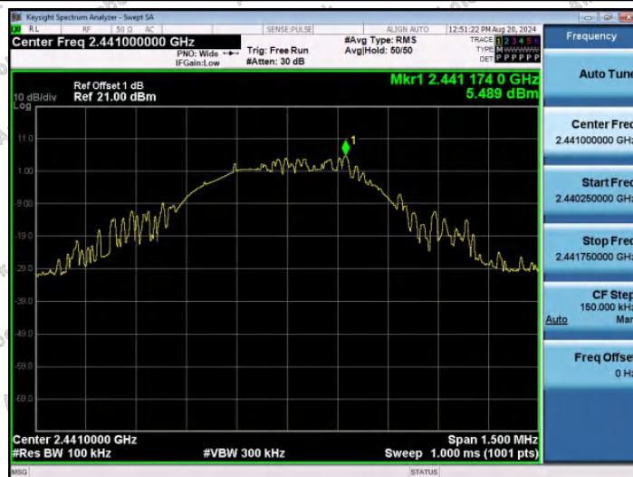
DH5-Ant1-2441-0~Reference-PASS
