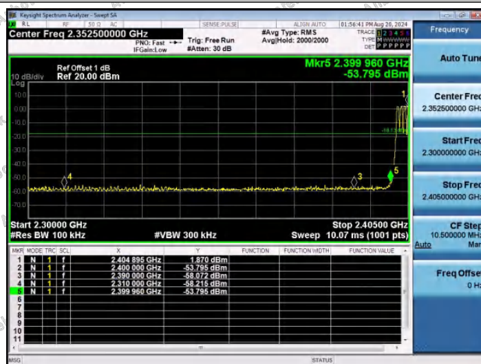
DH5-Ant1-Hop 2402-PASS
