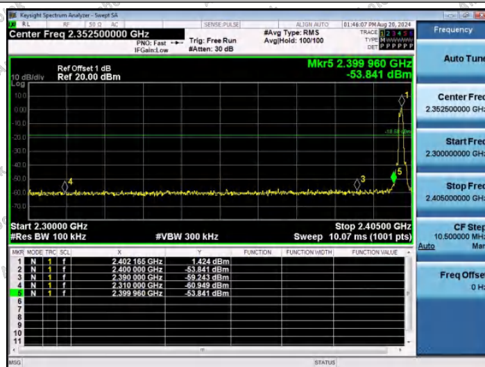
3DH5-Ant1-2402-PASS
