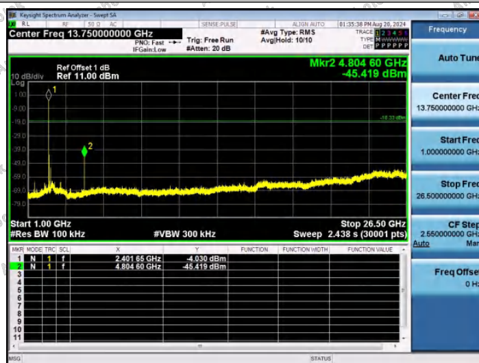
2DH5-Ant1-2402-1000~26500-PASS
