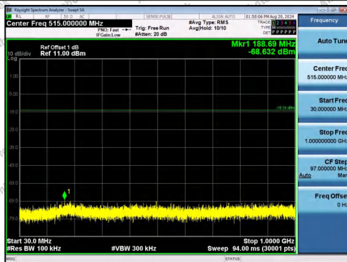
3DH5-Ant1-2480-30~1000-PASS
