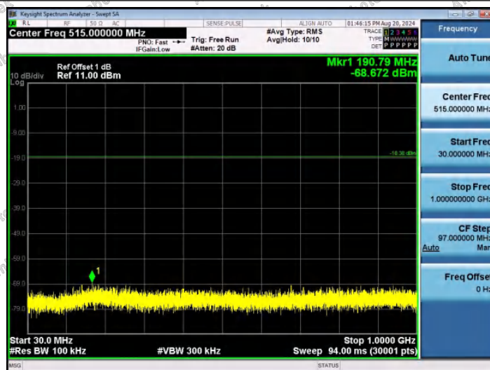
3DH5-Ant1-2402-30~1000-PASS
