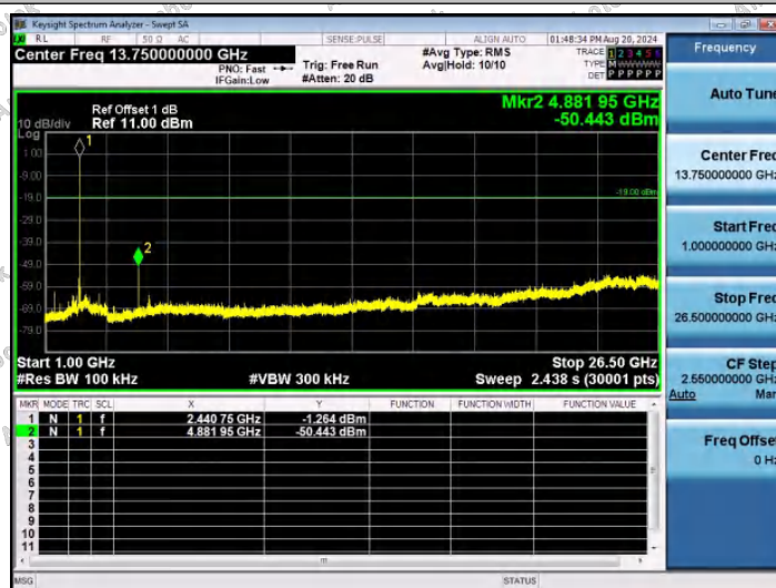
3DH5-Ant1-2441-1000~26500-PASS
