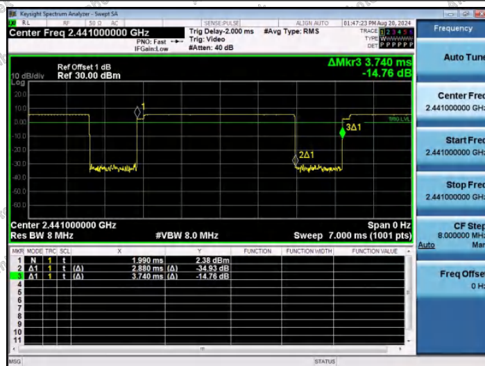
NTVN-3DH5-Ant1-2441
