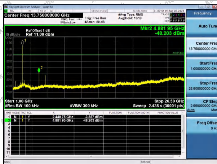
2DH5-Ant1-2441-1000~26500-PASS
