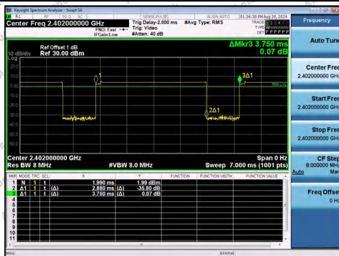
NTVN-2DH5-Ant1-2402
