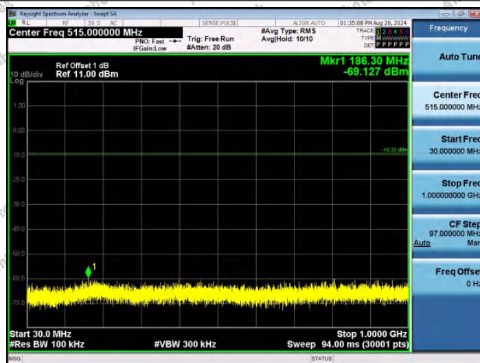
2DH5-Ant1-2402-30~1000-PASS
