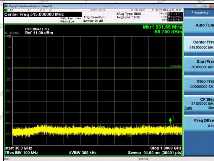
2DH5-Ant1-2441-30~1000-PASS
