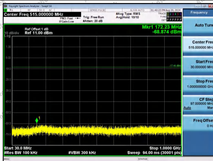
2DH5-Ant1-2480-30~1000-PASS
