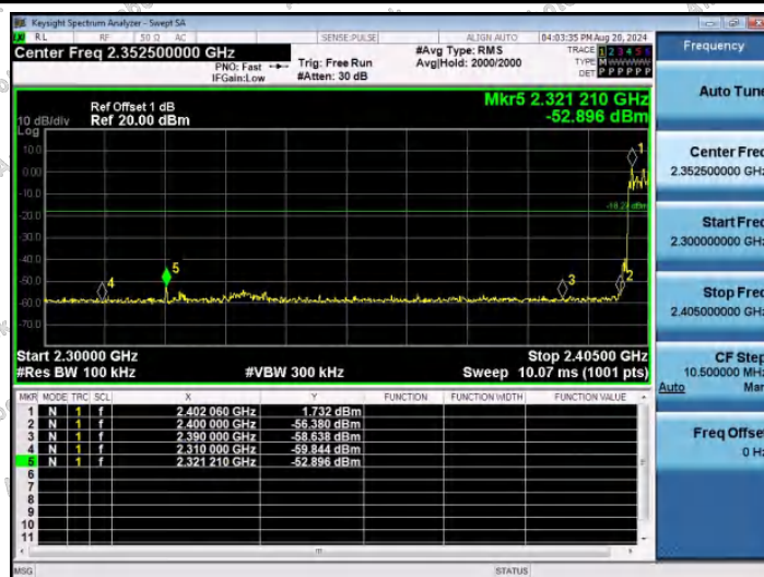
2DH5-Ant1-Hop_2402-PASS
