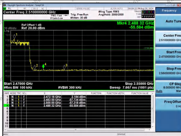
2DH5-Ant1-Hop_2480-PASS
