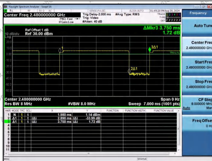
NTVN-3DH5-Ant1-2480
