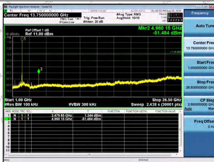
2DH5-Ant1-2480-1000~26500-PASS
