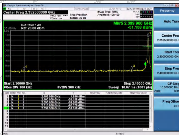
DH5-Ant1-2402-PASS
