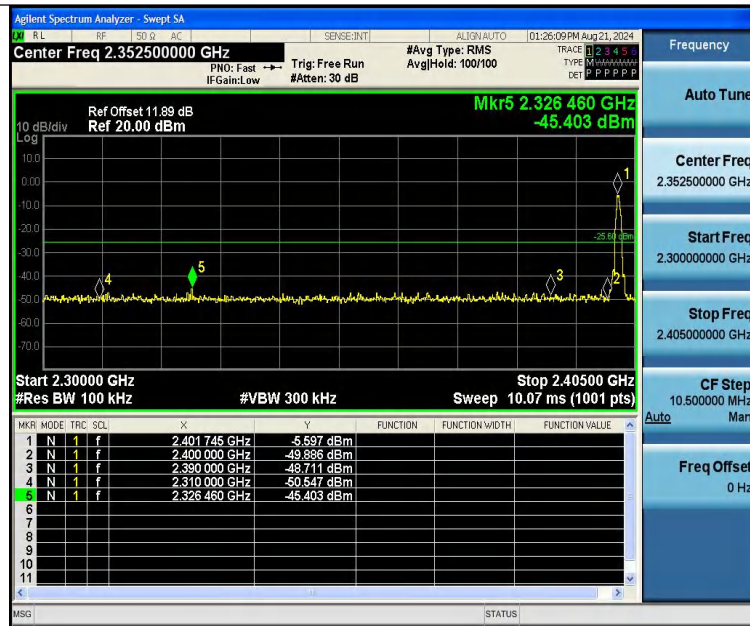
BLE_1M-Ant1-2402-PASS
