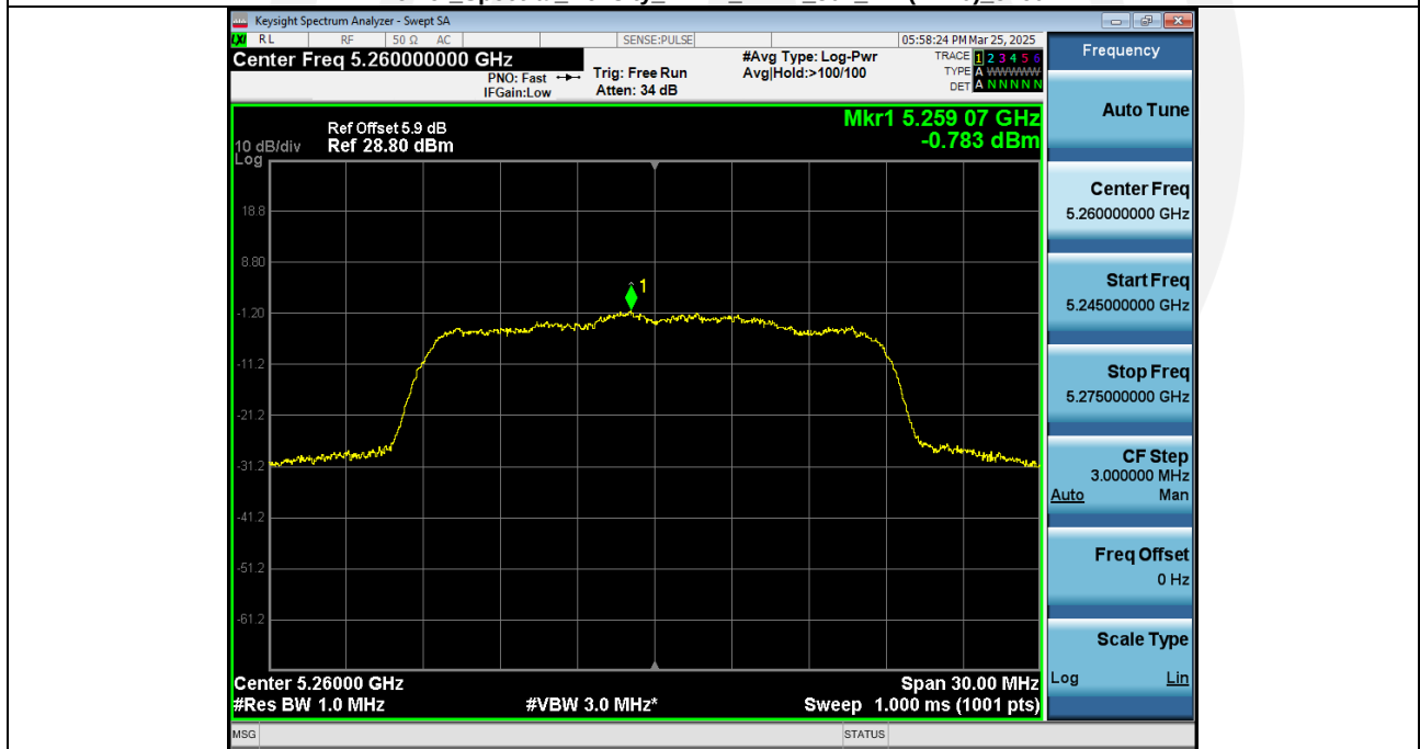
Power Spectral Density NVNT_ANT1_802_11n(HT20)_5260
