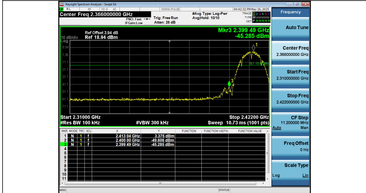
2 Bandedge_NVNT_ANT1_802_11b_2412
