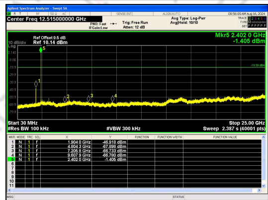
30.0 MHz - 25000.0 MHz Mode1_CH 00
