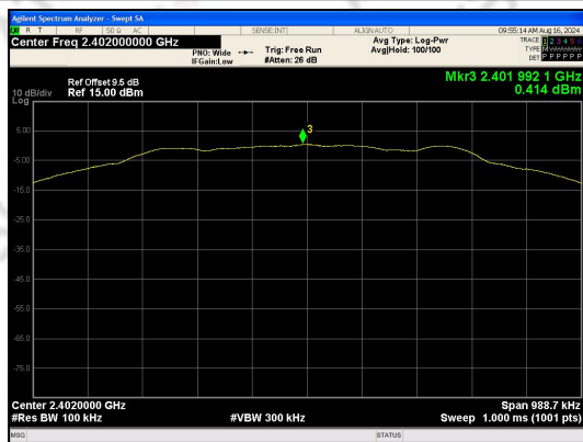
In-Band Reference Level Mode1_CH 00
