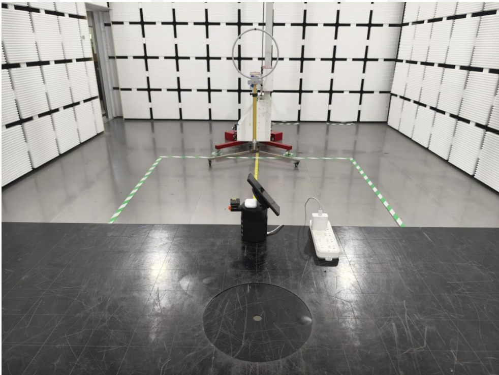
Spurious Radiation Emissions Test (<30MHz)
