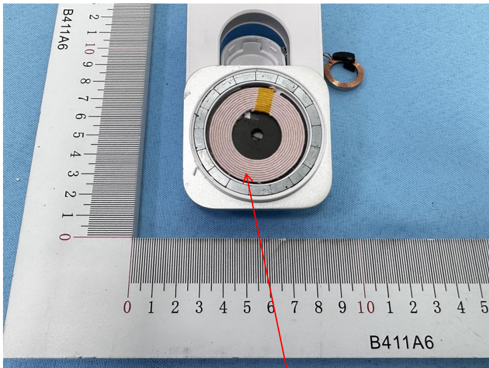
Phone WPT ANT
