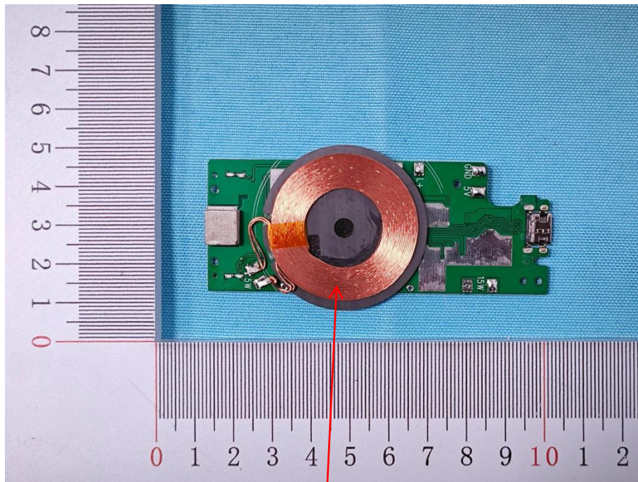
Earbuds WPT ANT
