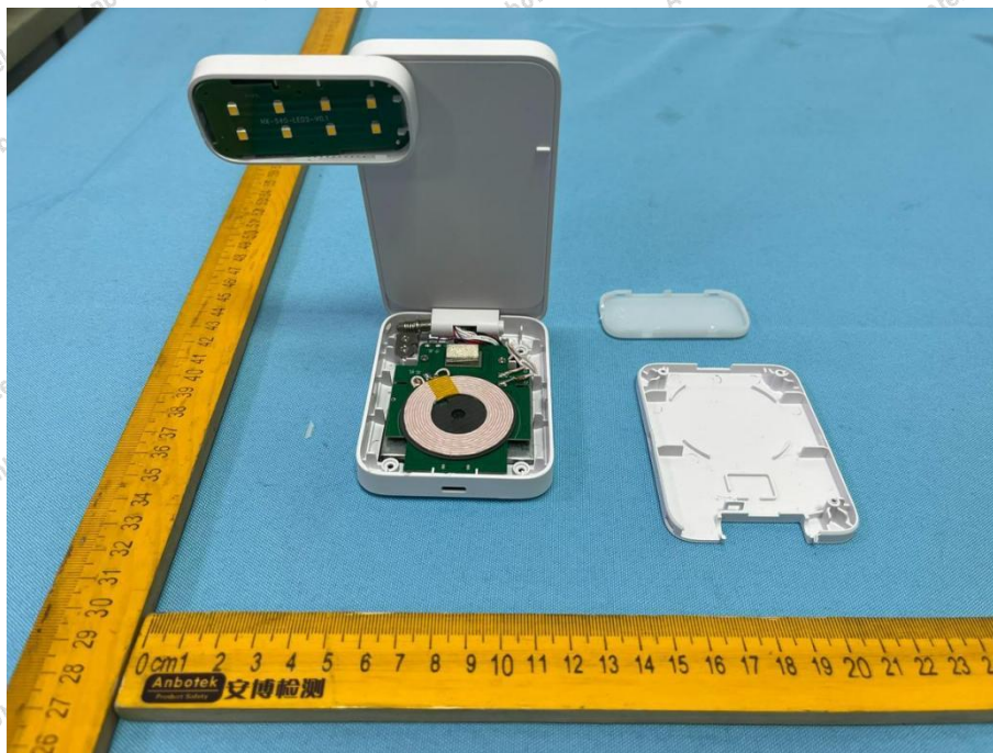
Phone ANT
