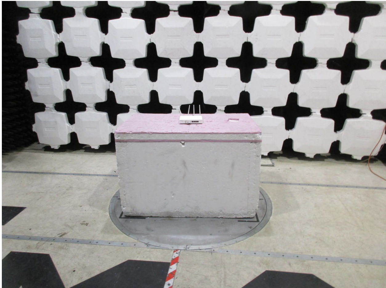
Radiated Testing, Table Setup #1
