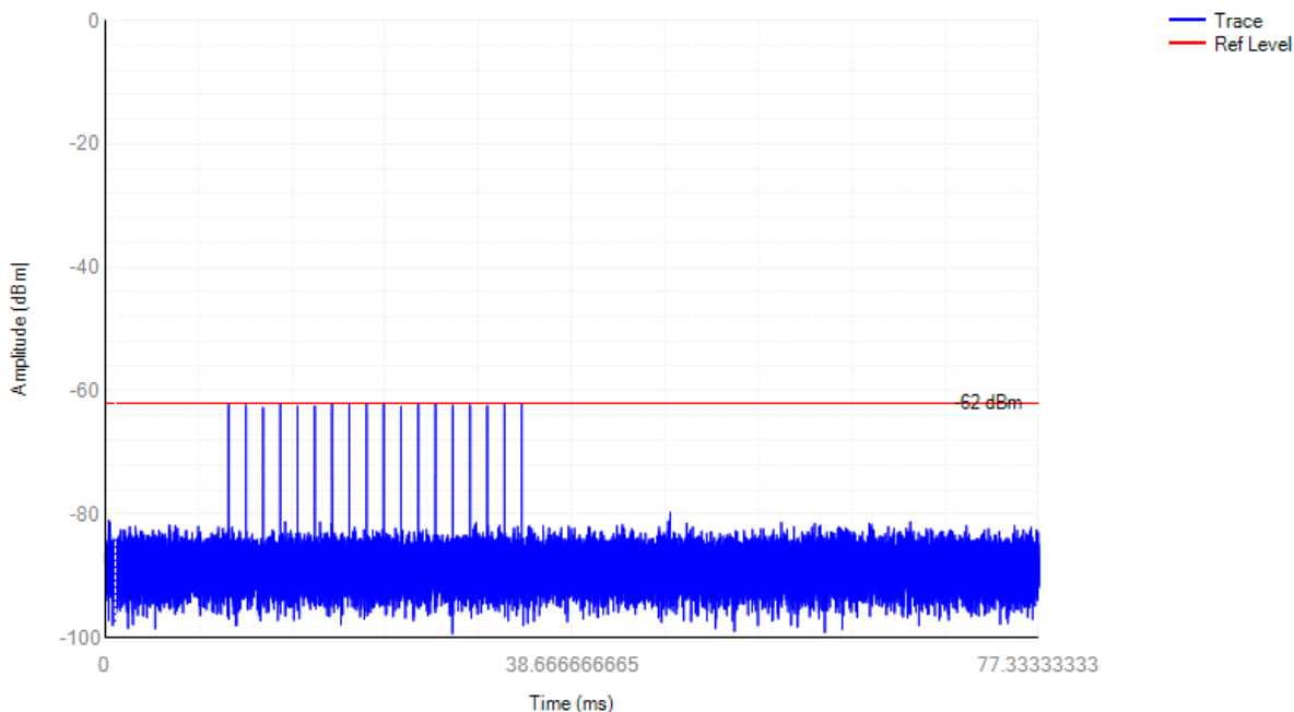
Radar Calibration
