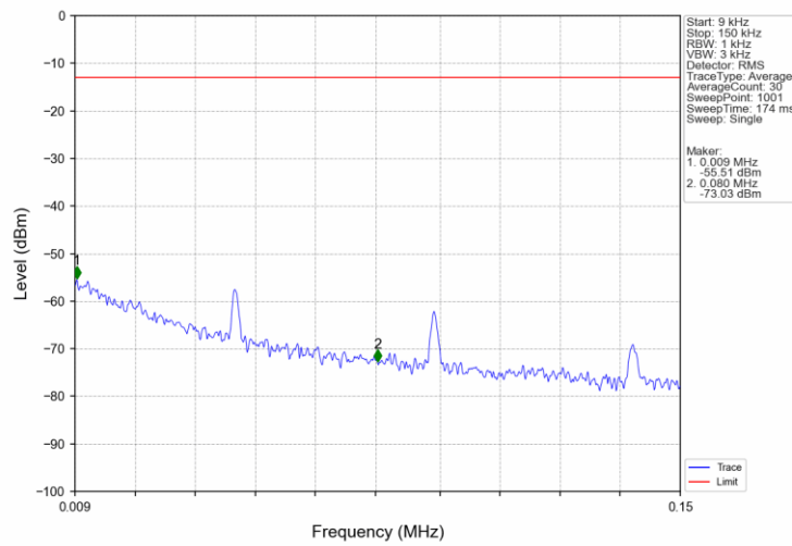
Band5_HSDPA_LCH_826.4MHz_Subtest 1_NTNV
