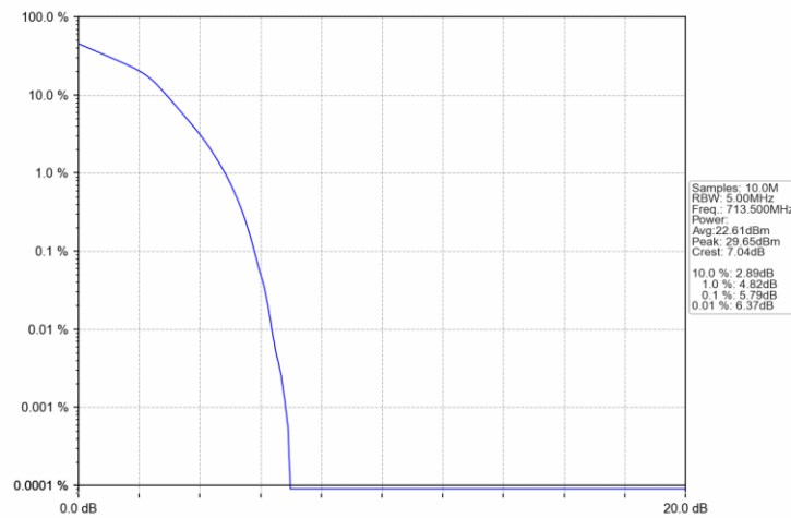
Band17 5MHz 16QAM HCH 713.5MHz RB 25 0 NTNV
