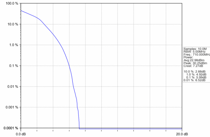
Band17 5MHz 16QAM MCH 710MHz RB 25 0 NTNV
