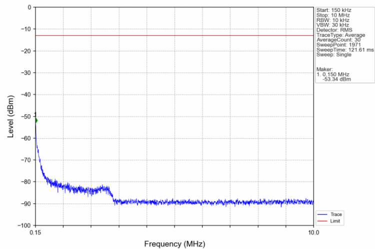
Band12_3MHz_16QAM_MCH_707.5MHz_RB_1_0_NTNV
