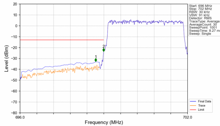
Band12_3MHz_16QAM_LCH_700.5MHz_RB_15_0_NTNV
