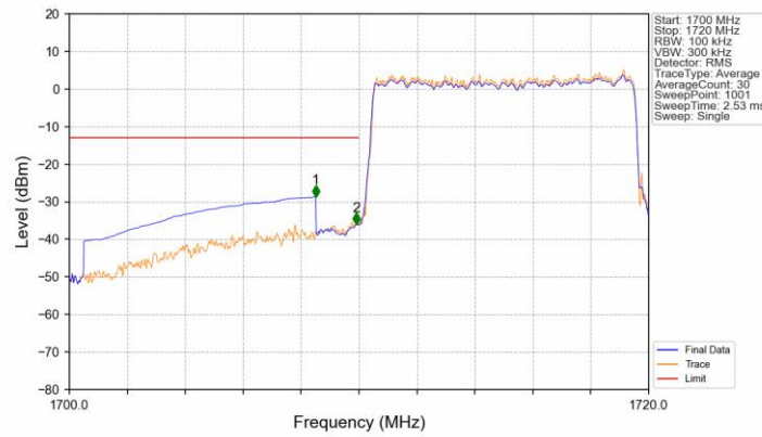
Band4_10MHz_16QAM_LCH_1715MHz_RB_50_0_NTNV
