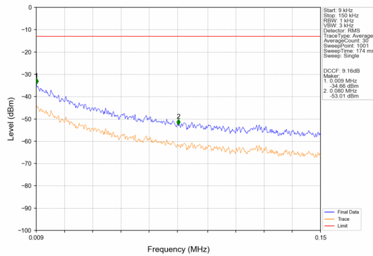
PCS1900_GPRS_MCH_1880MHz_1 TX Slot_NTNV
