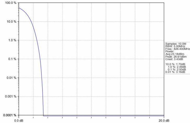
Band5_RMC_LCH_826.4MHz_12.2kbps RMC_NTNV
