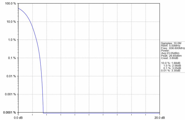
Band5_RMC_MCH_836.6MHz_12.2kbps RMC_NTNV
