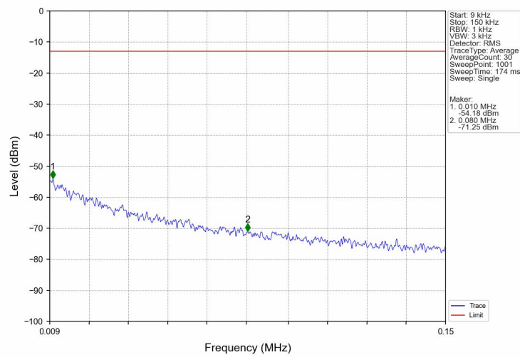
Band4_1.4MHz_QPSK_LCH_1710.7MHz_RB_1_0_NTNV
