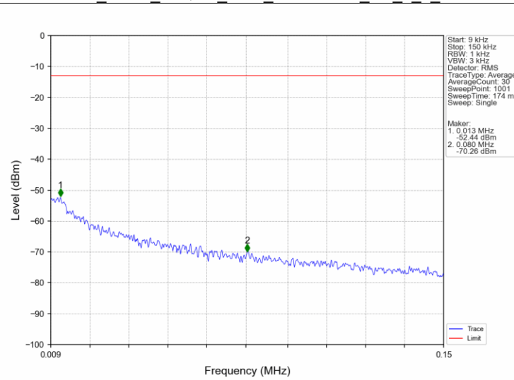
Band4_3MHz_16QAM_HCH_1753.5MHz_RB_1_0_NTNV
