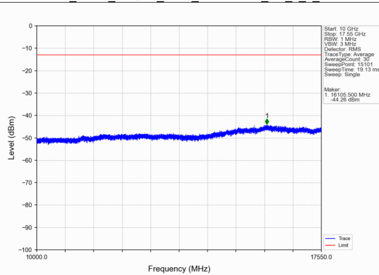
Band4_3MHz_16QAM_MCH_1732.5MHz_RB_1_0_NTNV
