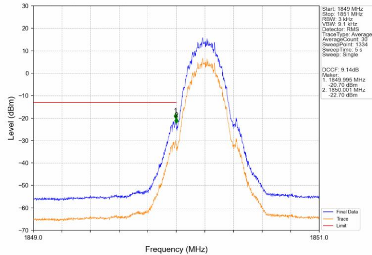
PCS1900_GSM_LCH_1850.2MHz_GSM_NTNV
