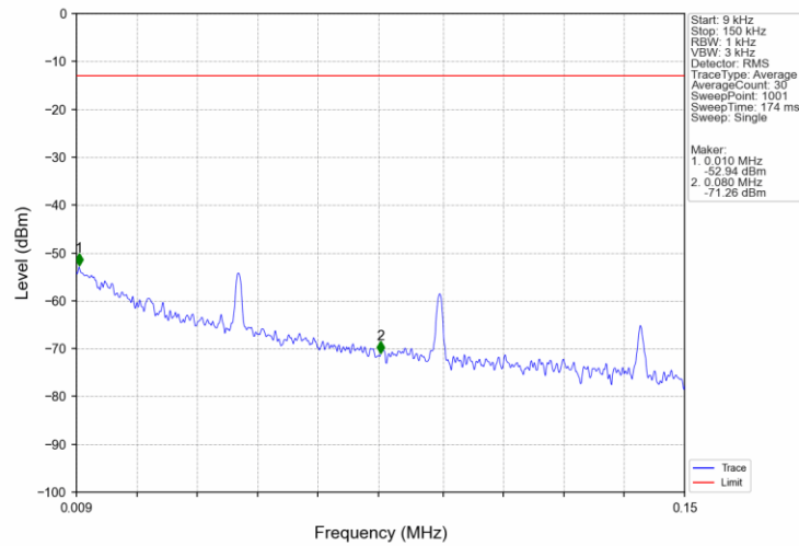
Band2 1.4MHz 16QAM LCH 1850.7MHz RB 1 0 NTN
