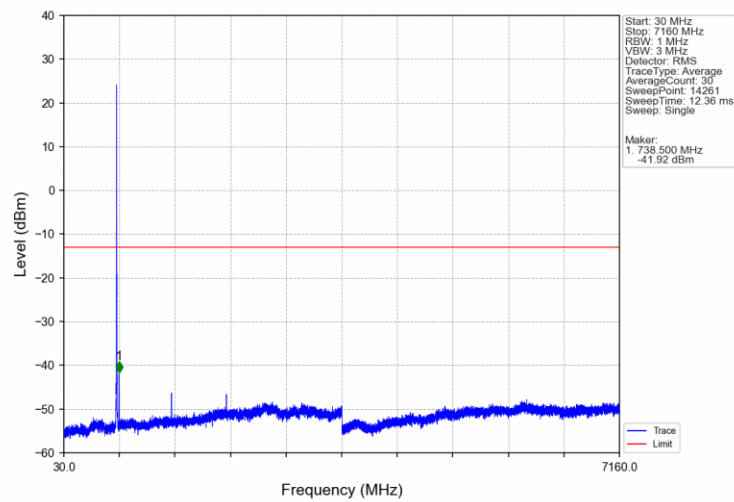
Band12_5MHz_QPSK_MCH_707.5MHz_RB_1_0_NTNV
