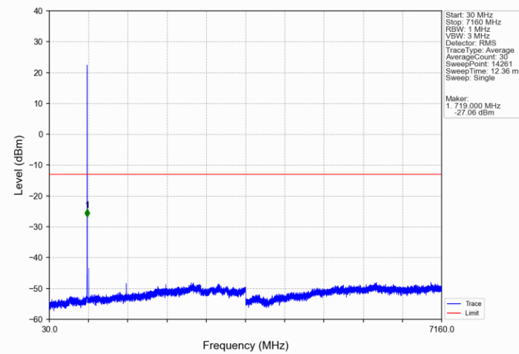
Band12_1.4MHz_16QAM_HCH_715.3MHz_RB_1_0_NTNV
