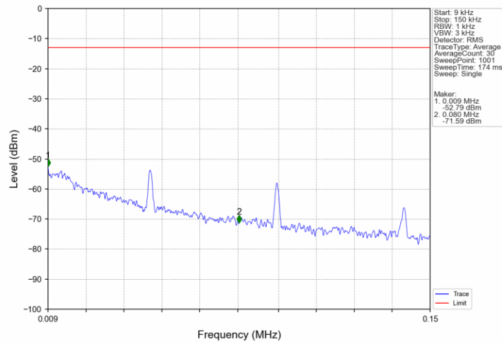
Band2_5MHz_16QAM_MCH_1880MHz_RB_1_0_NTNV
