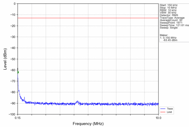
Band2_5MHz_16QAM_MCH_1880MHz_RB_1_0_NTNV
