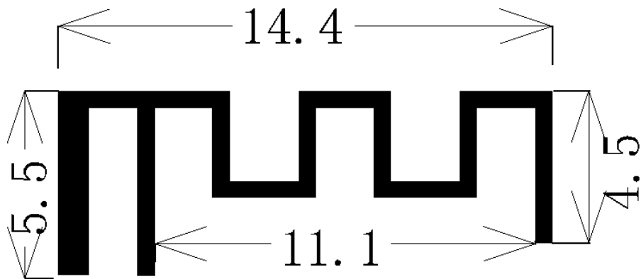
Antenna Photo & Length (mm)
