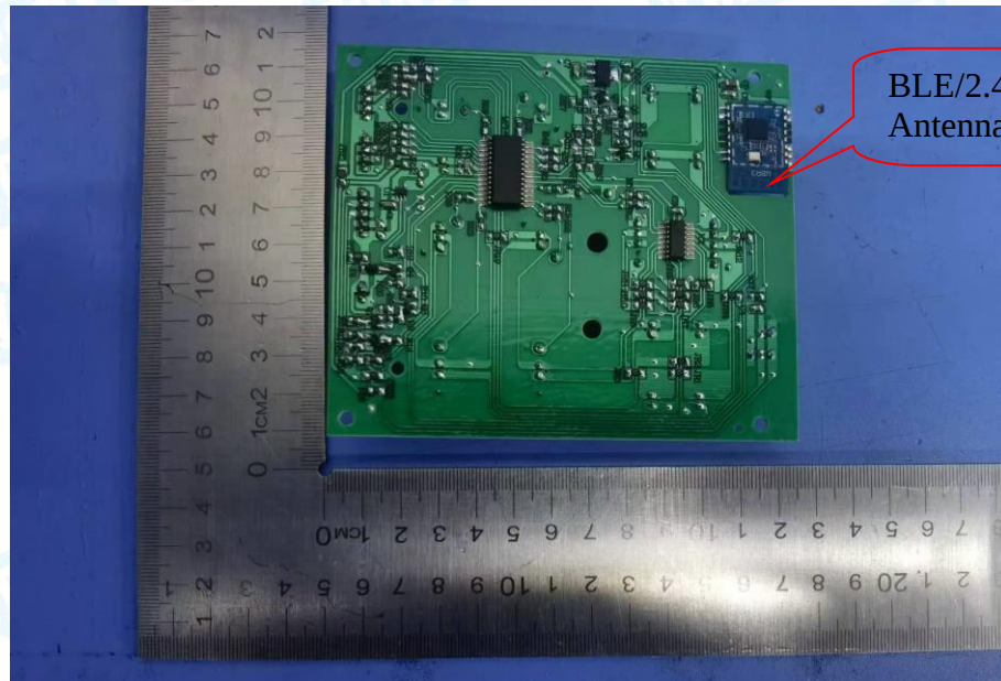
Photo 22 Appearance of PCB
