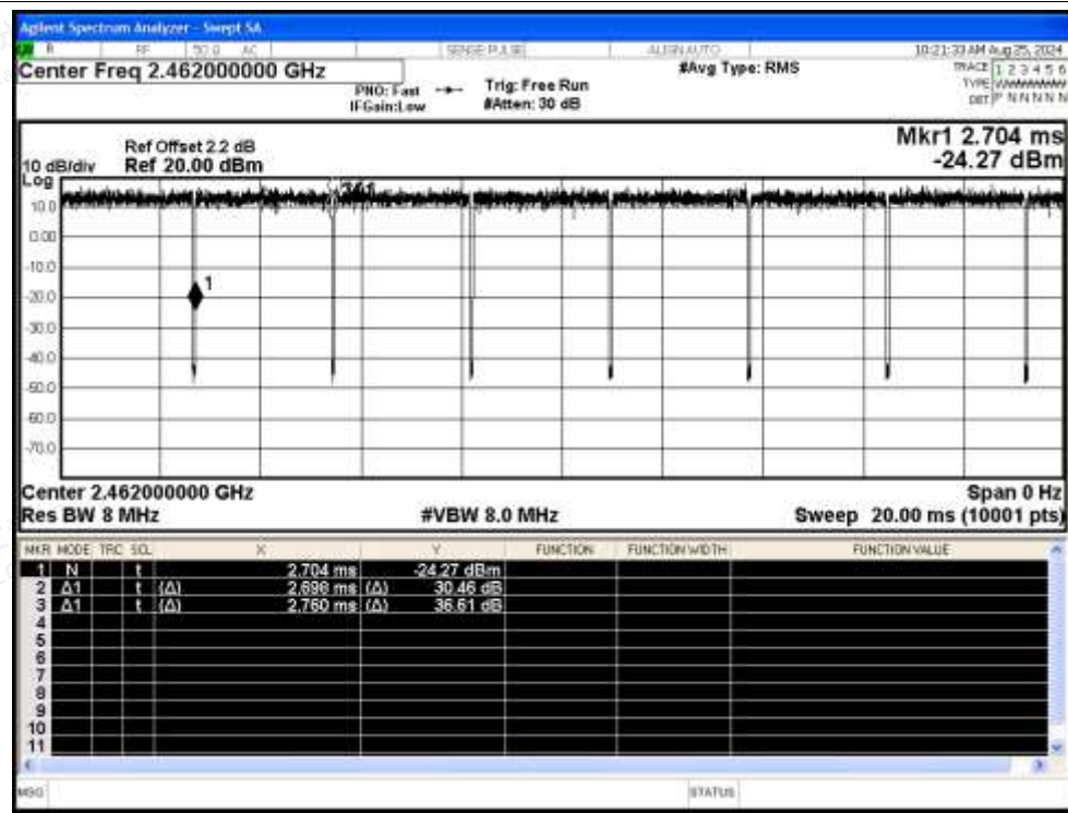
Duty Cycle NVNT g 2462MHz Ant
