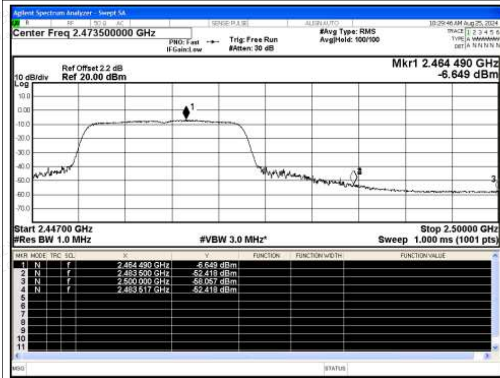
Restrict Band NVNT n20 2462MHz Ant Average
