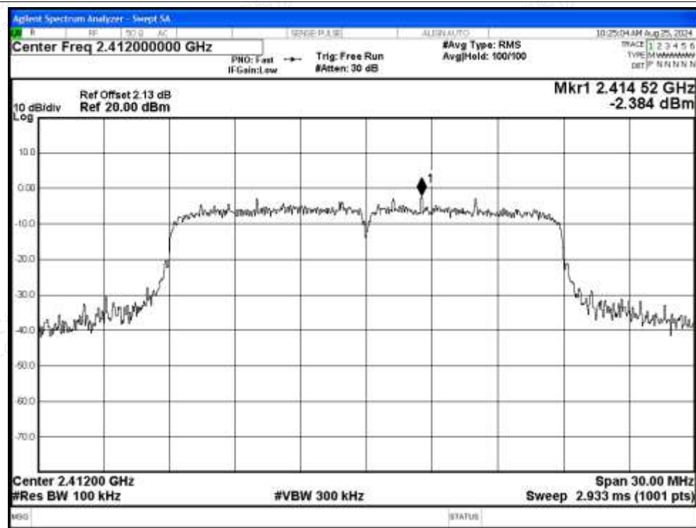
Band Edge NVNT n20 2412MHz Ant Emission
