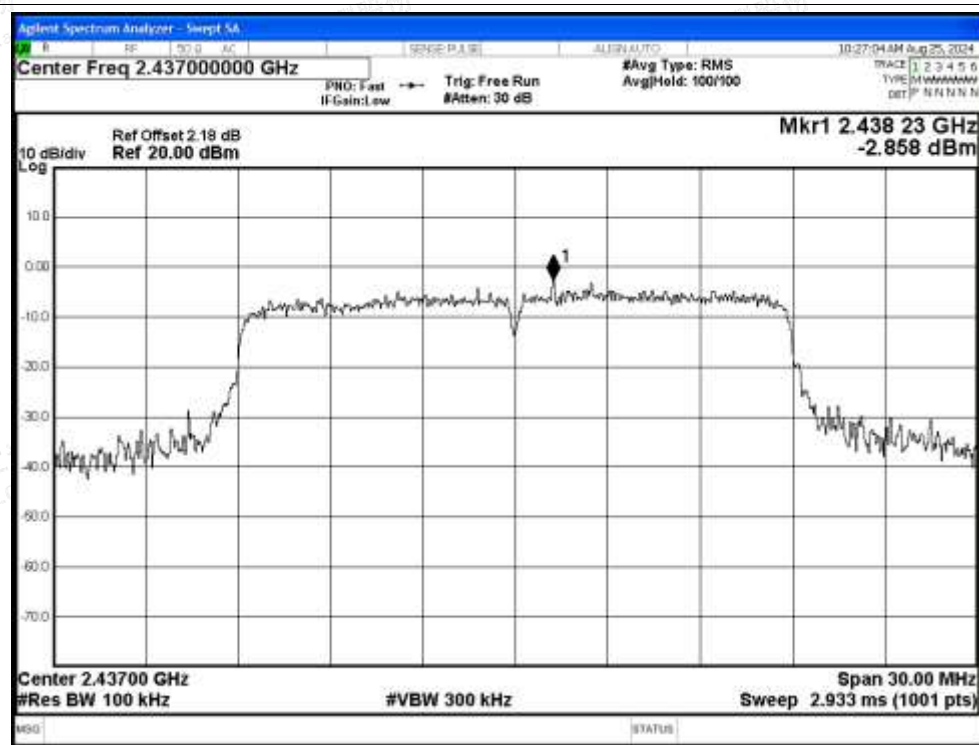
Tx. Spurious NVNT n20 2437MHz Ant Emission
