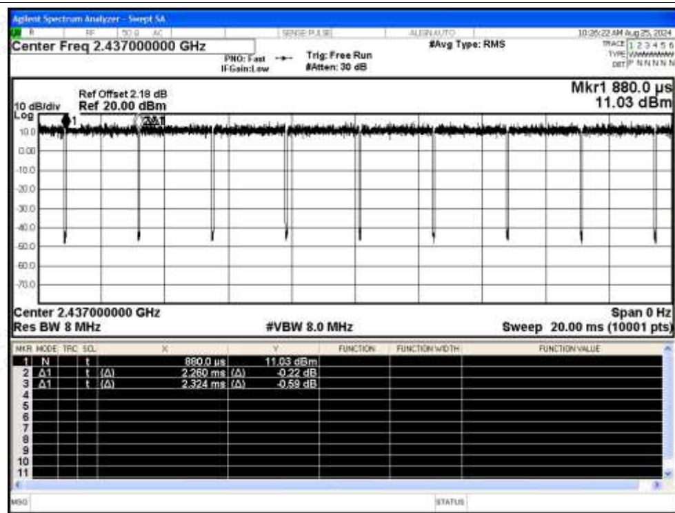
Duty Cycle NVNT n20 2437MHz Ant
