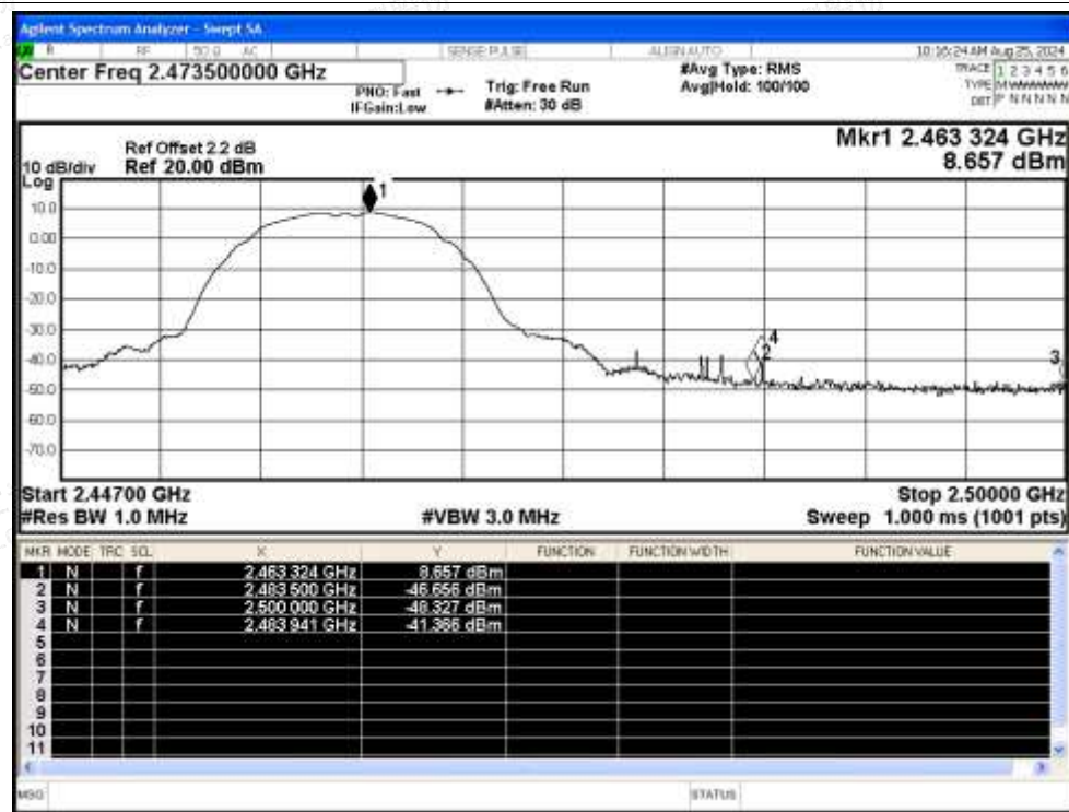
Restrict Band NVNT b 2462MHz Ant Average
