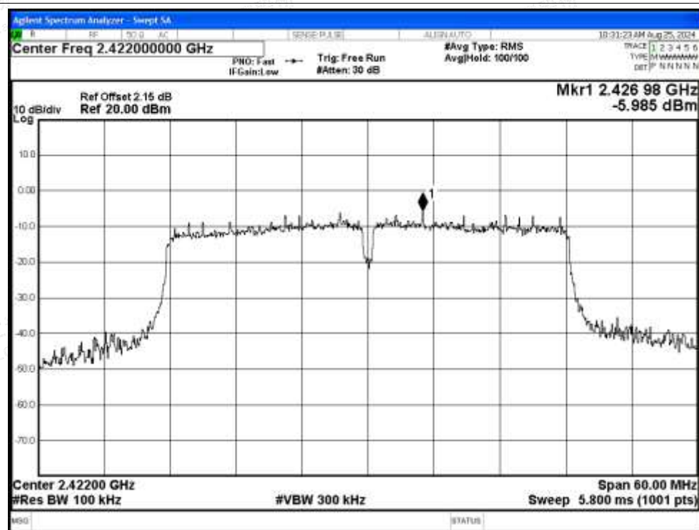
Tx. Spurious NVNT n40 2422MHz Ant Emission
