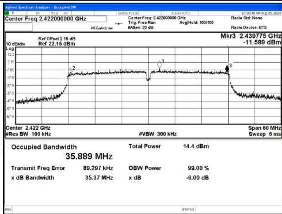
-6dB Bandwidth NVNT n40 2422MHz Ant
