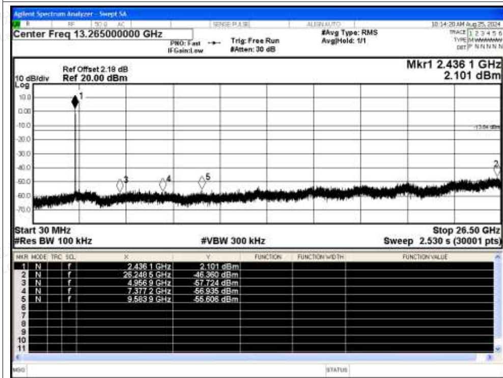
Tx. Spurious NVNT b 2437MHz Ant Emission
