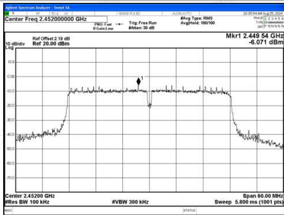
Tx. Spurious NVNT n40 2452MHz Ant Emission
