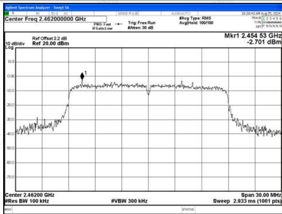
Tx. Spurious NVNT n20 2462MHz Ant Emission
