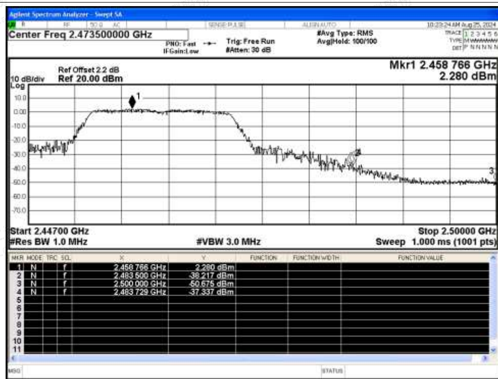
Restrict Band NVNT g 2462MHz Ant Average
