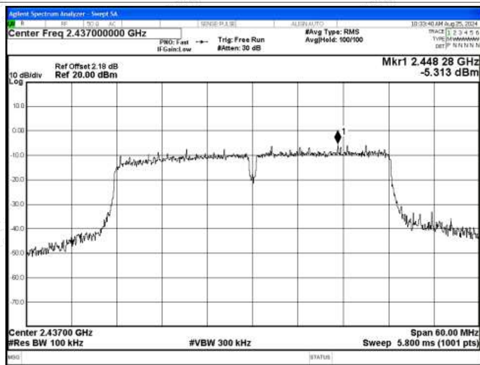
Tx. Spurious NVNT n40 2437MHz Ant Emission
