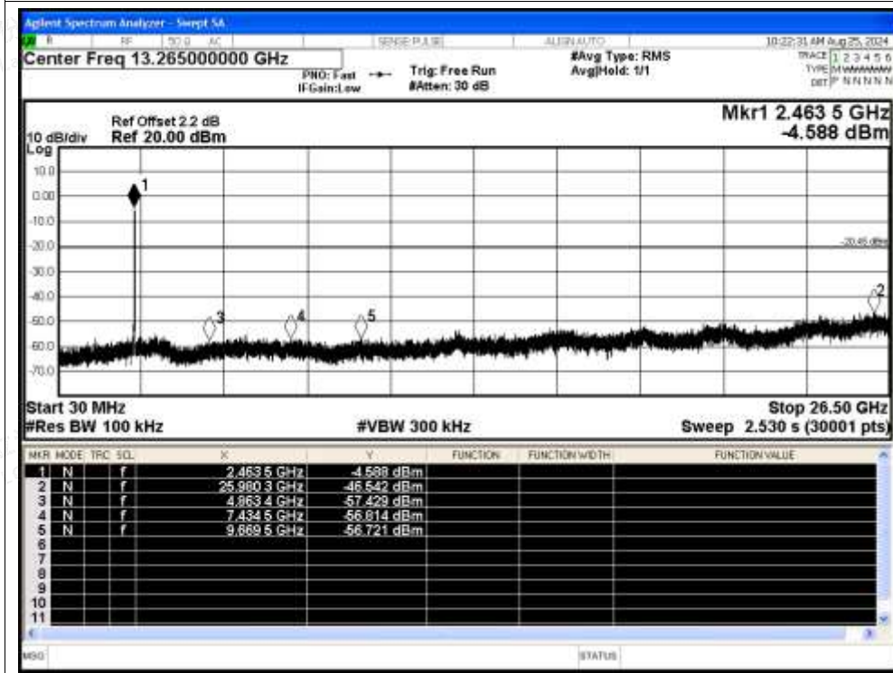
Tx. Spurious NVNT g 2462MHz Ant Emission
