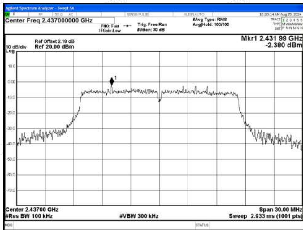
Tx. Spurious NVNT g 2437MHz Ant Emission
