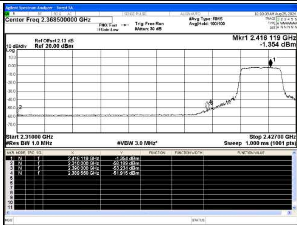
Restrict Band NVNT g 2412MHz Ant Average
