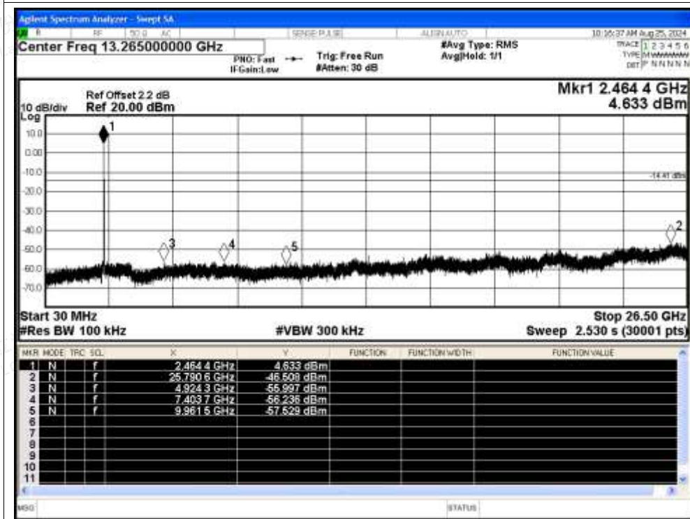
Tx. Spurious NVNT b 2462MHz Ant Emission
