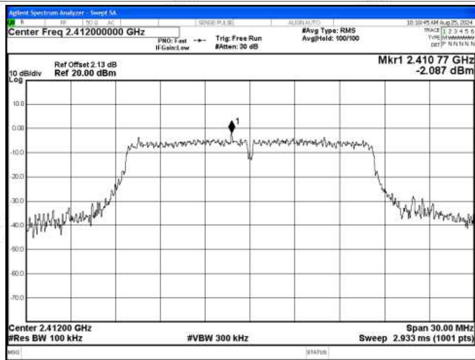
Tx. Spurious NVNT g 2412MHz Ant Emission
