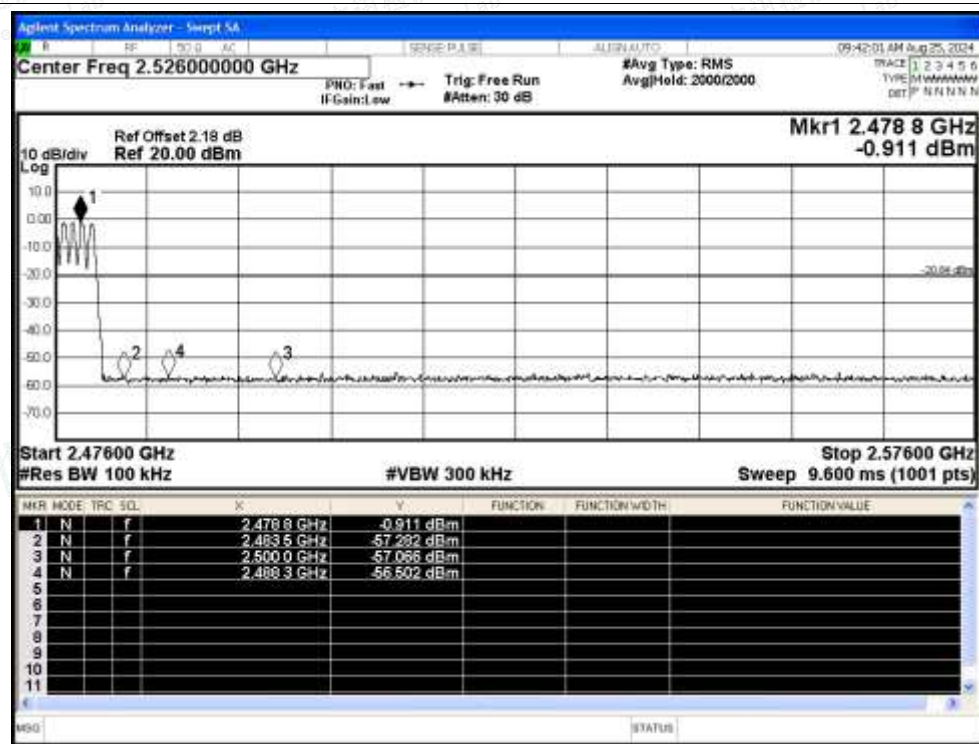
Band Edge(Hopping) NVNT 1-DH5 2480MHz Ant Hopping Emission
