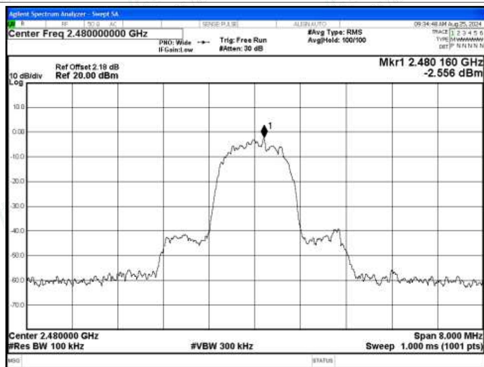
Band Edge NVNT 3-DH5 2480MHz Ant No-Hopping Emission
