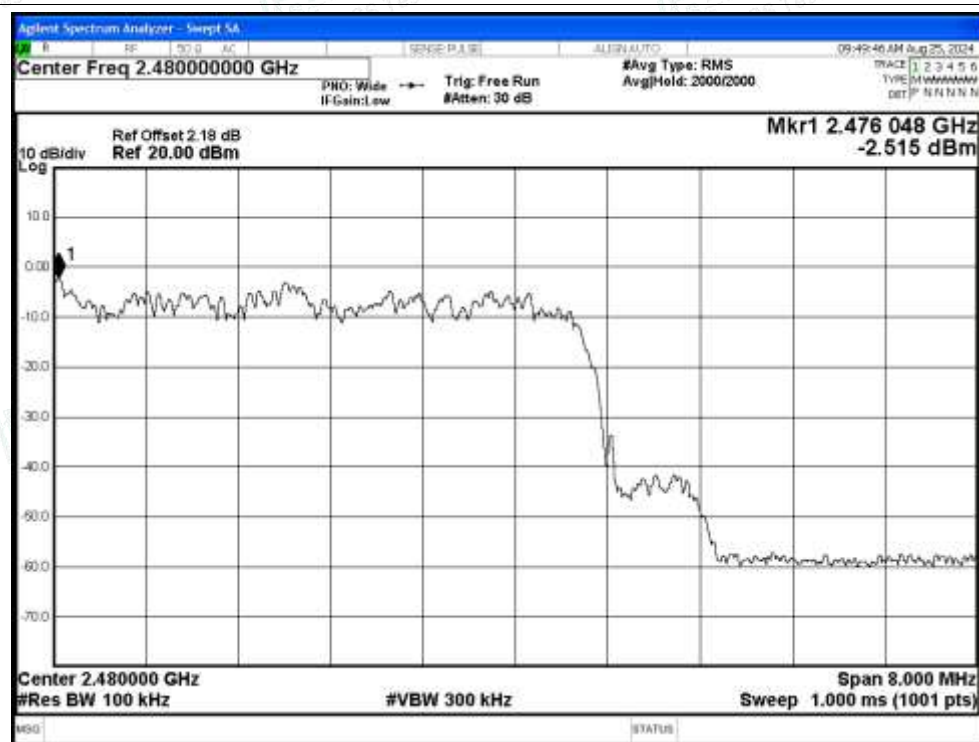
Band Edge(Hopping) NVNT 3-DH5 2480MHz Ant Hopping Emission
