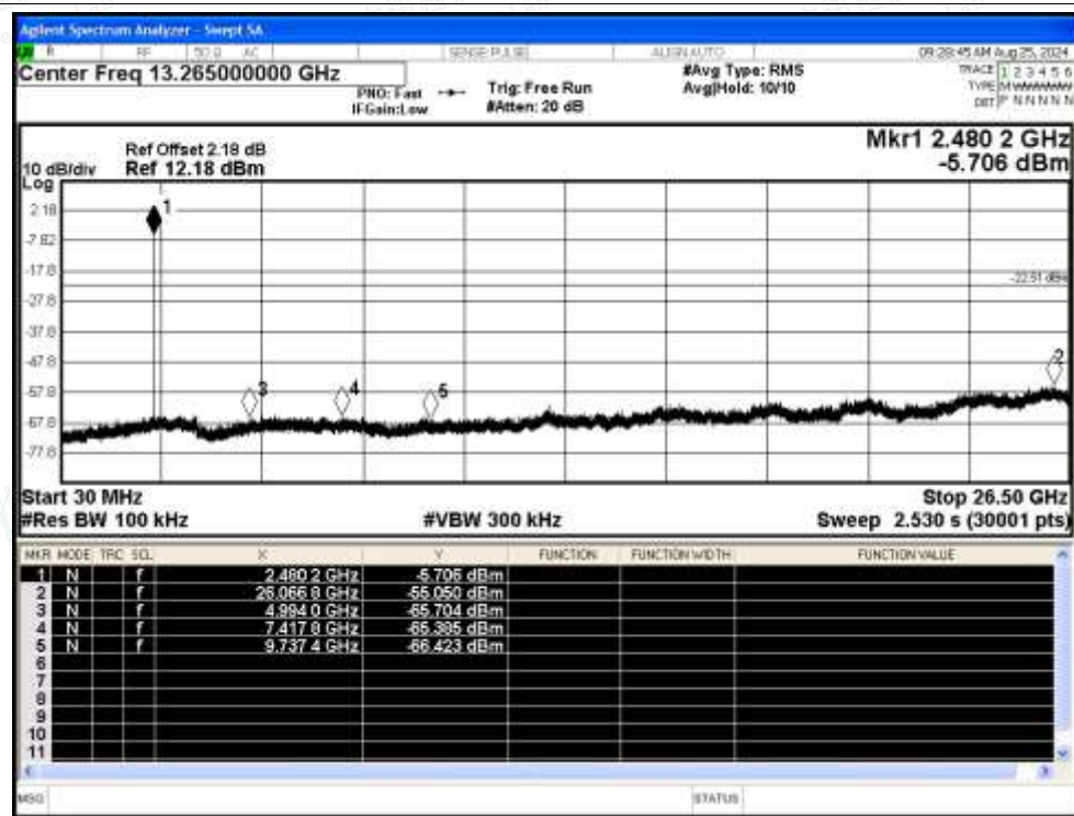
Tx. Spurious NVNT 2-DH5 2480MHz Ant Emission
