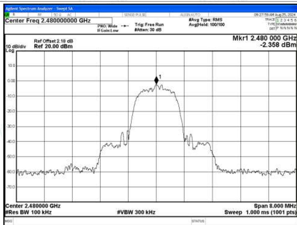
Band Edge NVNT 2-DH5 2480MHz Ant No-Hopping Emission
