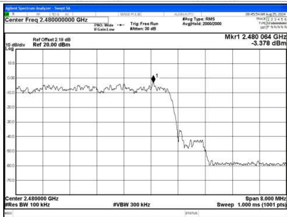
Band Edge(Hopping) NVNT 2-DH5 2480MHz Ant Hopping Emission
