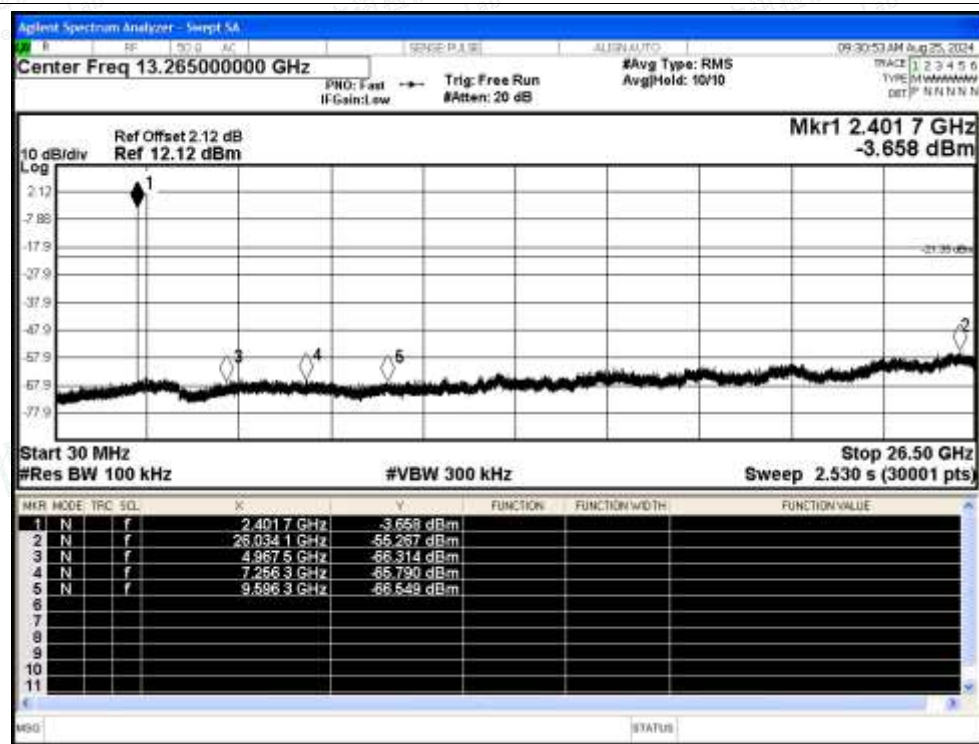
Tx. Spurious NVNT 3-DH5 2402MHz Ant Emission
