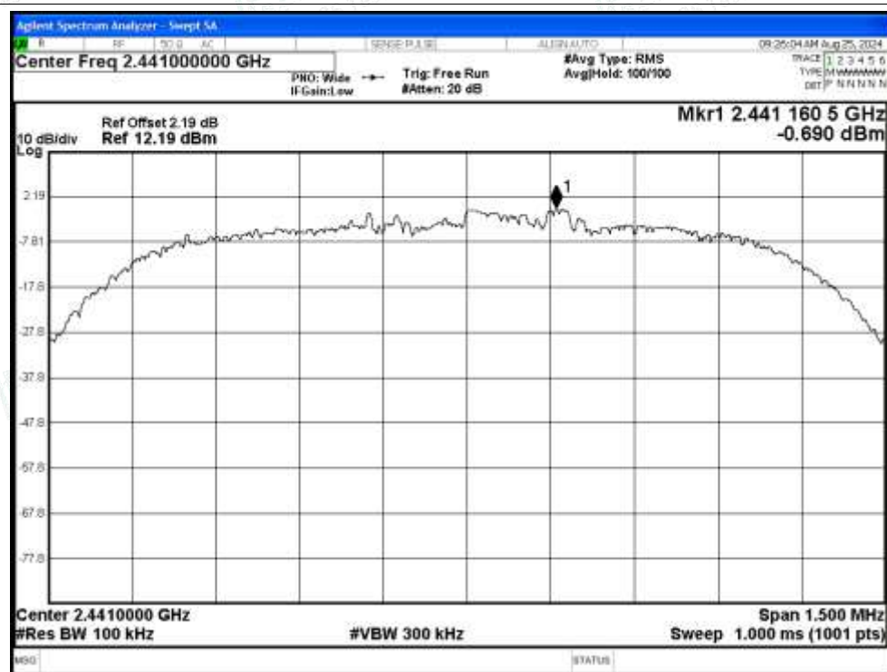
Tx. Spurious NVNT 2-DH5 2441MHz Ant Emission
