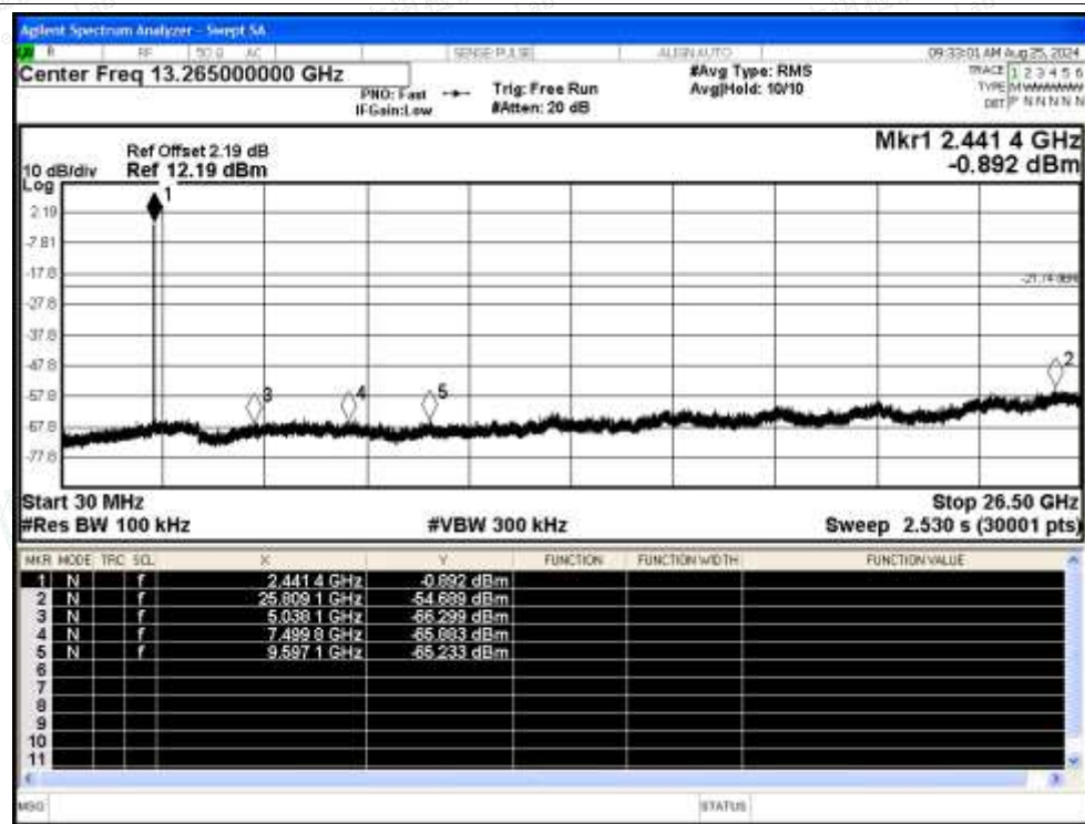
Tx. Spurious NVNT 3-DH5 2441MHz Ant Emission
