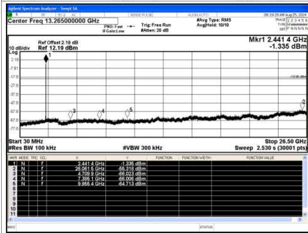
Tx. Spurious NVNT 1-DH5 2441MHz Ant Emission
