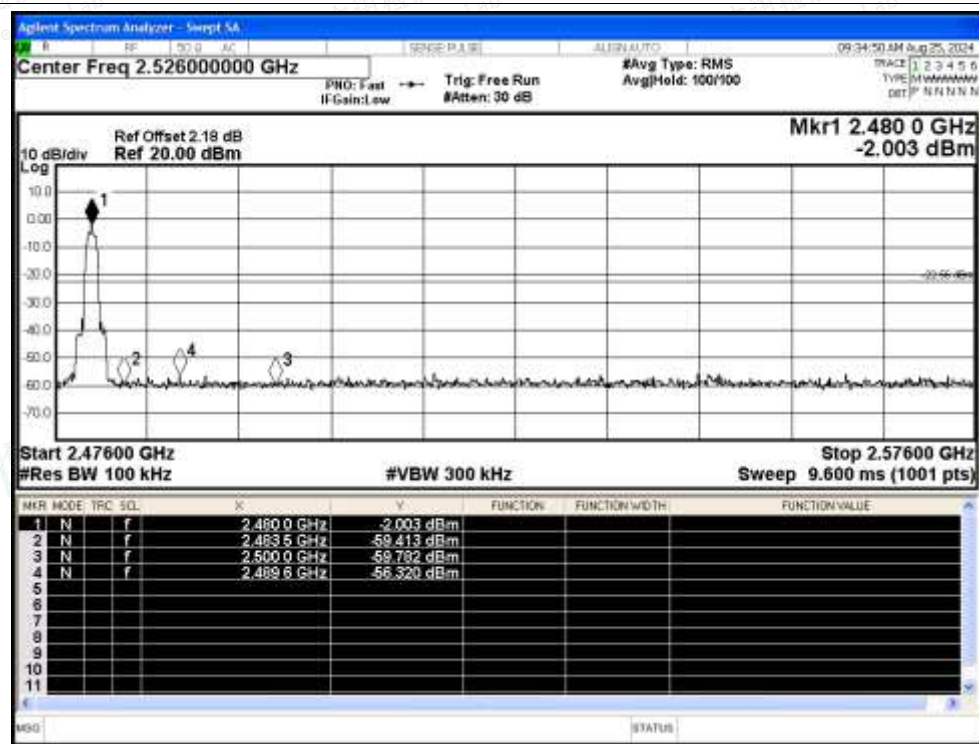
Band Edge NVNT 3-DH5 2480MHz Ant No-Hopping Emission
