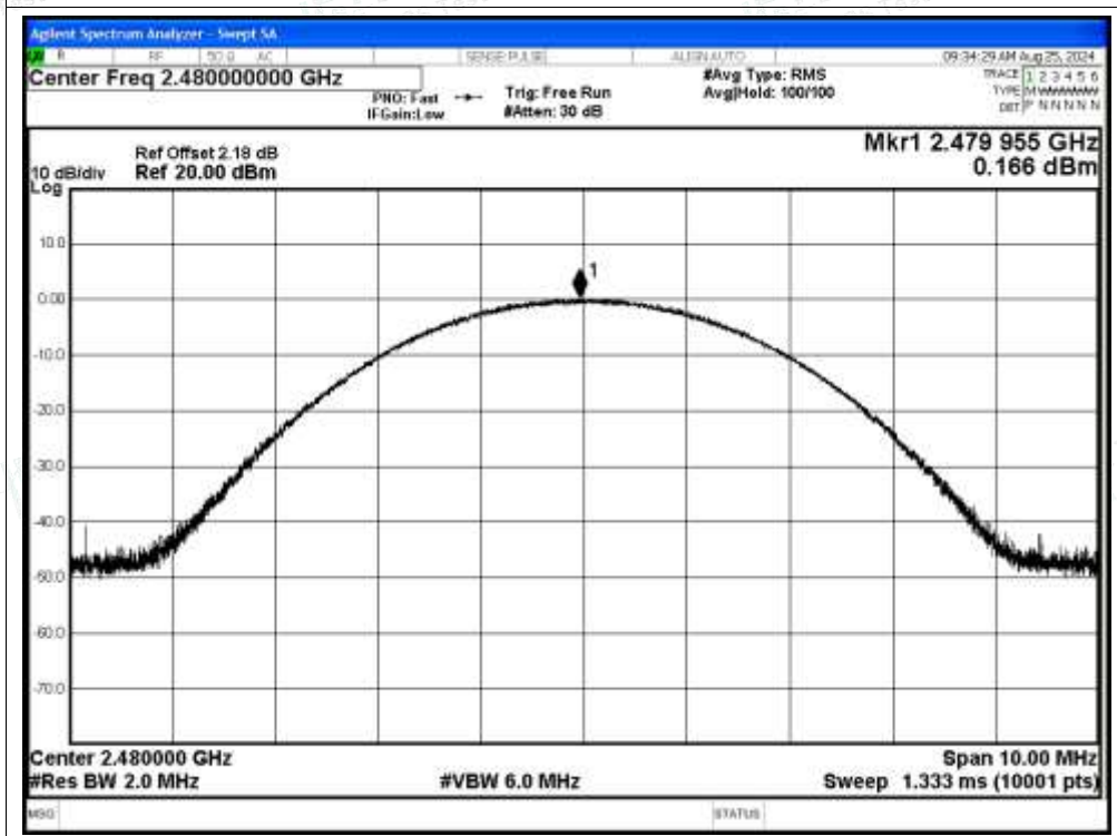
Power NVNT 3-DH5 2480MHz Ant
