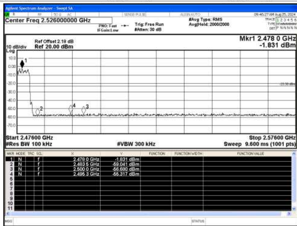
Band Edge(Hopping) NVNT 2-DH5 2480MHz Ant Hopping Emission
