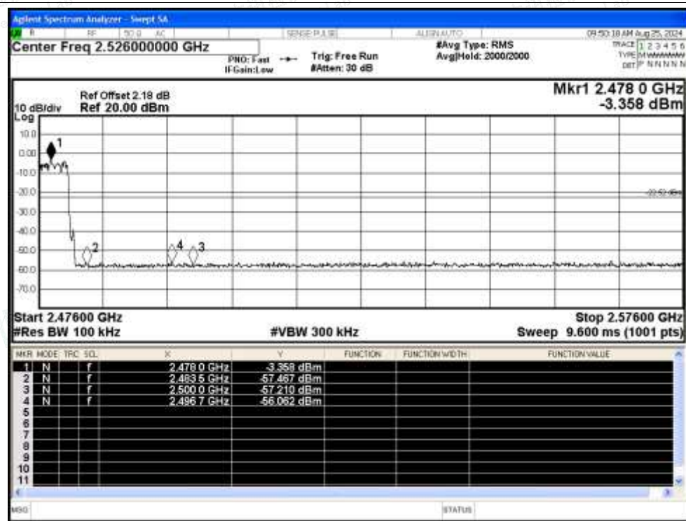
Band Edge(Hopping) NVNT 3-DH5 2480MHz Ant Hopping Emission
