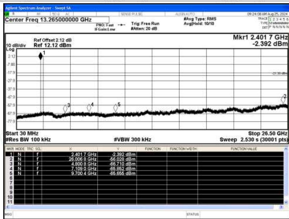
Tx. Spurious NVNT 2-DH5 2402MHz Ant Emission
