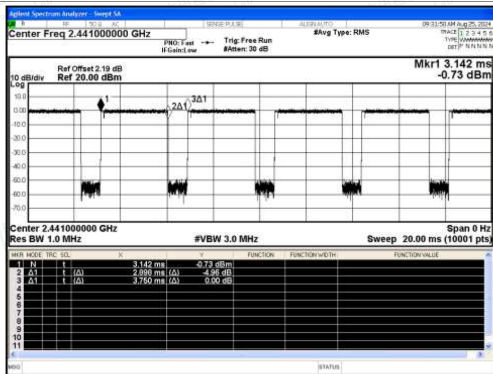
Duty Cycle NVNT 3-DH5 2441MHz Ant
