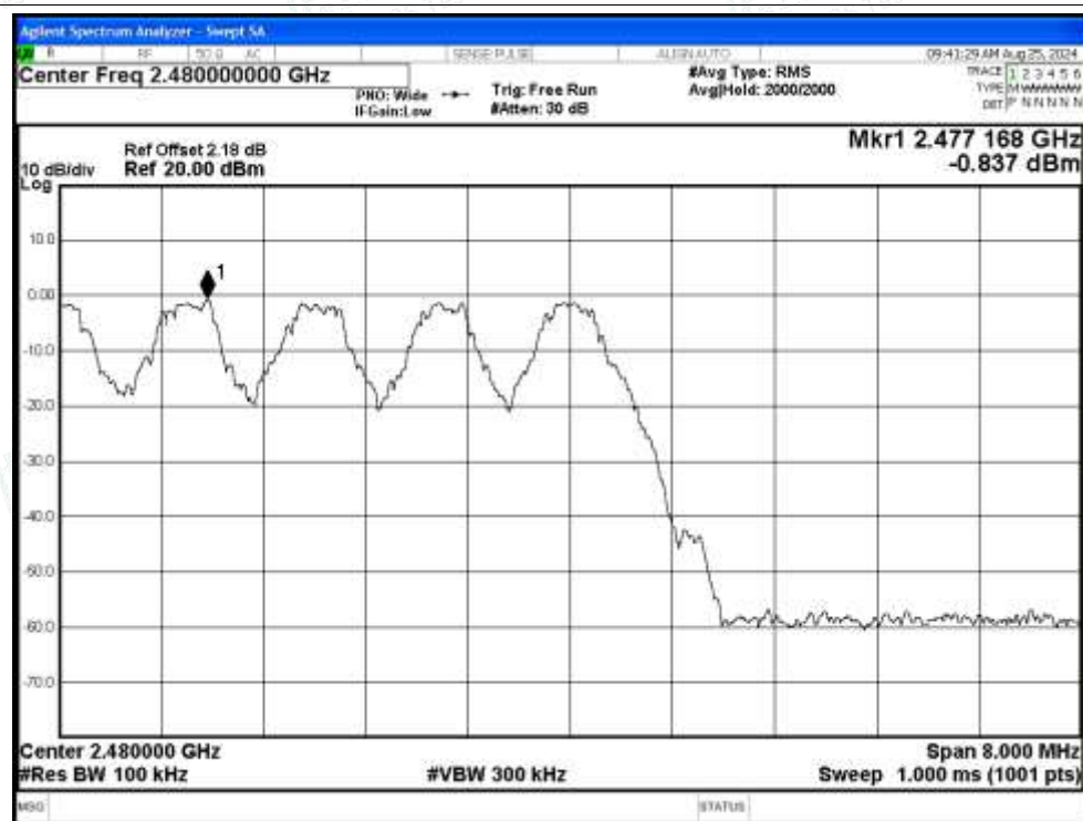
Band Edge(Hopping) NVNT 1-DH5 2480MHz Ant Hopping Emission
