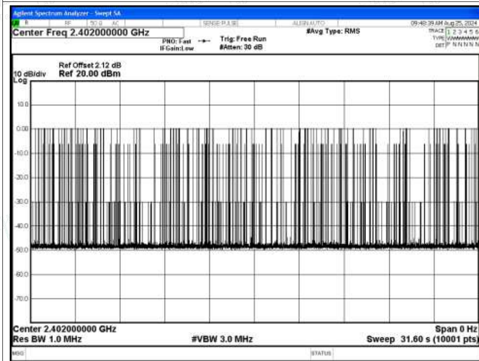
Dwell NVNT 3-DH5 2402MHz Ant Accumulated
