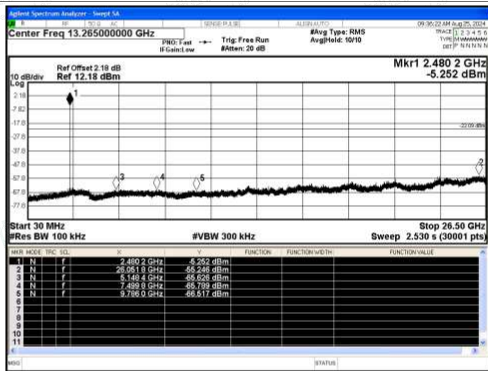
Tx. Spurious NVNT 3-DH5 2480MHz Ant Emission
