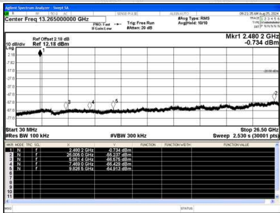
Tx. Spurious NVNT 1-DH5 2480MHz Ant Emission
