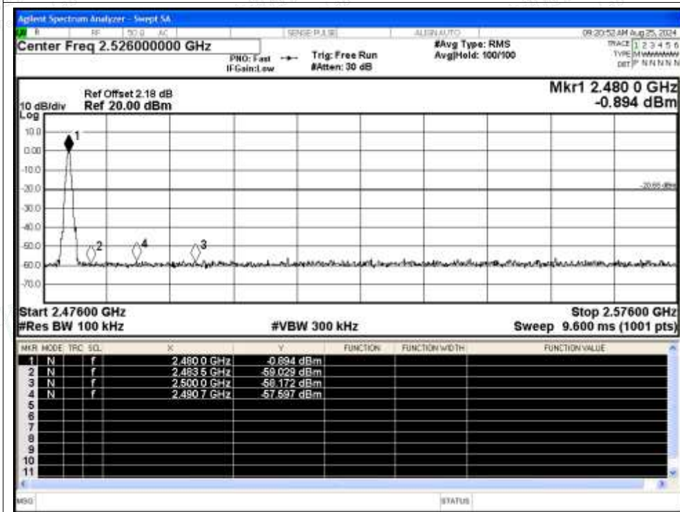
Band Edge NVNT 1-DH5 2480MHz Ant No-Hopping Emission
