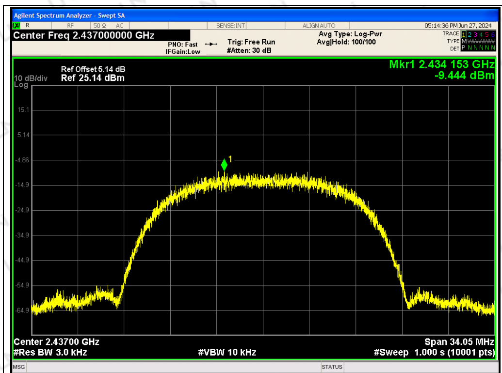
CH06: 2437MHz
