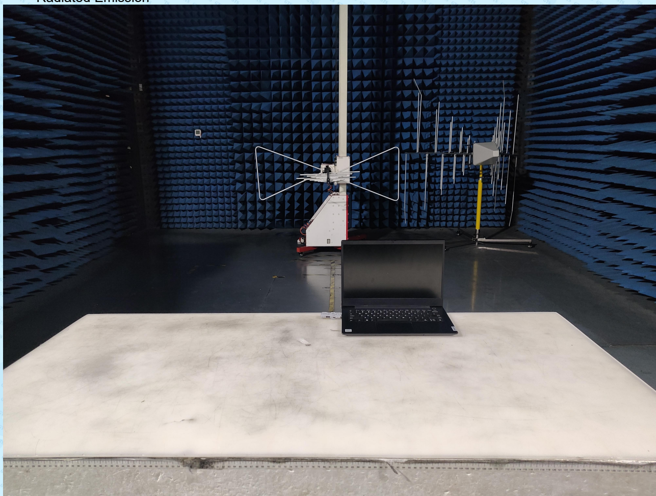
Radiated Emission
