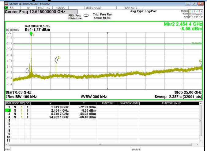
802.11g High CH, 2462MHz 30MHz-25GHz
