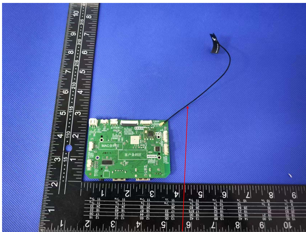
Internal antenna
