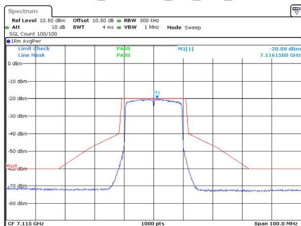
802.11ax20_7115MHz_RU_Full_Chain 1
