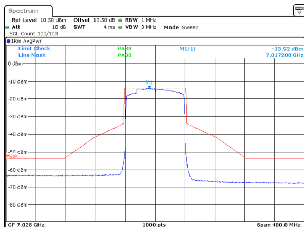
802.11ax80_7025MHz_RU_Full_Chain 1
