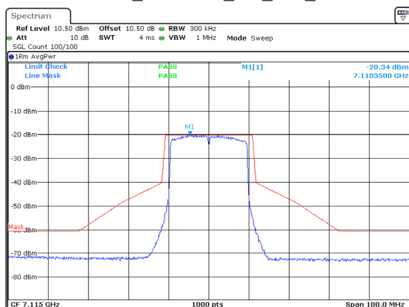
802.11ax20_7115MHz_RU_Full_Chain 0
