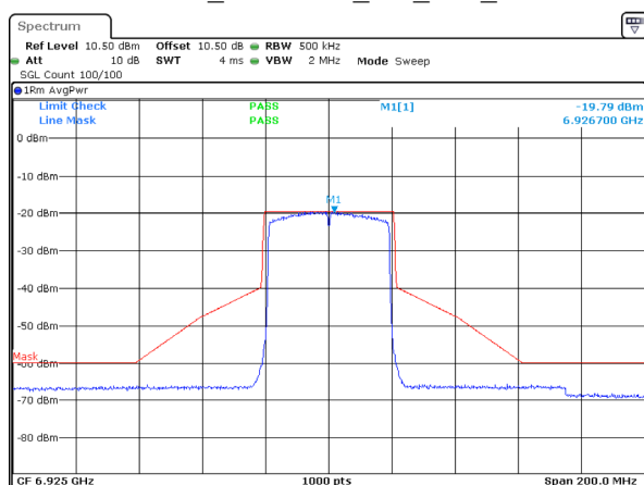
802.11ax40_6925MHz_RU_Full_Chain 3
