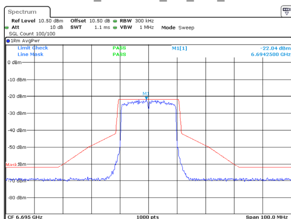
802.11ax20_6695MHz_RU_Full_Chain 3
