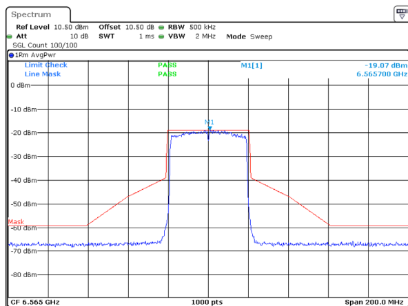
802.11ax40_6565MHz_RU_Full_Chain 3
