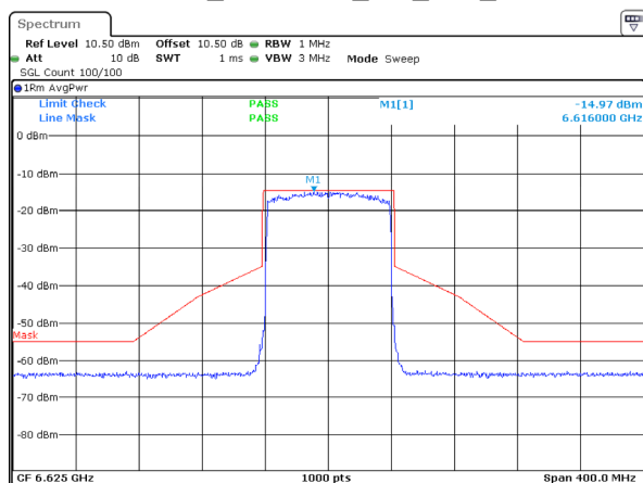
802.11ax80_6625MHz_RU_Full_Chain 3
