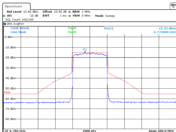
802.11ax80_6785MHz_RU_Full_Chain 0
