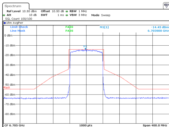
802.11ax80_6705MHz_RU_Full_Chain 3
