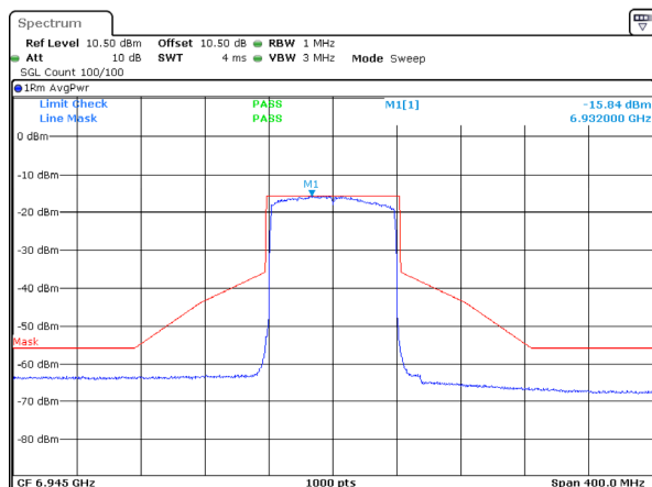
802.11ax80_6945MHz_RU_Full_Chain 0
