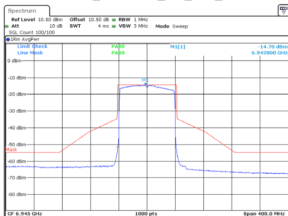
802.11ax80_6945MHz_RU_Full_Chain 2
