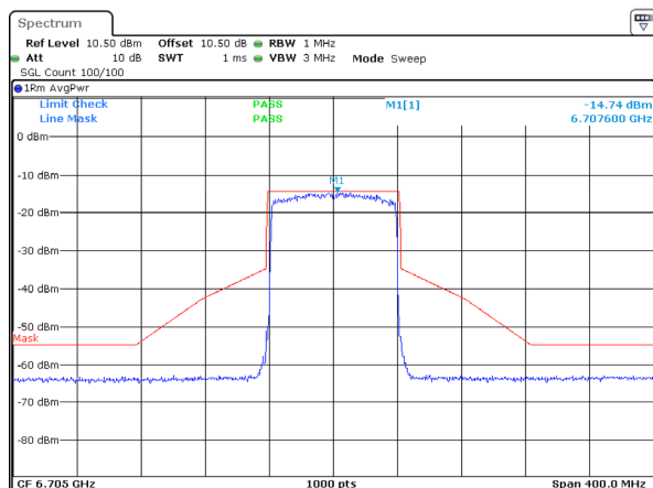
802.11ax80_6705MHz_RU_Full_Chain 0
