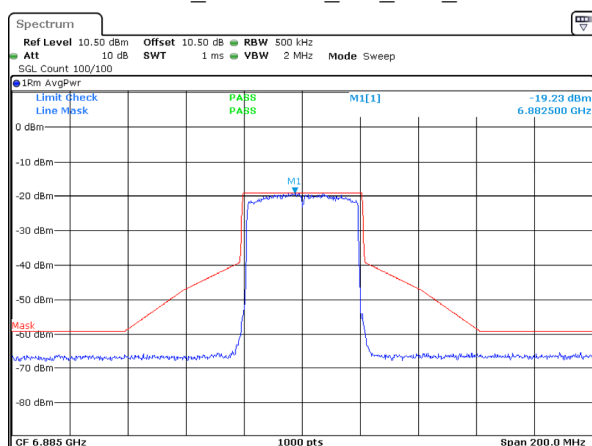
802.11ax40_6885MHz_RU_Full_Chain 3
