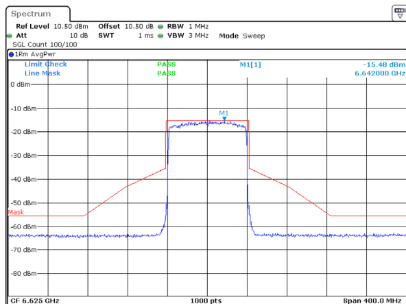
802.11ax80_6625MHz_RU_Full_Chain 0
