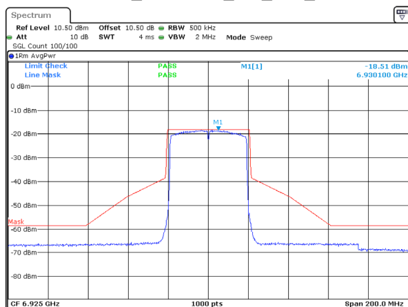
802.11ax40_6925MHz_RU_Full_Chain 2
