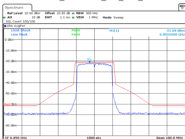
802.11ax20_6895MHz_RU_Full_Chain 1
