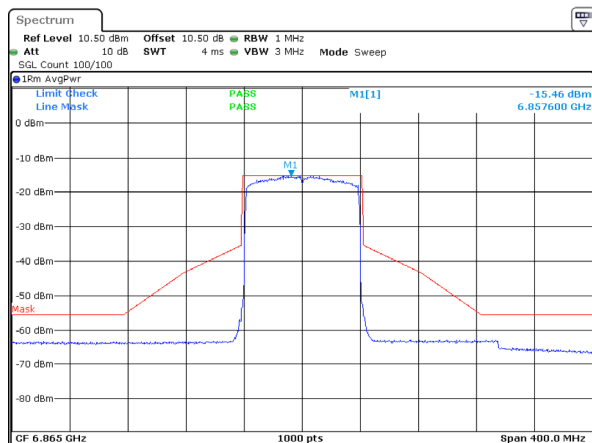
802.11ax80_6865MHz_RU_Full_Chain 0
