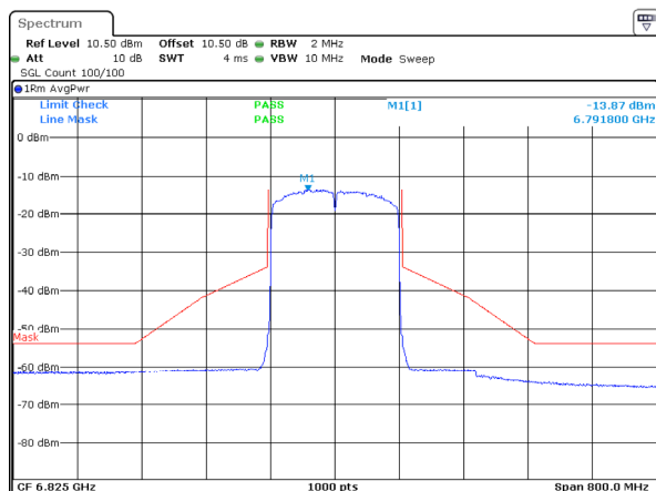
802.11ax160_6825MHz_RU_Full_Chain 2
