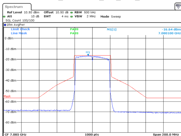
802.11ax40_7085MHz_RU_Full_Chain 0
