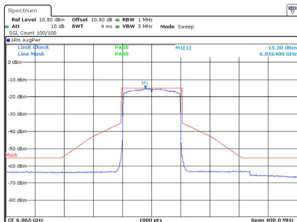
802.11ax80_6865MHz_RU_Full_Chain 1
