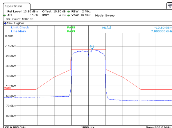
802.11ax160_6985MHz_RU_Full_Chain 1
