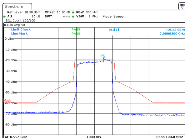
802.11ax20_6995MHz_RU_Full_Chain 2
