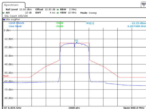
802.11ax160_6825MHz_RU_Full_Chain 1
