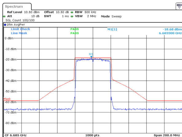
802.11ax40_6685MHz_RU_Full_Chain 3
