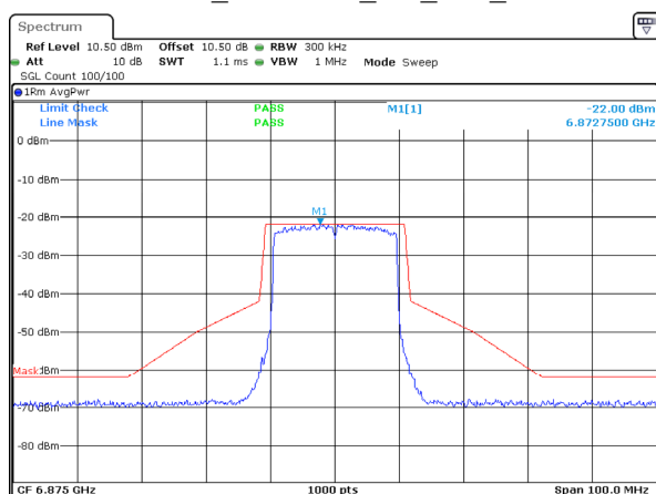
802.11ax20_6875MHz_RU_Full_Chain 1
