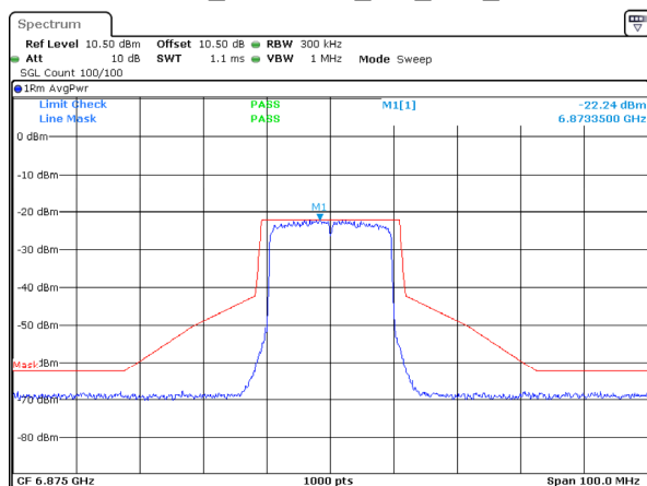
802.11ax20_6875MHz_RU_Full_Chain 3
