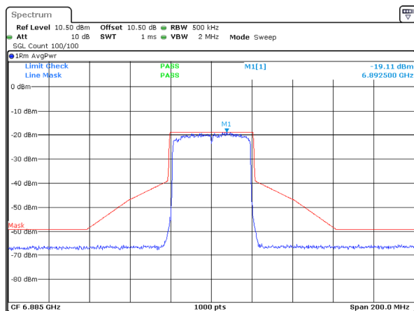
802.11ax40_6885MHz_RU_Full_Chain 1
