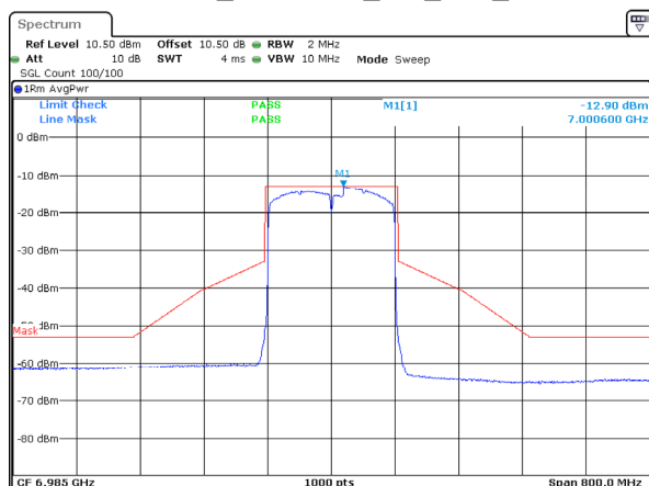
802.11ax160_6985MHz_RU_Full_Chain 2
