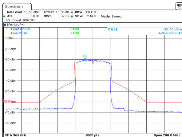
802.11ax40_6965MHz_RU_Full_Chain 1
