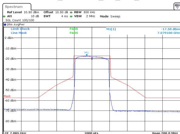
802.11ax40_7085MHz_RU_Full_Chain 3
