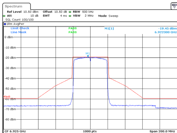
802.11ax40_6925MHz_RU_Full_Chain 0
