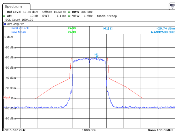
802.11ax20_6695MHz_RU_Full_Chain 2
