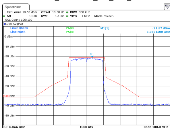
802.11ax20_6855MHz_RU_Full_Chain 3
