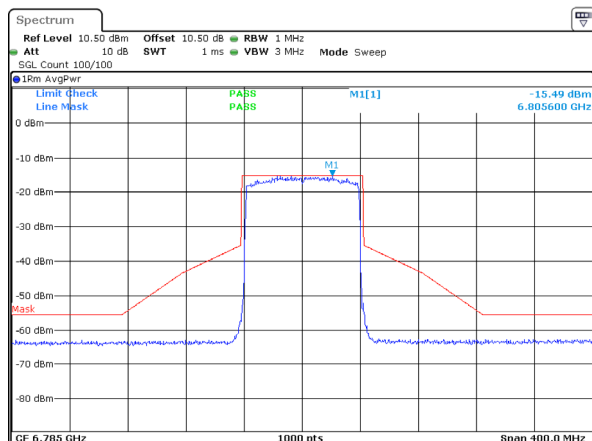
802.11ax80_6785MHz_RU_Full_Chain 1
