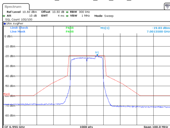
802.11ax20_6995MHz_RU_Full_Chain 0
