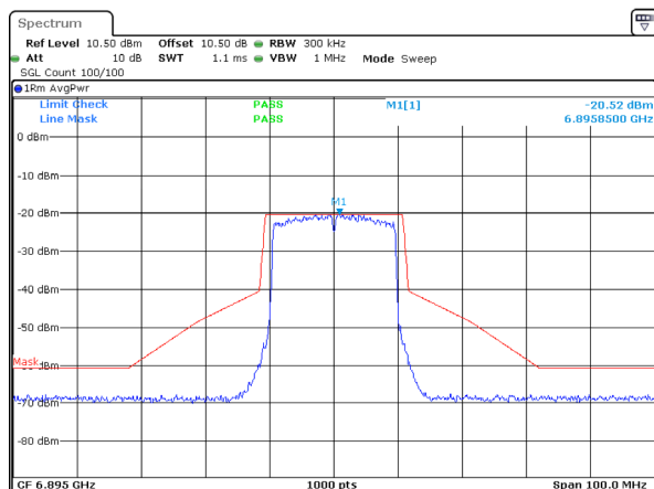
802.11ax20_6895MHz_RU_Full_Chain 2
