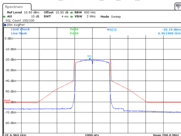
802.11ax40_6965MHz_RU_Full_Chain 3
