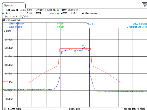
802.11ax20_6995MHz_RU_Full_Chain 1
