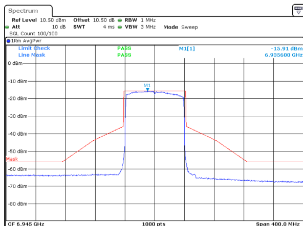
802.11ax80_6945MHz_RU_Full_Chain 1
