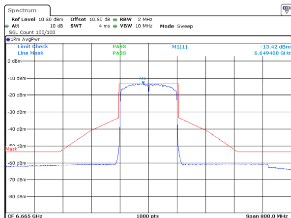
802.11ax160_6665MHz_RU_Full_Chain 2
