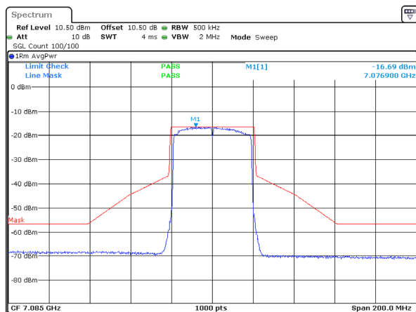
802.11ax40_7085MHz_RU_Full_Chain 1
