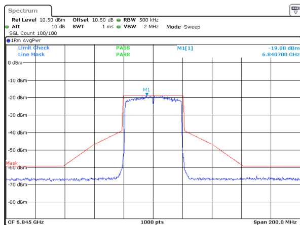
802.11ax40_6845MHz_RU_Full_Chain 3
