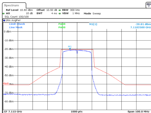
802.11ax20_7115MHz_RU_Full_Chain 3
