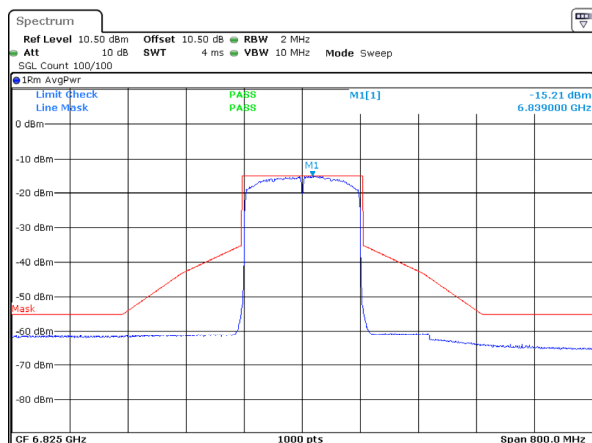
802.11ax160_6825MHz_RU_Full_Chain 3
