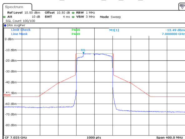
802.11ax80_7025MHz_RU_Full_Chain 2
