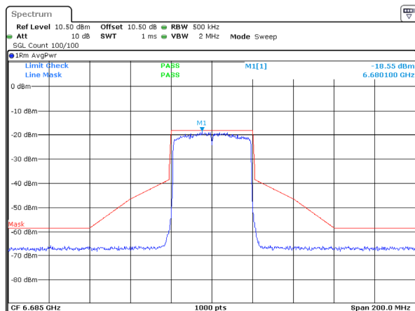
802.11ax40_6685MHz_RU_Full_Chain 0
