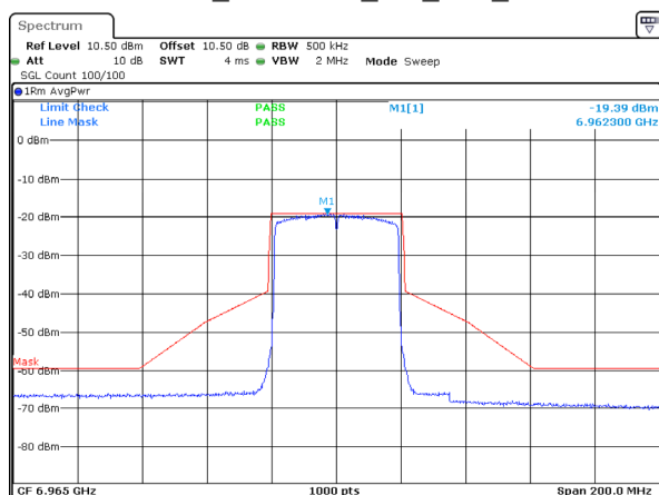
802.11ax40_6965MHz_RU_Full_Chain 2
