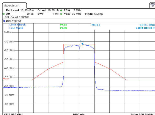
802.11ax160_6985MHz_RU_Full_Chain 0
