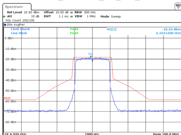
802.11ax20_6535MHz_RU_Full_Chain 2
