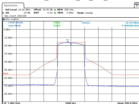
802.11ax40_7085MHz_RU_Full_Chain 2
