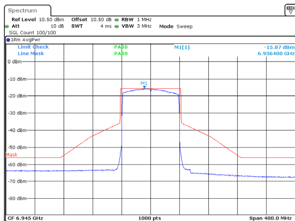
802.11ax80_6945MHz_RU_Full_Chain 3
