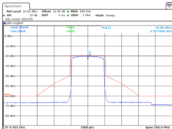
802.11ax40_6925MHz_RU_Full_Chain 1
