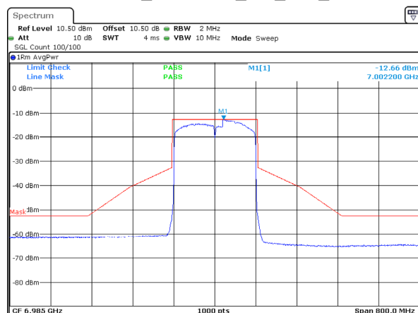
802.11ax160_6985MHz_RU_Full_Chain 3
