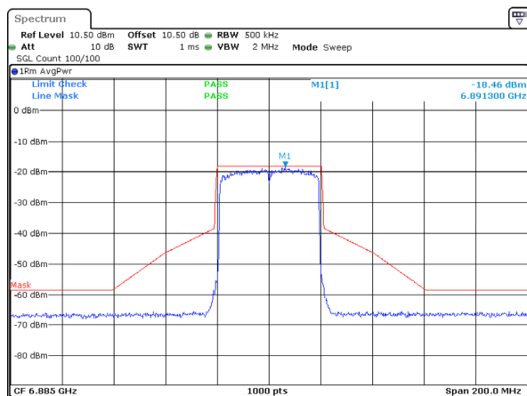
802.11ax40_6885MHz_RU_Full_Chain 0
