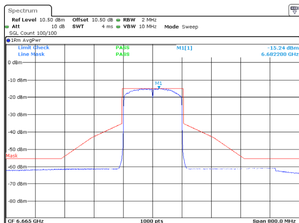
802.11ax160_6665MHz_RU_Full_Chain 3
