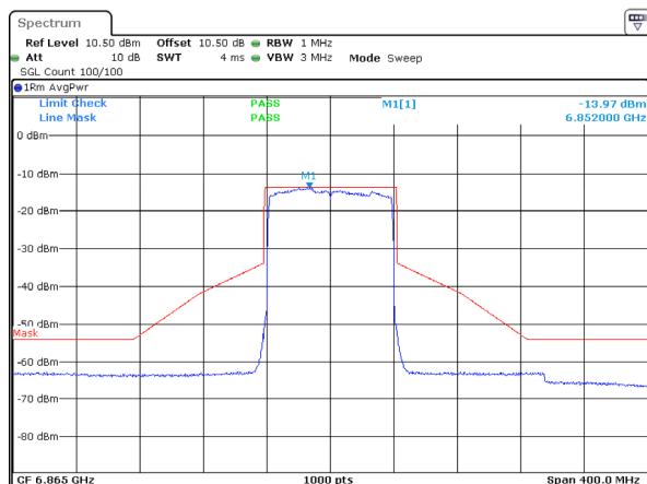
802.11ax80_6865MHz_RU_Full_Chain 2
