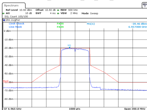
802.11ax40_6965MHz_RU_Full_Chain 0
