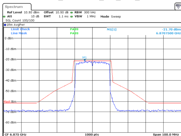
802.11ax20_6875MHz_RU_Full_Chain 0
