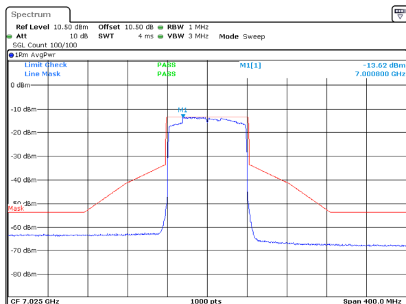
802.11ax80_7025MHz_RU_Full_Chain 0
