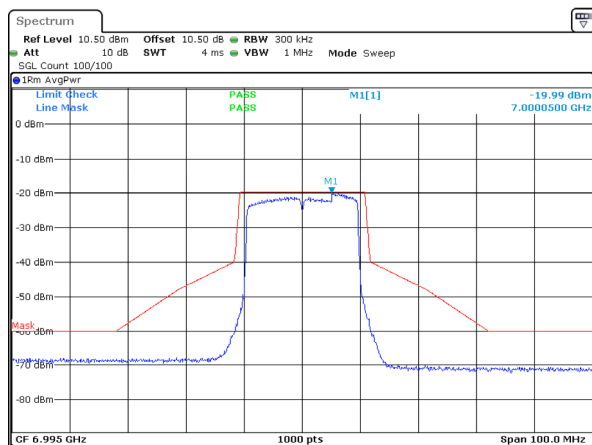
802.11ax20_6995MHz_RU_Full_Chain 3
