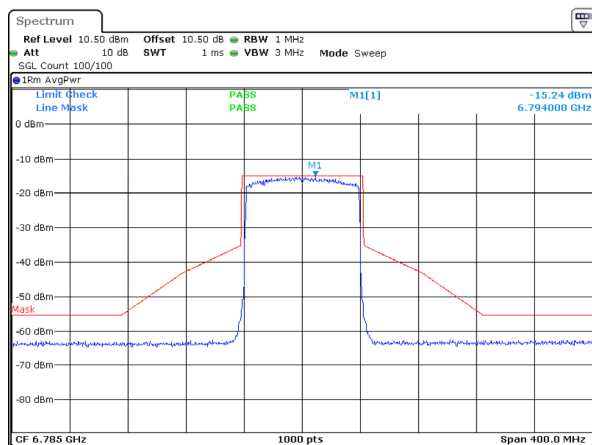
802.11ax80_6785MHz_RU_Full_Chain 3
