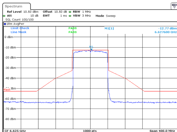
802.11ax80_6625MHz_RU_Full_Chain 2
