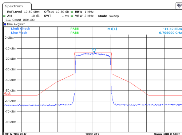
802.11ax80_6705MHz_RU_Full_Chain 1
