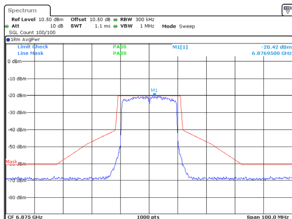
802.11ax20_6875MHz_RU_Full_Chain 2
