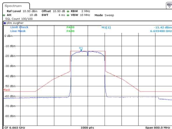
802.11ax160_6665MHz_RU_Full_Chain 1
