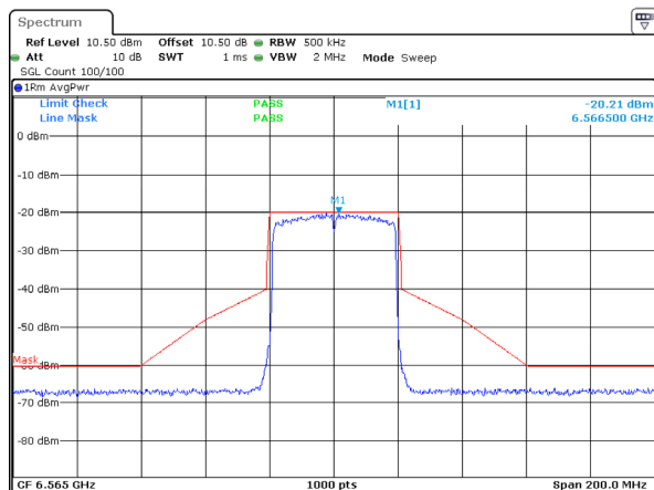
802.11ax40_6565MHz_RU_Full_Chain 0
