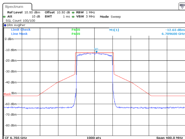
802.11ax80_6705MHz_RU_Full_Chain 2
