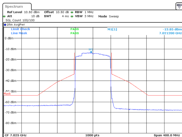
802.11ax80_7025MHz_RU_Full_Chain 3
