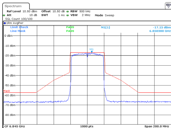
802.11ax40_6845MHz_RU_Full_Chain 2
