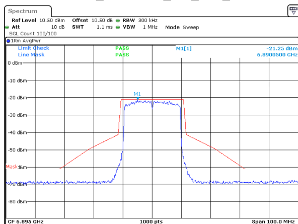
802.11ax20_6895MHz_RU_Full_Chain 3
