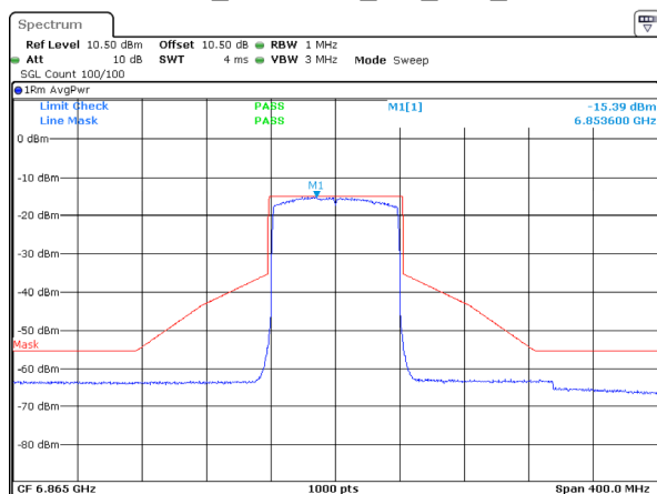
802.11ax80_6865MHz_RU_Full_Chain 3
