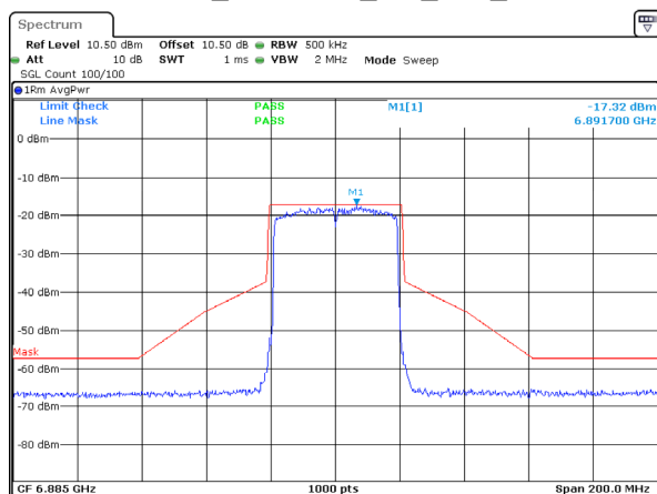
802.11ax40_6885MHz_RU_Full_Chain 2
