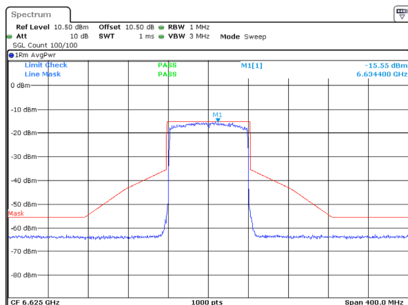
802.11ax80_6625MHz_RU_Full_Chain 1
