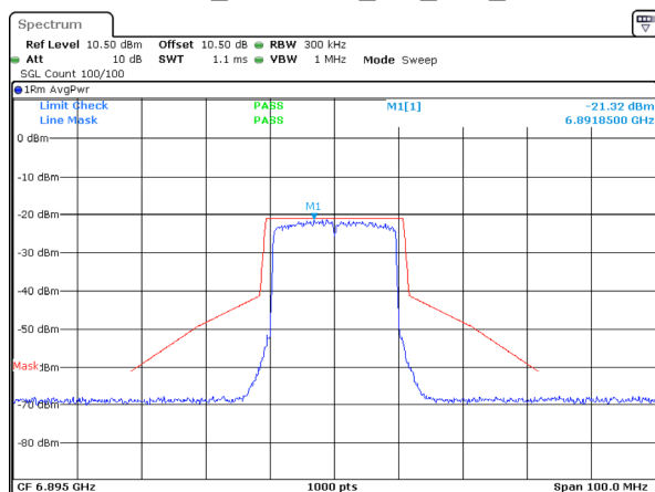
802.11ax20_6895MHz_RU_Full_Chain 0
