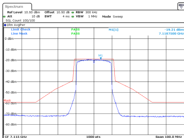
802.11ax20_7115MHz_RU_Full_Chain 2
