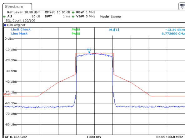
802.11ax80_6785MHz_RU_Full_Chain 2
