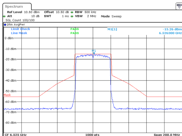
802.11ax40_6525MHz_RU_Full_Chain 2
