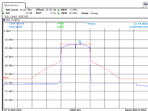
802.11ax160_6665MHz_RU_Full_Chain 0
