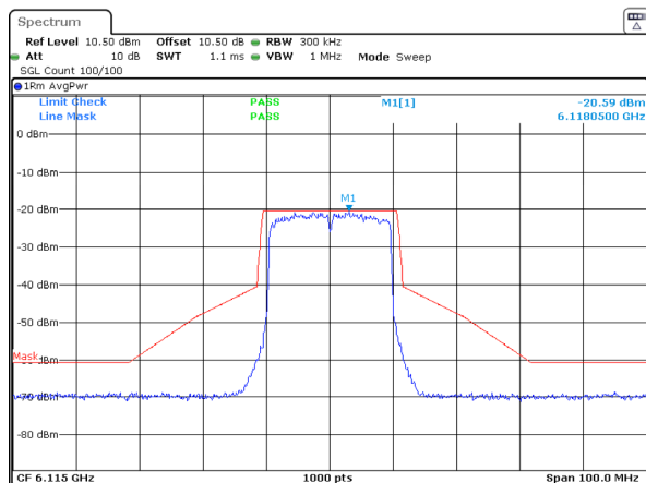
802.11ax20_6115MHz_RU_Full_Chain 2
