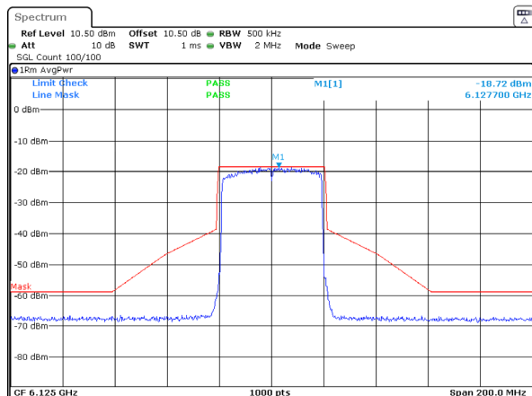
802.11ax40_6125MHz_RU_Full_Chain 3
