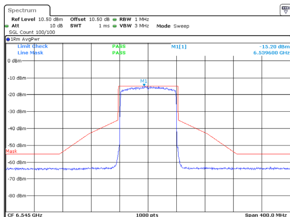
802.11ax80_6545MHz_RU_Full_Chain 0
