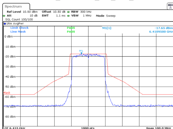
802.11ax20_6415MHz_RU_Full_Chain 2
