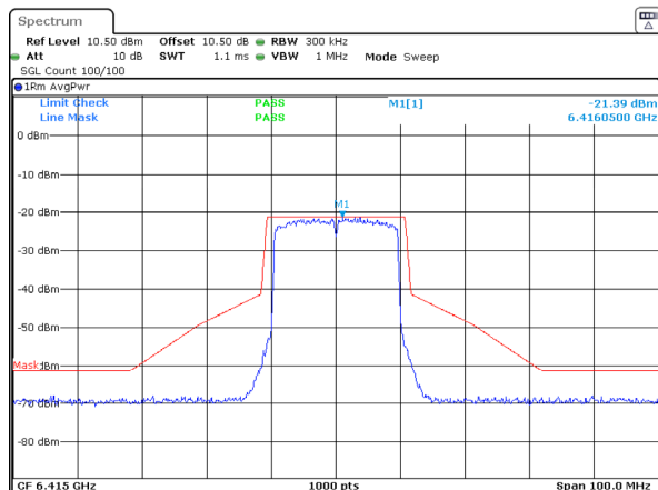
802.11ax20_6415MHz_RU_Full_Chain 1
