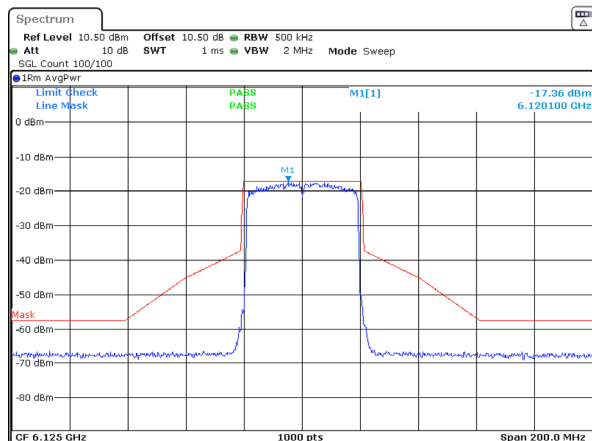
802.11ax40_6125MHz_RU_Full_Chain 2
