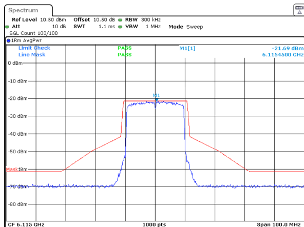
802.11ax20_6115MHz_RU_Full_Chain 3
