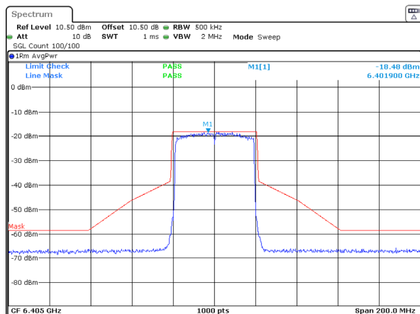
802.11ax40_6405MHz_RU_Full_Chain 1
