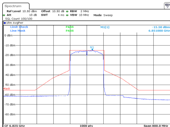
802.11ax160_6825MHz_RU_Full_Chain 0
