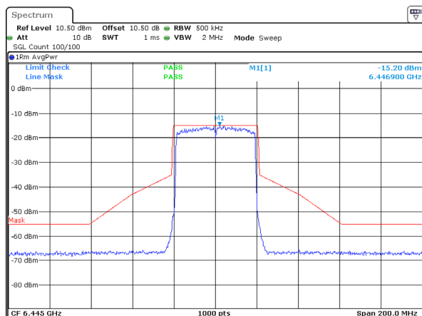
802.11ax40_6445MHz_RU_Full_Chain 2
