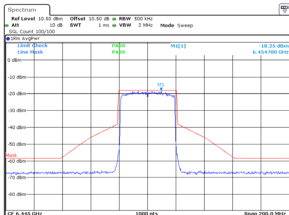
802.11ax40_6445MHz_RU_Full_Chain 3
