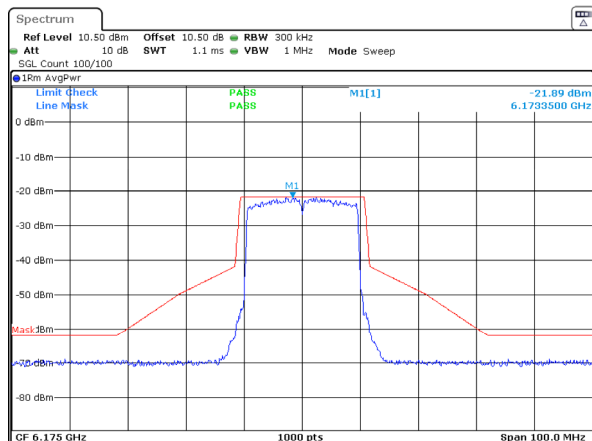
802.11ax20_6175MHz_RU_Full_Chain 1
