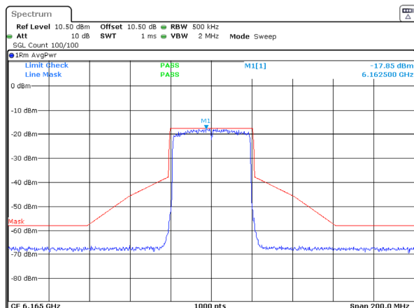
802.11ax40_6165MHz_RU_Full_Chain 3
