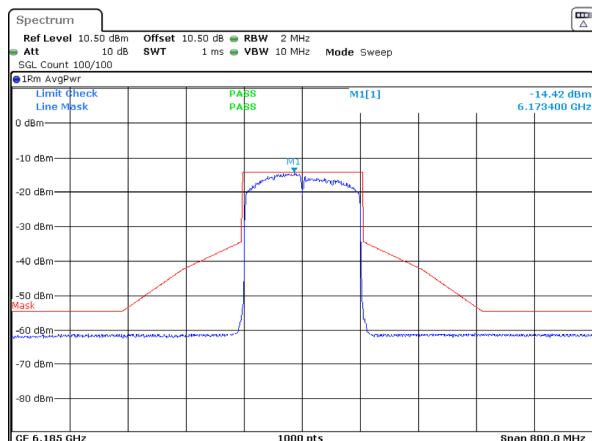
802.11ax160_6185MHz_RU_Full_Chain 3
