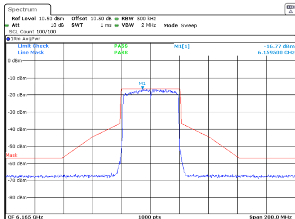
802.11ax40_6165MHz_RU_Full_Chain 2
