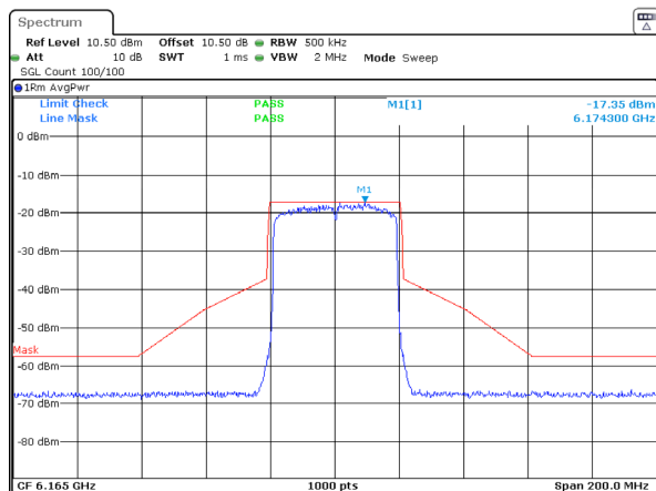
802.11ax40_6165MHz_RU_Full_Chain 1
