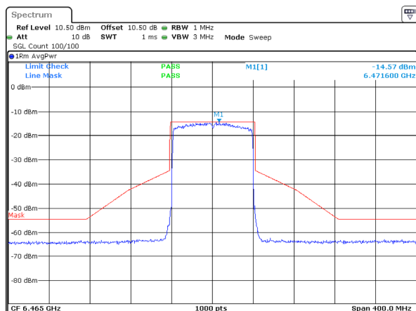
802.11ax80_6465MHz_RU_Full_Chain 0
