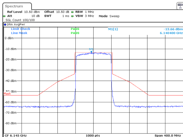
802.11ax80_6145MHz_RU_Full_Chain 2
