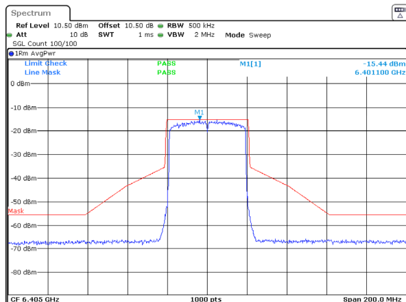
802.11ax40_6405MHz_RU_Full_Chain 2
