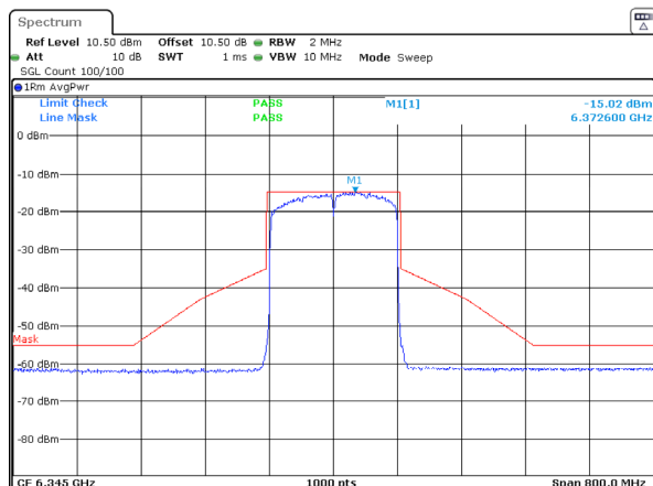
802.11ax160_6345MHz_RU_Full_Chain 3
