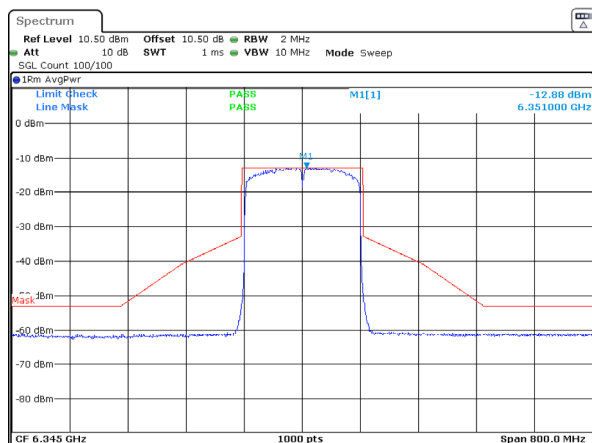
802.11ax160_6345MHz_RU_Full_Chain 2
