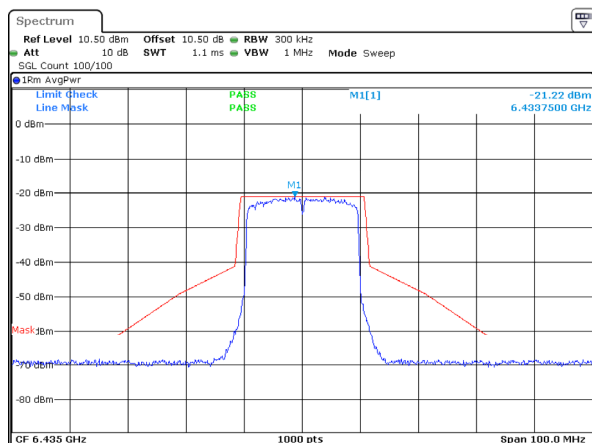
802.11ax20_6435MHz_RU_Full_Chain 0
