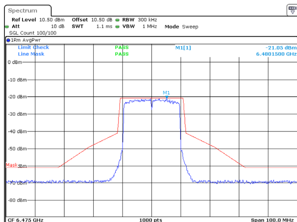
802.11ax20_6475MHz_RU_Full_Chain 0
