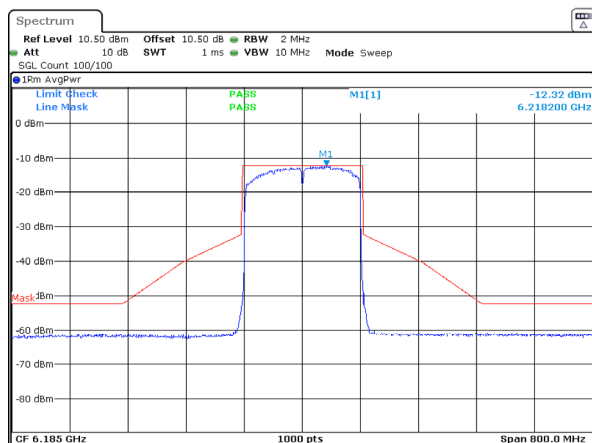
802.11ax160_6185MHz_RU_Full_Chain 2
