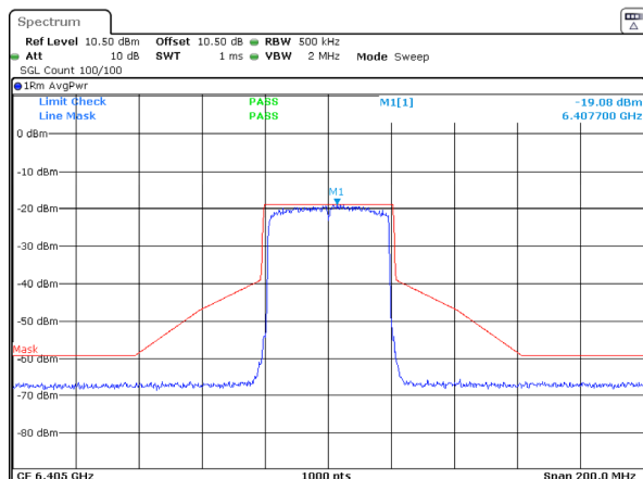
802.11ax40_6405MHz_RU_Full_Chain 3
