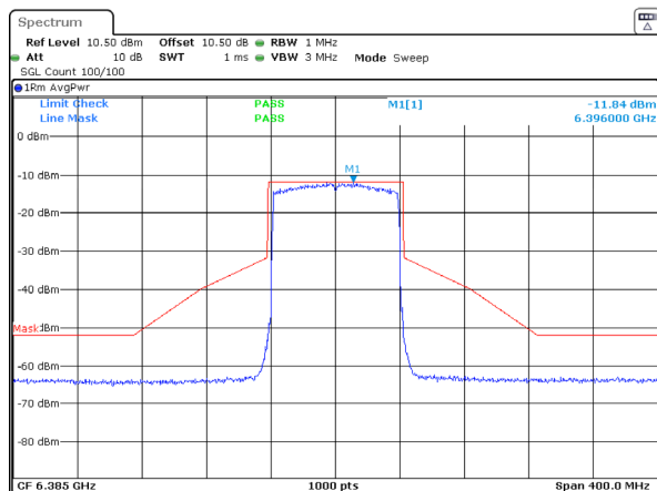
802.11ax80_6385MHz_RU_Full_Chain 2
