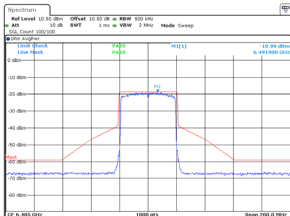
802.11ax40_6485MHz_RU_Full_Chain 3
