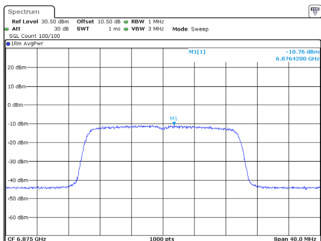
802.11ax20_6875MHz_RU_Full_Chain 1
