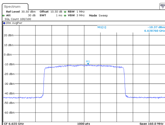
802.11ax80_6625MHz_RU_Full_Chain 0
