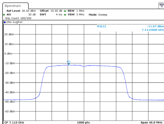
802.11ax20_7115MHz_RU_Full_Chain 3
