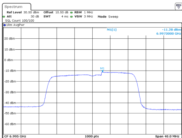
802.11ax20_6995MHz_RU_Full_Chain 1
