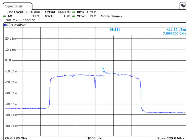
802.11ax160_6985MHz_RU_Full_Chain 1
