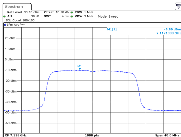
802.11ax20_7115MHz_RU_Full_Chain 2
