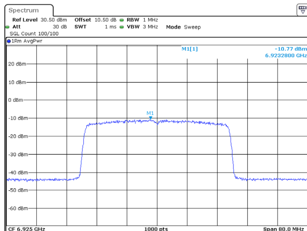
802.11ax40_6925MHz_RU_Full_Chain 3
