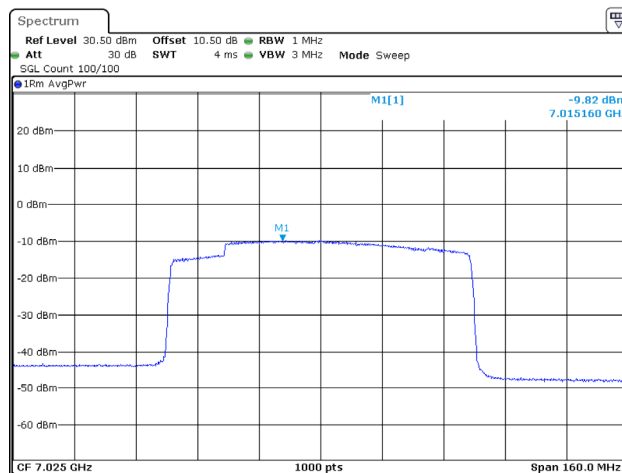
802.11ax80_7025MHz_RU_Full_Chain 2
