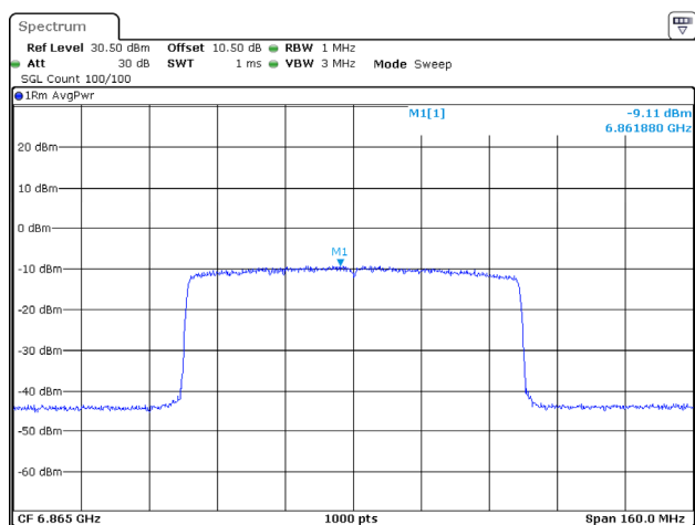
802.11ax80_6865MHz_RU_Full_Chain 2
