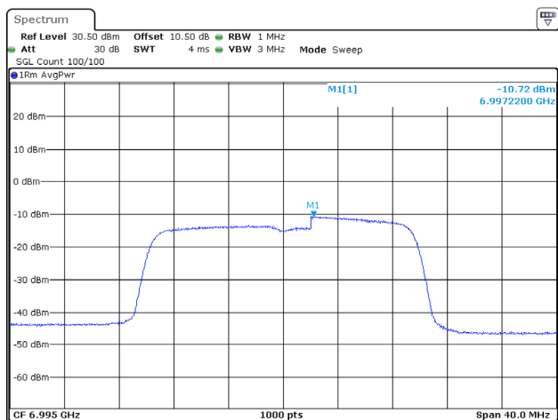
802.11ax20_6995MHz_RU_Full_Chain 3
