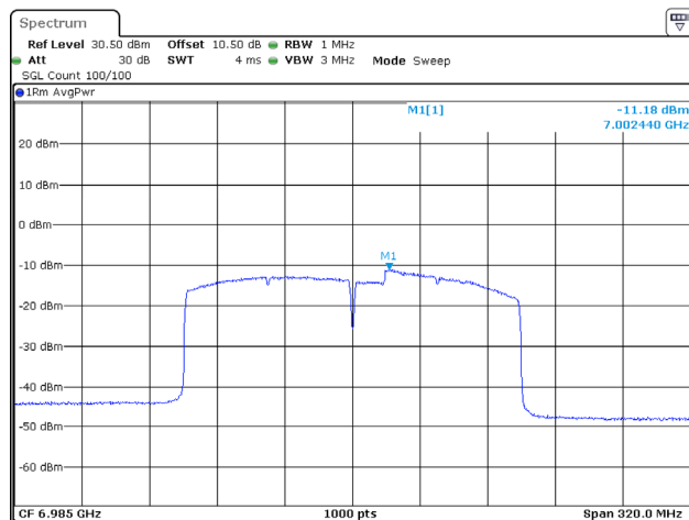
802.11ax160_6985MHz_RU_Full_Chain 3
