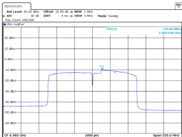
802.11ax160_6985MHz_RU_Full_Chain 2
