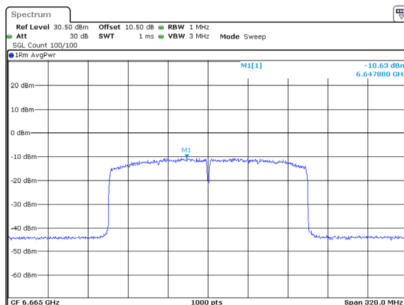
802.11ax160_6665MHz_RU_Full_Chain 1
