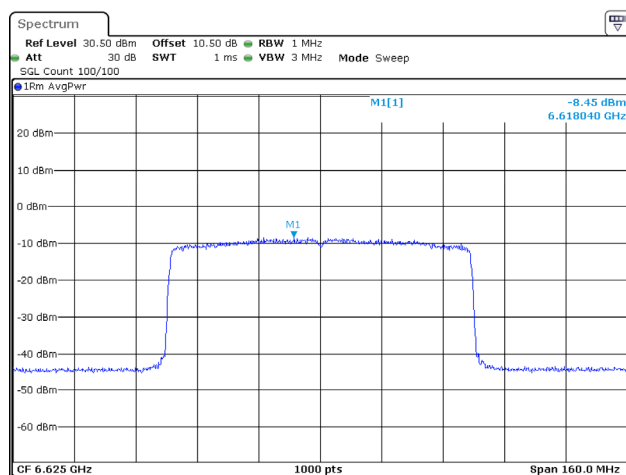
802.11ax80_6625MHz_RU_Full_Chain 2
