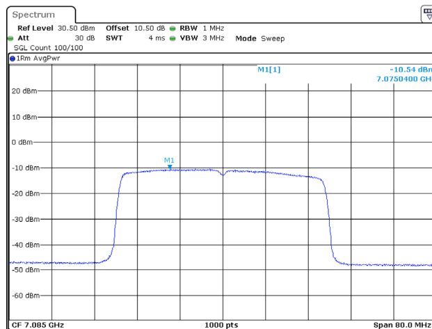
802.11ax40_7085MHz_RU_Full_Chain 0
