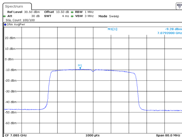
802.11ax40_7085MHz_RU_Full_Chain 2
