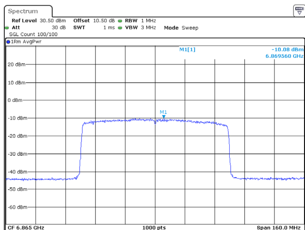
802.11ax80_6865MHz_RU_Full_Chain 1
