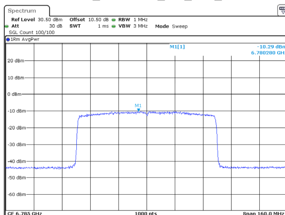
802.11ax80_6785MHz_RU_Full_Chain 3
