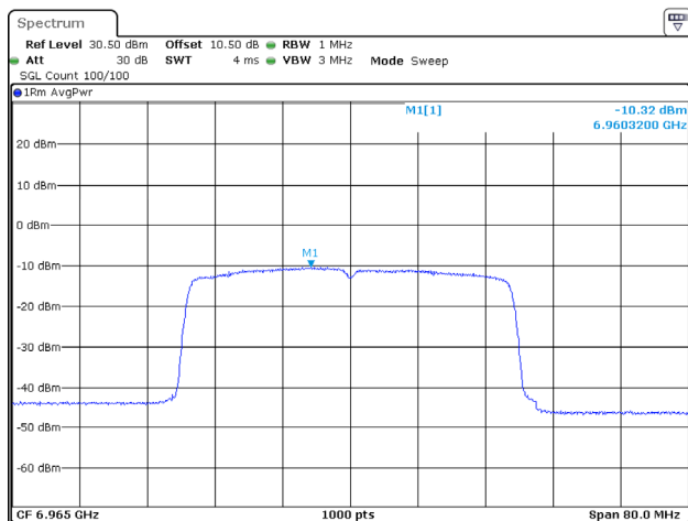
802.11ax40_6965MHz_RU_Full_Chain 0
