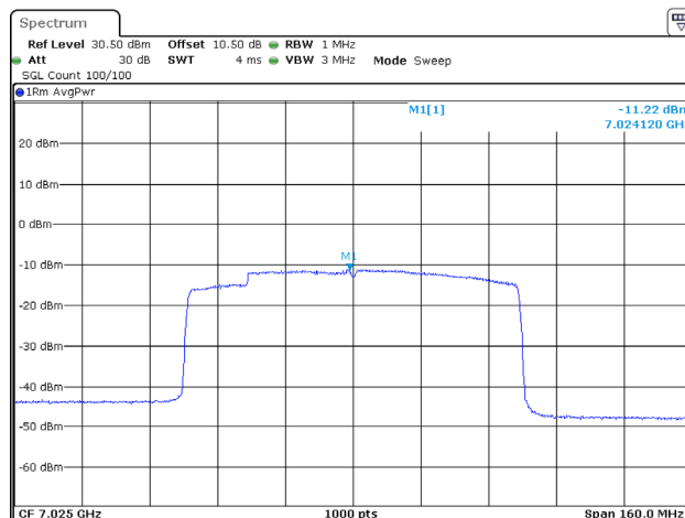
802.11ax80_7025MHz_RU_Full_Chain 1
