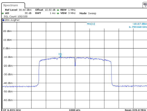
802.11ax160_6825MHz_RU_Full_Chain 0
