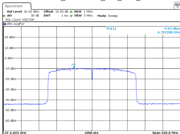
802.11ax160_6825MHz_RU_Full_Chain 2
