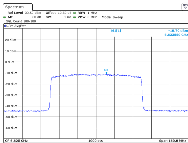
802.11ax80_6625MHz_RU_Full_Chain 3
