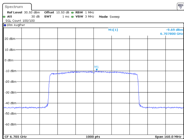
802.11ax80_6705MHz_RU_Full_Chain 1
