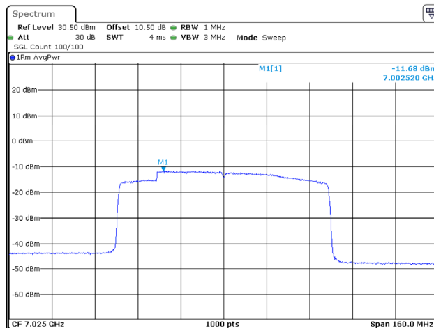
802.11ax80_7025MHz_RU_Full_Chain 3
