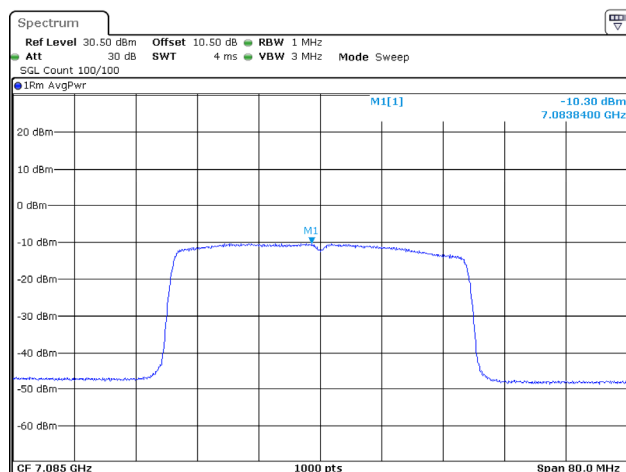
802.11ax40_7085MHz_RU_Full_Chain 1
