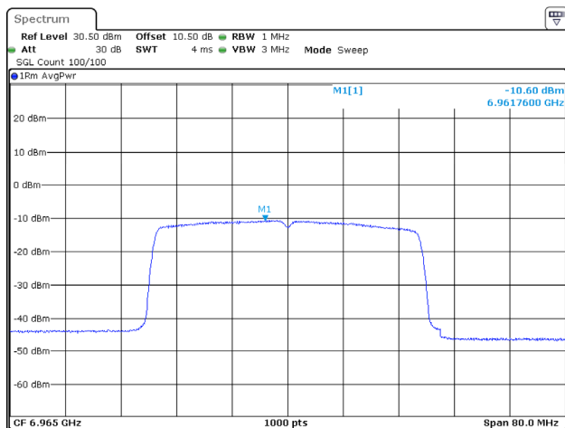
802.11ax40_6965MHz_RU_Full_Chain 3
