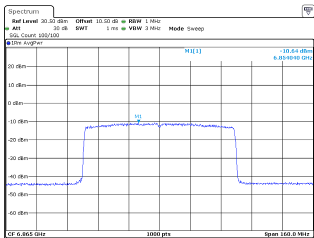
802.11ax80_6865MHz_RU_Full_Chain 3
