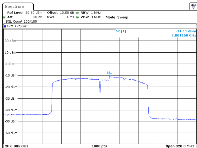
802.11ax160_6985MHz_RU_Full_Chain 0
