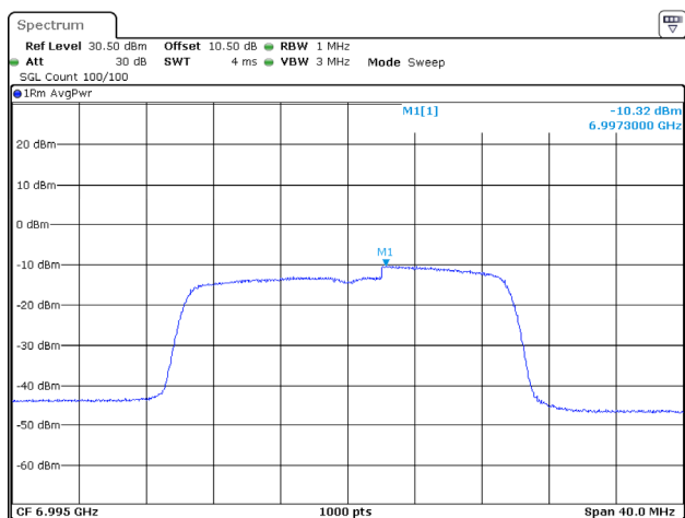
802.11ax20_6995MHz_RU_Full_Chain 2
