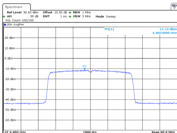
802.11ax40_6885MHz_RU_Full_Chain 3
