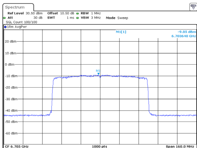
802.11ax80_6705MHz_RU_Full_Chain 2
