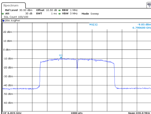
802.11ax160_6825MHz_RU_Full_Chain 1
