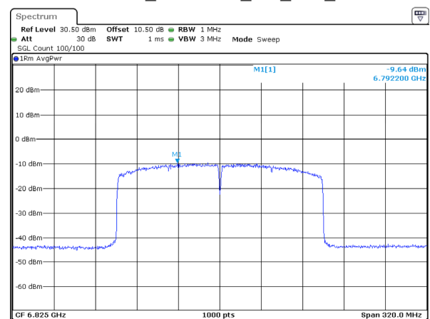
802.11ax160_6825MHz_RU_Full_Chain 3
