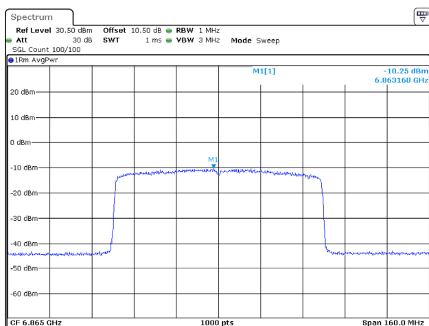
802.11ax80_6865MHz_RU_Full_Chain 0
