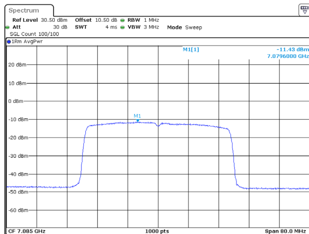
802.11ax40_7085MHz_RU_Full_Chain 3
