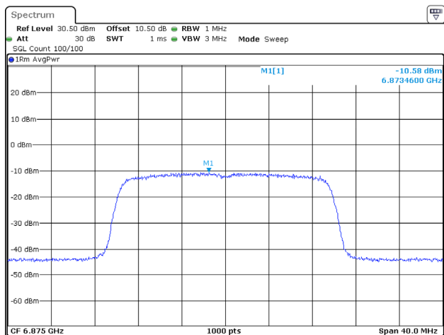
802.11ax20_6875MHz_RU_Full_Chain 3
