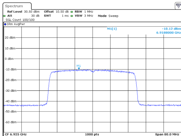
802.11ax40_6925MHz_RU_Full_Chain 2
