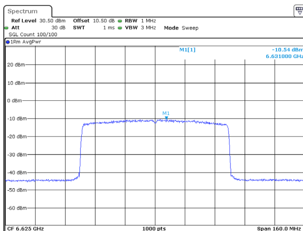
802.11ax80_6625MHz_RU_Full_Chain 1
