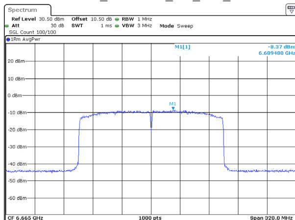
802.11ax160_6665MHz_RU_Full_Chain 2
