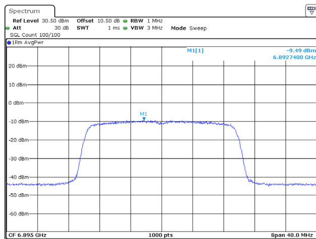
802.11ax20_6895MHz_RU_Full_Chain 2
