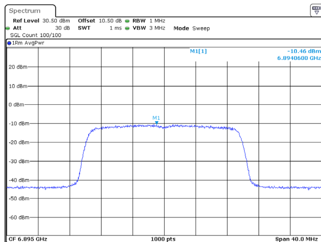
802.11ax20_6895MHz_RU_Full_Chain 3
