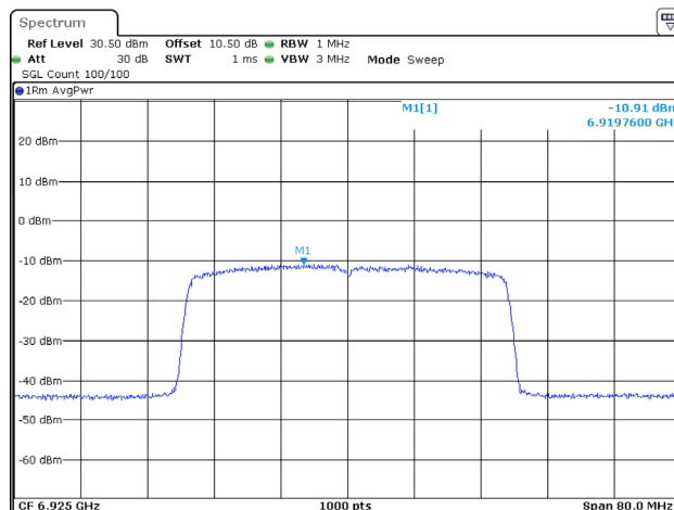
802.11ax40_6925MHz_RU_Full_Chain 0
