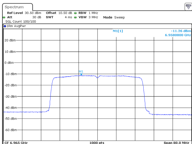
802.11ax40_6965MHz_RU_Full_Chain 1
