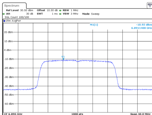
802.11ax20_6895MHz_RU_Full_Chain 1
