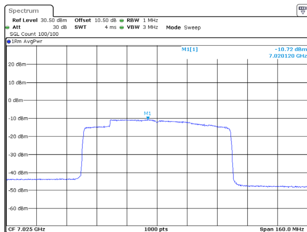
802.11ax80_7025MHz_RU_Full_Chain 0
