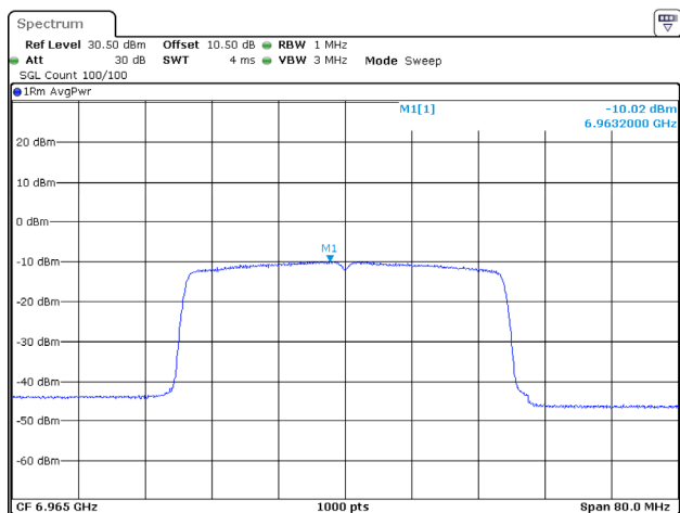
802.11ax40_6965MHz_RU_Full_Chain 2
