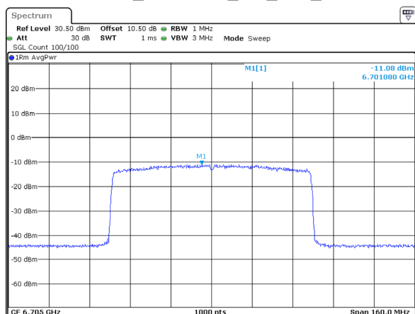
802.11ax80_6705MHz_RU_Full_Chain 3
