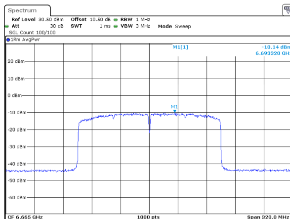
802.11ax160_6665MHz_RU_Full_Chain 0
