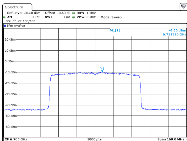
802.11ax80_6705MHz_RU_Full_Chain 0
