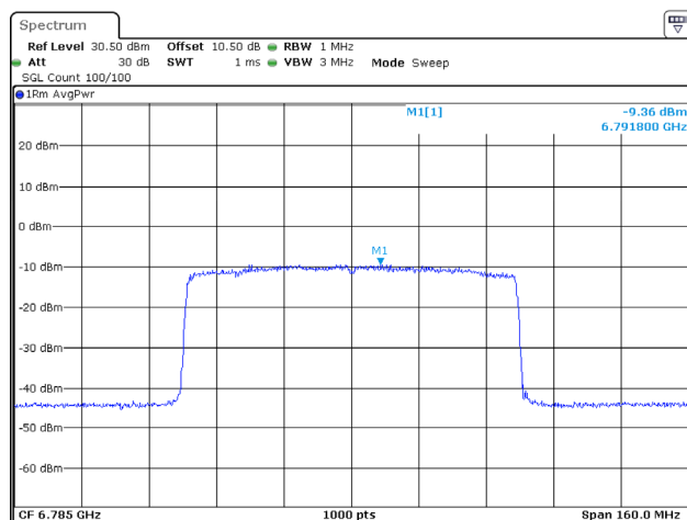
802.11ax80_6785MHz_RU_Full_Chain 2
