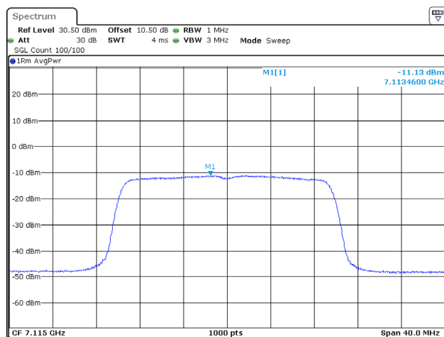
802.11ax20_7115MHz_RU_Full_Chain 1
