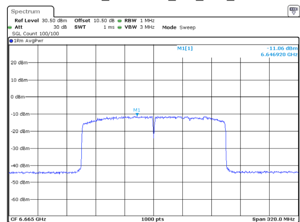
802.11ax160_6665MHz_RU_Full_Chain 3
