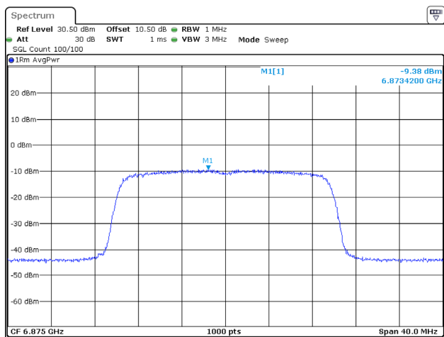
802.11ax20_6875MHz_RU_Full_Chain 2
