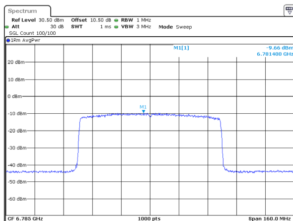
802.11ax80_6785MHz_RU_Full_Chain 1
