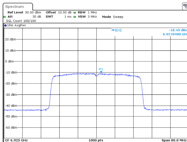
802.11ax40_6925MHz_RU_Full_Chain 1
