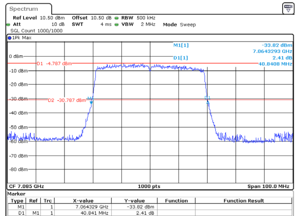
802.11ax40_7085MHz_RU_Full_Chain 0 40.841MHz
