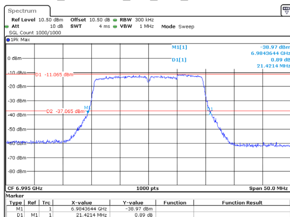
802.11ax20_6995MHz_RU_Full_Chain 1 21.421MHz
