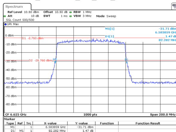
802.11ax80_6625MHz_RU_Full_Chain 3 82.282MHz
