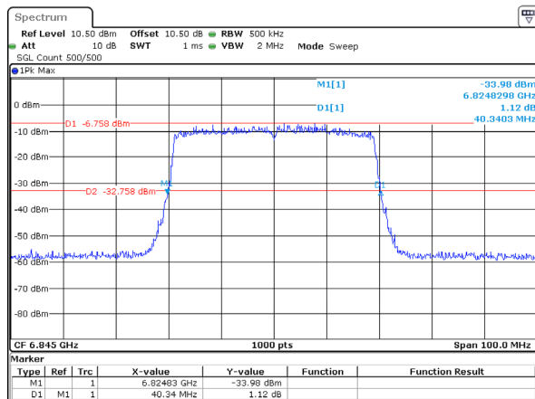
802.11ax40_6845MHz_RU_Full_Chain 2 40.340MHz
