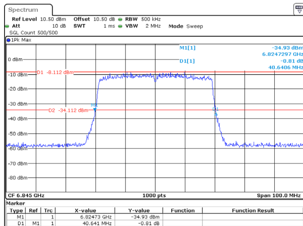
802.11ax40_6845MHz_RU_Full_Chain 0 40.641MHz
