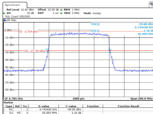
802.11ax80_6785MHz_RU_Full_Chain 2 82.883MHz
