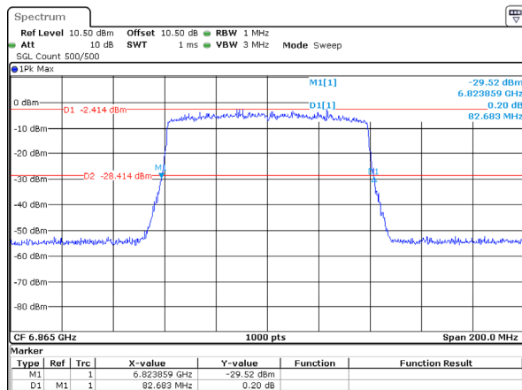
802.11ax80_6865MHz_RU_Full_Chain 2 82.683MHz
