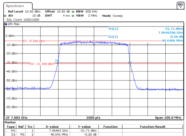
802.11ax40_7085MHz_RU_Full_Chain 1 40.641MHz
