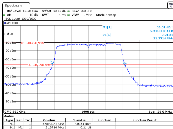
802.11ax20_6995MHz_RU_Full_Chain 0 21.371MHz
