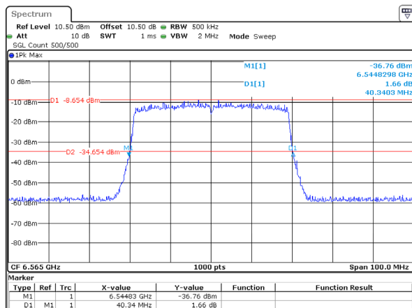
802.11ax40_6565MHz_RU_Full_Chain 0 40.340MHz
