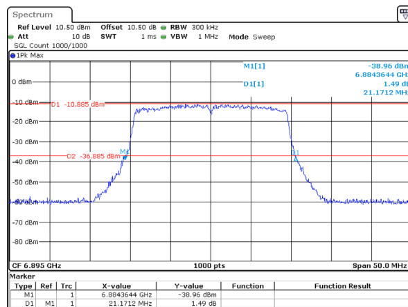
802.11ax20_6895MHz_RU_Full_Chain 2 21.171MHz
