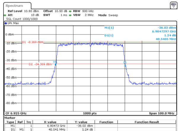
802.11ax40_6925MHz_RU_Full_Chain 3 40.541MHz
