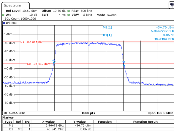
802.11ax40_6965MHz_RU_Full_Chain 0 40.541MHz
