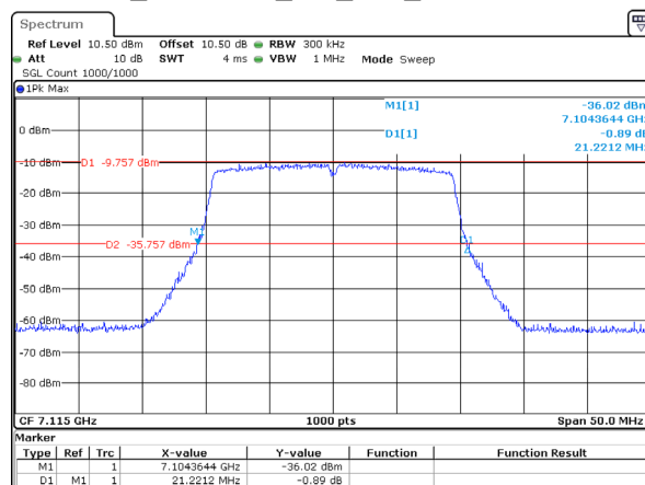
802.11ax20_7115MHz_RU_Full_Chain 1 21.221MHz
