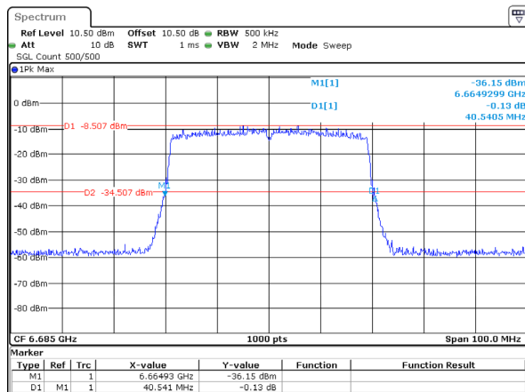
802.11ax40_6685MHz_RU_Full_Chain 1 40.541MHz
