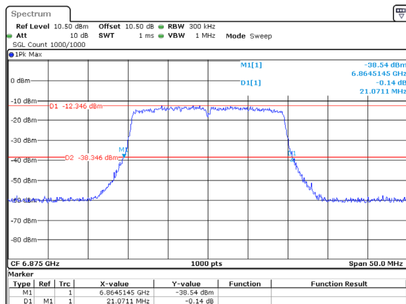
802.11ax20_6875MHz_RU_Full_Chain 0 21.071MHz
