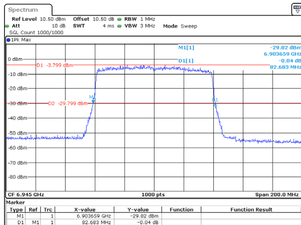
802.11ax80_6945MHz_RU_Full_Chain 1 82.683MHz
