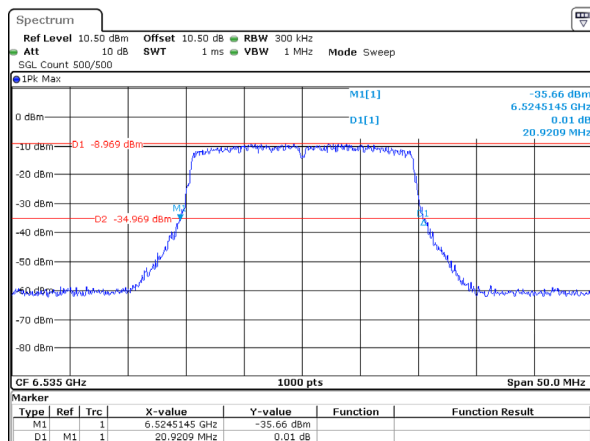
802.11ax20_6535MHz_RU_Full_Chain 2 20.921MHz
