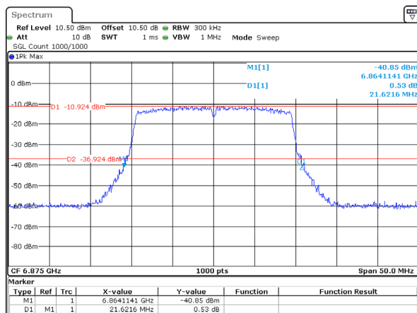
802.11ax20_6875MHz_RU_Full_Chain 2 21.622MHz
