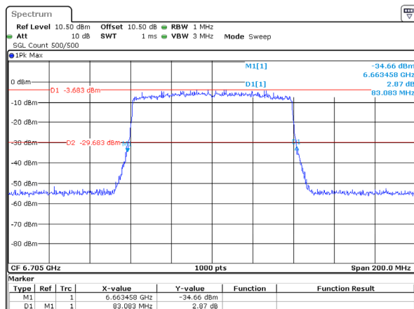
802.11ax80_6705MHz_RU_Full_Chain 1 83.083MHz
