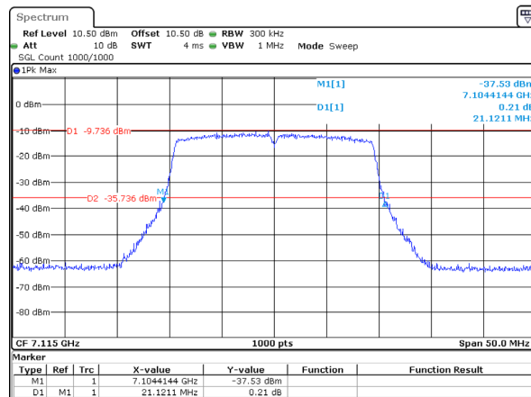
802.11ax20_7115MHz_RU_Full_Chain 3 21.121MHz
