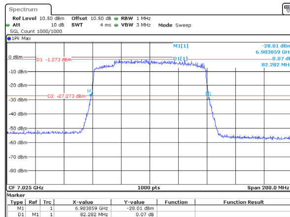
802.11ax80_7025MHz_RU_Full_Chain 1 82.282MHz
