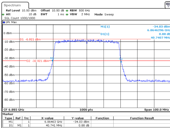
802.11ax40_6885MHz_RU_Full_Chain 2 40.741MHz
