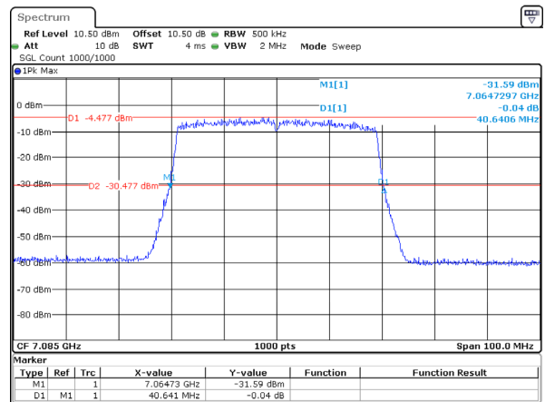
802.11ax40_7085MHz_RU_Full_Chain 2 40.641MHz
