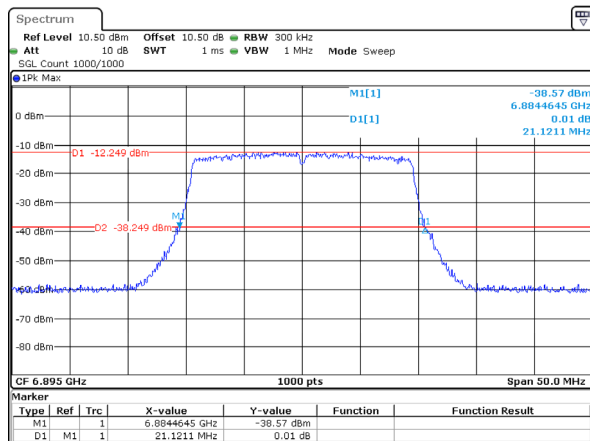
802.11ax20_6895MHz_RU_Full_Chain 1 21.121MHz
