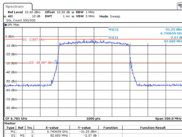
802.11ax80_6785MHz_RU_Full_Chain 3 82.683MHz
