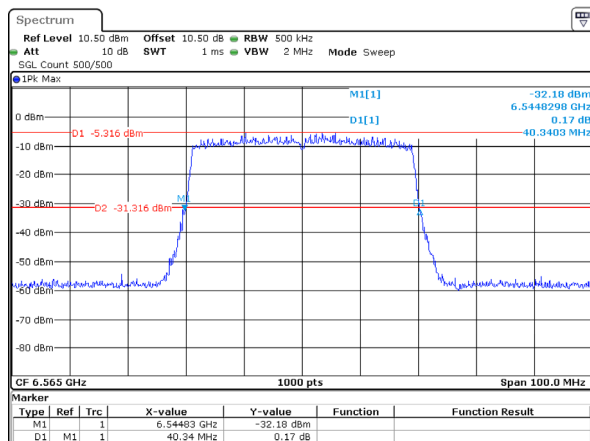
802.11ax40_6565MHz_RU_Full_Chain 2 40.340MHz
