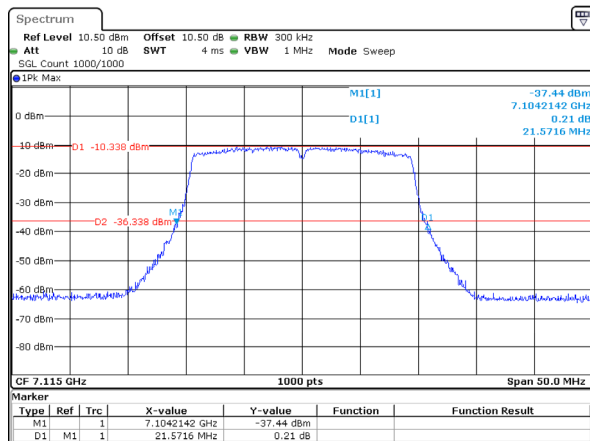
802.11ax20_7115MHz_RU_Full_Chain 0 21.572MHz
