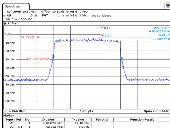
802.11ax80_6865MHz_RU_Full_Chain 0 82.082MHz
