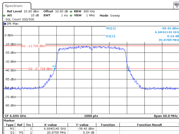
802.11ax20_6695MHz_RU_Full_Chain 3 20.871MHz
