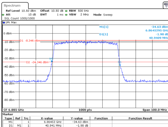
802.11ax40_6885MHz_RU_Full_Chain 1 40.941MHz
