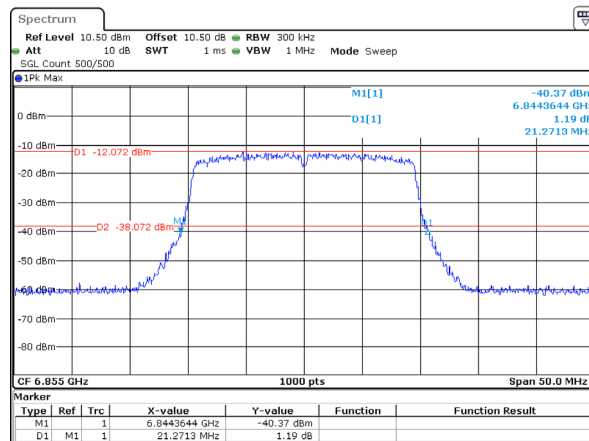
802.11ax20_6855MHz_RU_Full_Chain 3 21.271MHz
