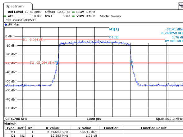
802.11ax80_6785MHz_RU_Full_Chain 1 82.883MHz
