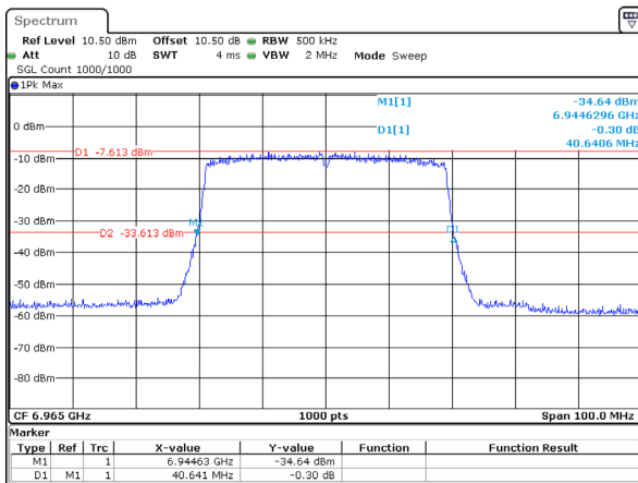
802.11ax40_6965MHz_RU_Full_Chain 2 40.641MHz
