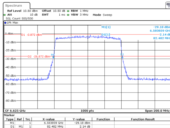
802.11ax80_6625MHz_RU_Full_Chain 2 82.482MHz
