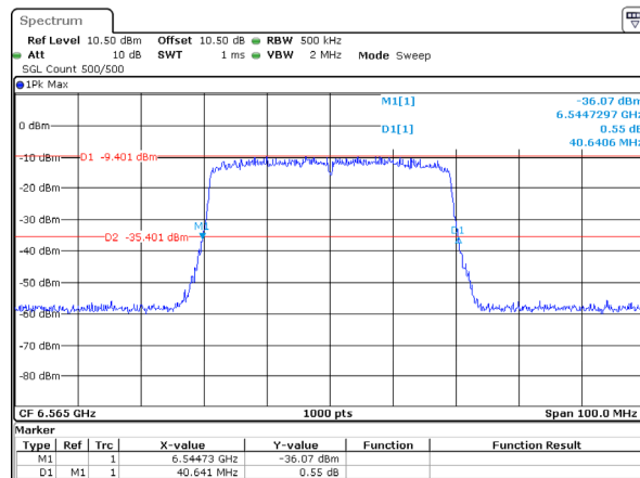
802.11ax40_6565MHz_RU_Full_Chain 1 40.641MHz
