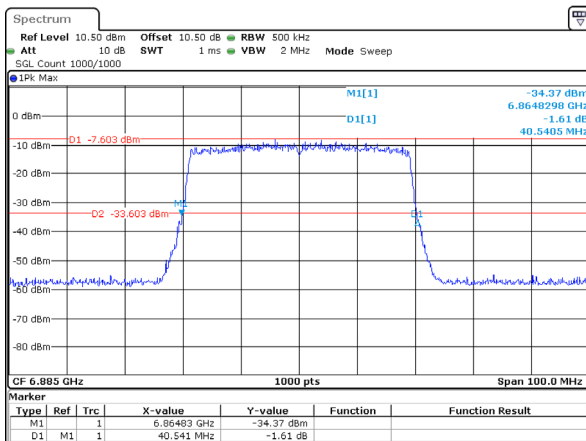
802.11ax40_6885MHz_RU_Full_Chain 3 40.541MHz
