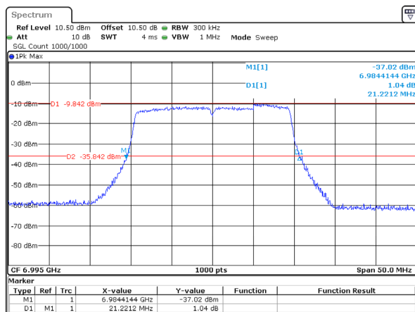
802.11ax20_6995MHz_RU_Full_Chain 2 21.221MHz
