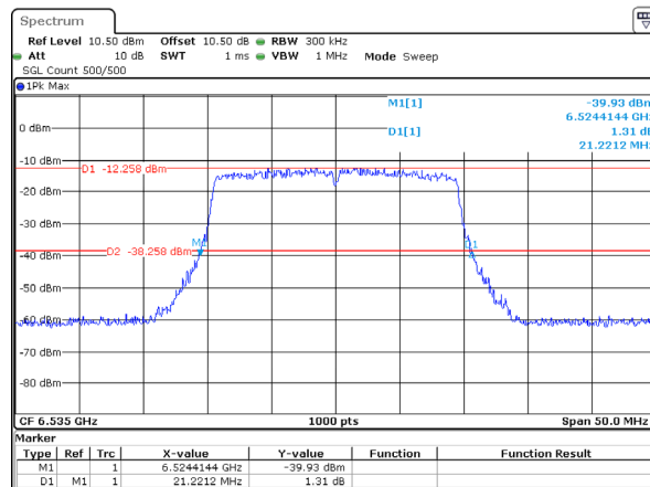
802.11ax20_6535MHz_RU_Full_Chain 3 21.221MHz
