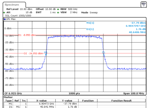
802.11ax40_6925MHz_RU_Full_Chain 1 40.641MHz
