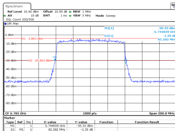
802.11ax80_6785MHz_RU_Full_Chain 0 82.282MHz
