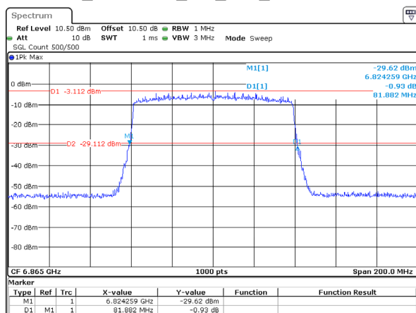
802.11ax80_6865MHz_RU_Full_Chain 3 81.882MHz
