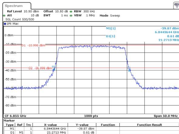
802.11ax20_6855MHz_RU_Full_Chain 2 21.271MHz
