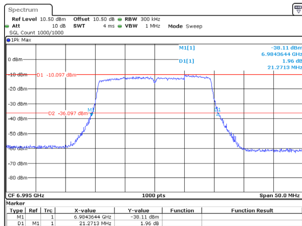
802.11ax20_6995MHz_RU_Full_Chain 3 21.271MHz
