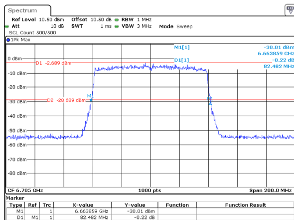
802.11ax80_6705MHz_RU_Full_Chain 3 82.482MHz
