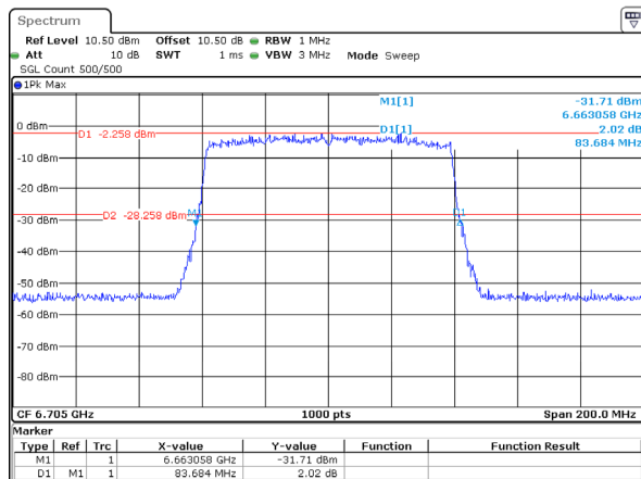
802.11ax80_6705MHz_RU_Full_Chain 2 83.684MHz
