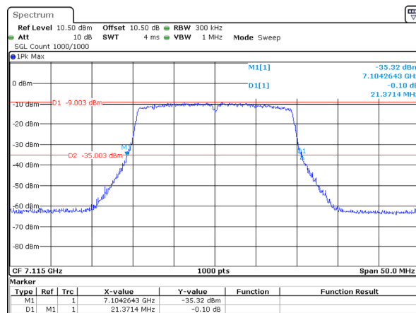
802.11ax20_7115MHz_RU_Full_Chain 2 21.371MHz
