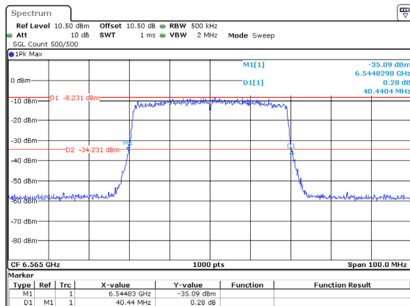
802.11ax40_6565MHz_RU_Full_Chain 3 40.440MHz
