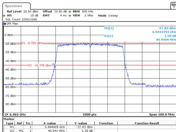
802.11ax40_6965MHz_RU_Full_Chain 3 40.941MHz
