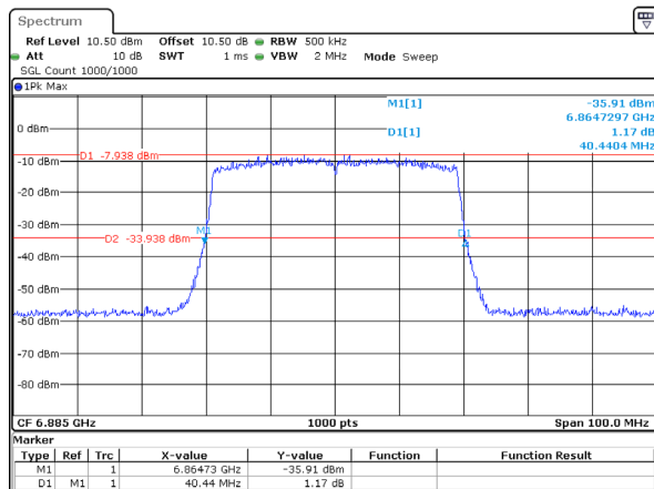
802.11ax40_6885MHz_RU_Full_Chain 0 40.440MHz
