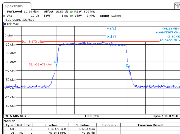
802.11ax40_6685MHz_RU_Full_Chain 2 40.641MHz
