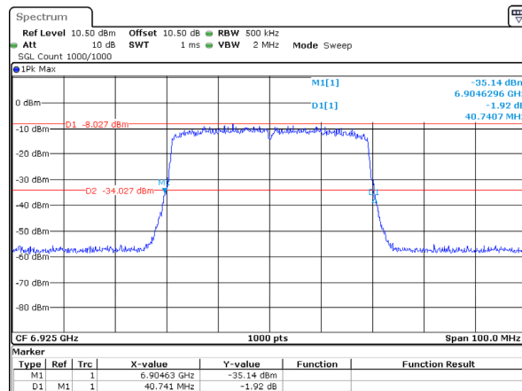
802.11ax40_6925MHz_RU_Full_Chain 0 40.741MHz
