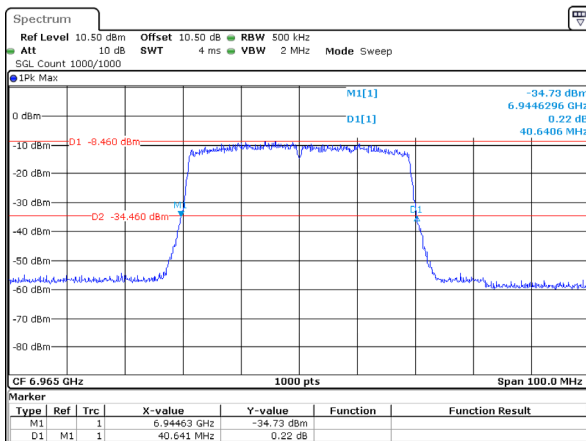
802.11ax40_6965MHz_RU_Full_Chain 1 40.641MHz
