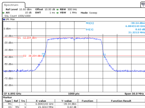
802.11ax20_6895MHz_RU_Full_Chain 0 21.321MHz
