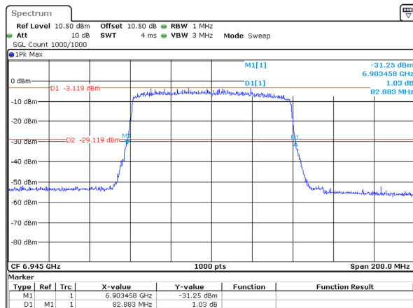
802.11ax80_6945MHz_RU_Full_Chain 0 82.883MHz
