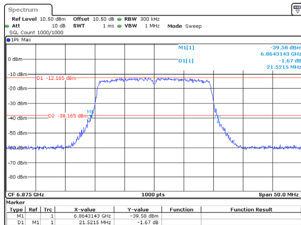
802.11ax20_6875MHz_RU_Full_Chain 1 21.522MHz
