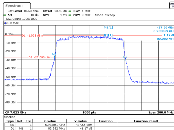
802.11ax80_7025MHz_RU_Full_Chain 0 82.282MHz
