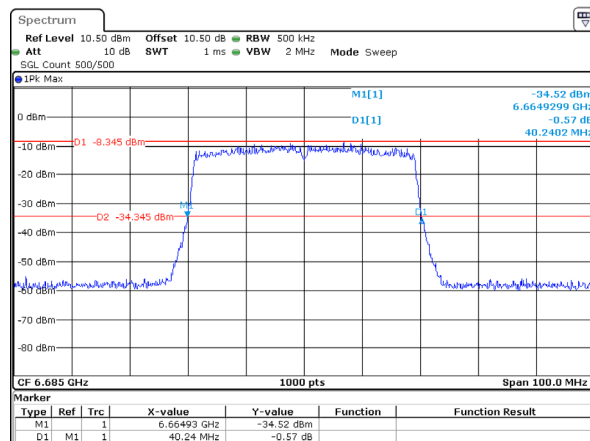
802.11ax40_6685MHz_RU_Full_Chain 0 40.240MHz
