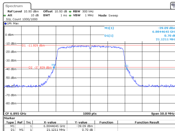
802.11ax20_6895MHz_RU_Full_Chain 3 21.121MHz
