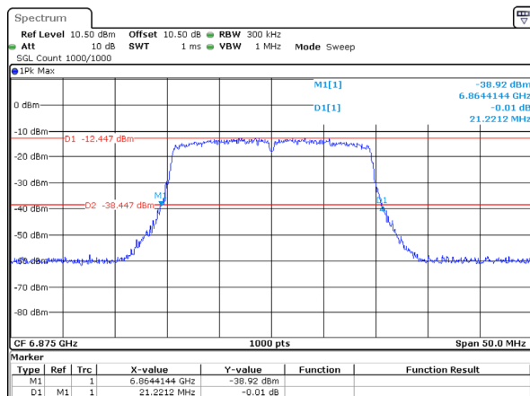
802.11ax20_6875MHz_RU_Full_Chain 3 21.221MHz
