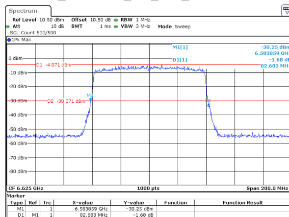
802.11ax80_6625MHz_RU_Full_Chain 0 82.683MHz
