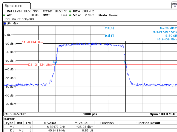
802.11ax40_6845MHz_RU_Full_Chain 3 40.641MHz
