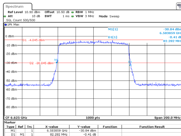
802.11ax80_6625MHz_RU_Full_Chain 1 82.282MHz
