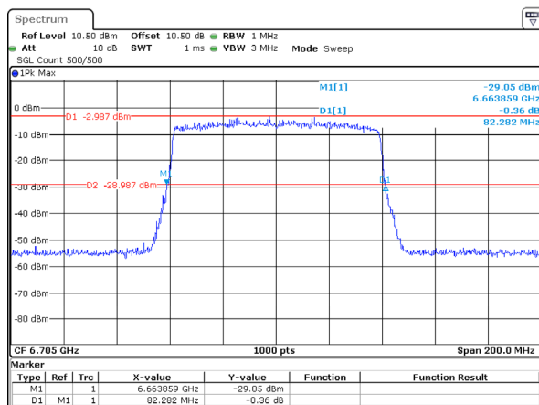
802.11ax80_6705MHz_RU_Full_Chain 0 82.282MHz
