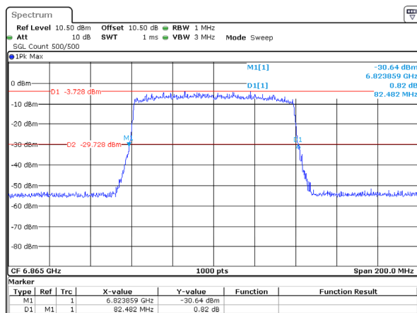
802.11ax80_6865MHz_RU_Full_Chain 1 82.482MHz
