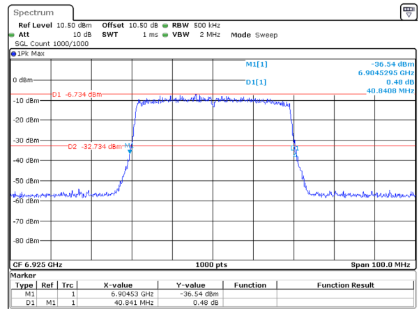
802.11ax40_6925MHz_RU_Full_Chain 2 40.841MHz
