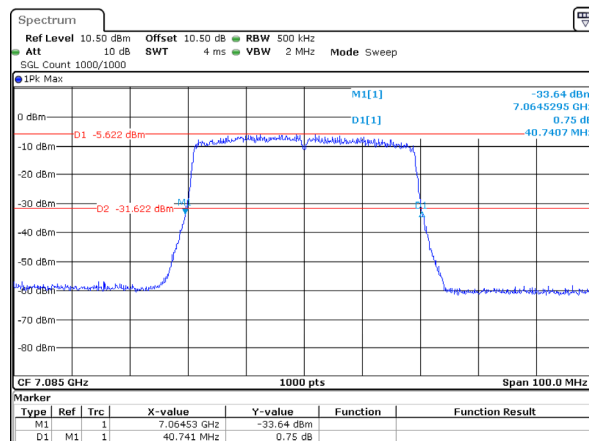
802.11ax40_7085MHz_RU_Full_Chain 3 40.741MHz
