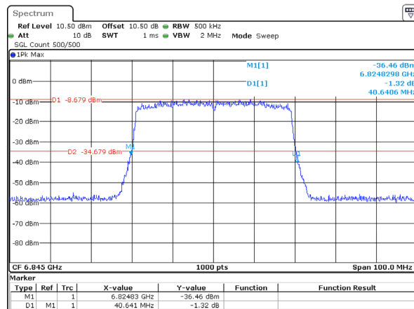
802.11ax40_6845MHz_RU_Full_Chain 1 40.641MHz
