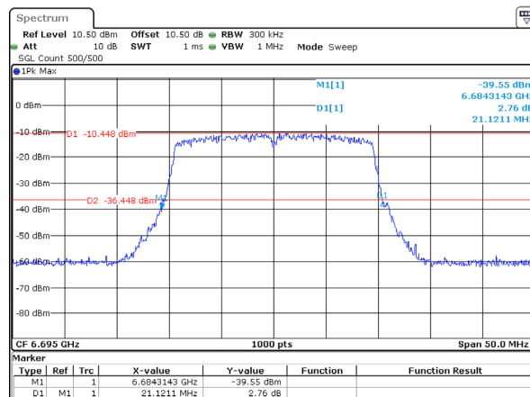
802.11ax20_6695MHz_RU_Full_Chain 2 21.121MHz
