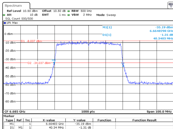
802.11ax40_6685MHz_RU_Full_Chain 3 40.340MHz
