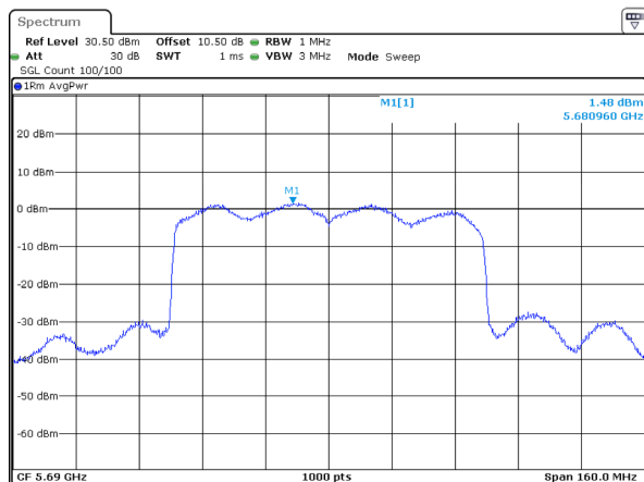
802.11ax80_5690MHz_RU_Full_Chain 1
