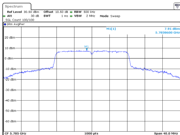
802.11a_5785MHz_Chain 0
