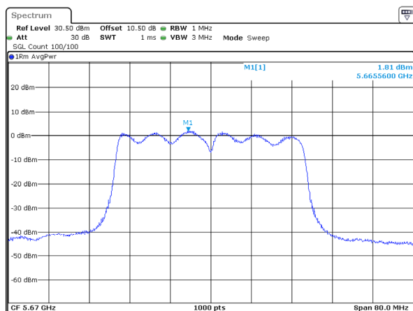
802.11ax40_5670MHz_RU_Full_Chain 3
