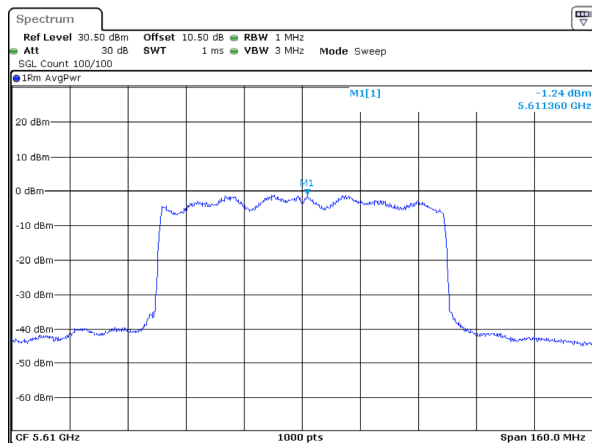
802.11ax80_5610MHz_RU_Full_Chain 2
