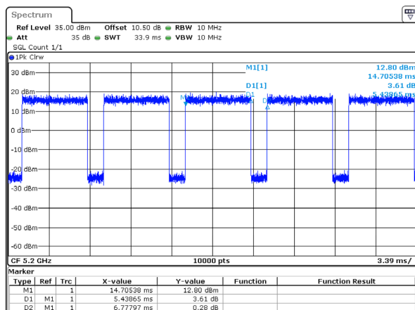
802.11ax20_5200MHz_RU_Full_Chain 0
