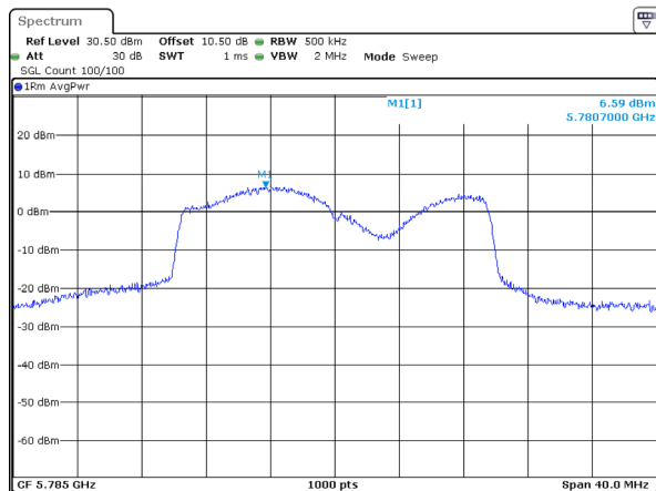
802.11ax20_5785MHz_RU_Full_Chain 2
