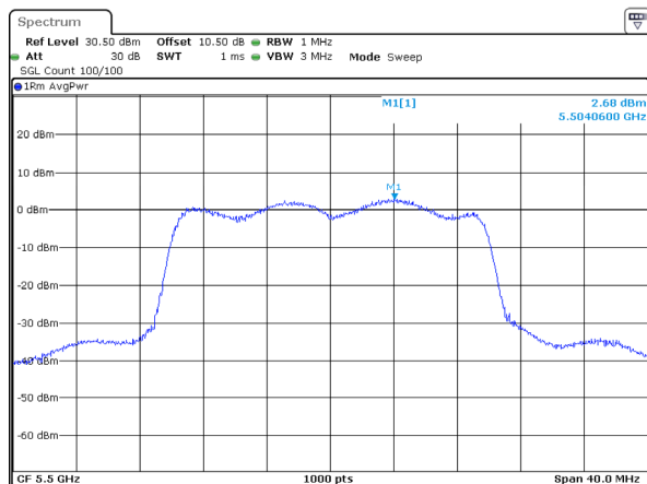
802.11ax20_5500MHz_RU_Full_Chain 3
