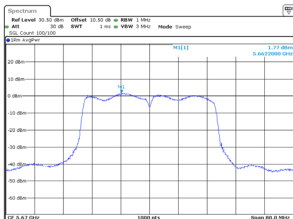
802.11ax40_5670MHz_RU_Full_Chain 0
