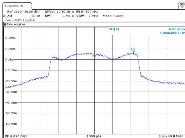
802.11ax20_5825MHz_RU_Full_Chain 2
