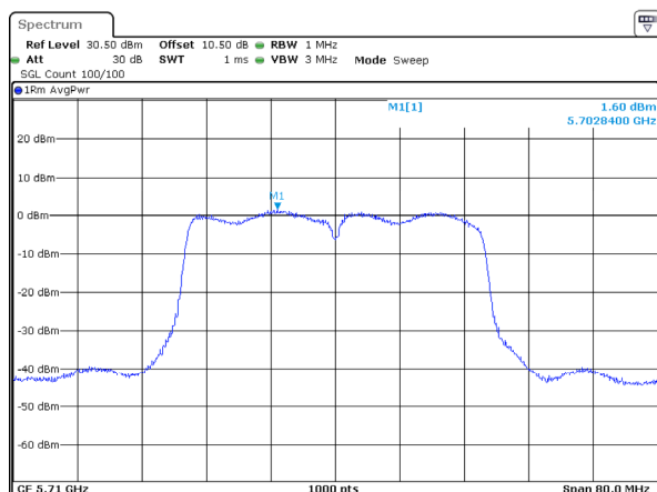
802.11ax40_5710MHz_RU_Full_Chain 0
