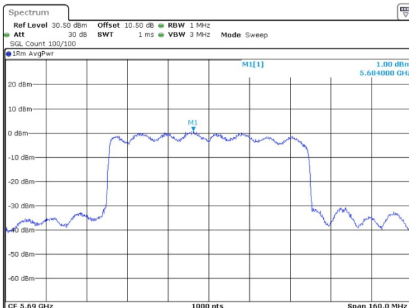
802.11ax80_5690MHz_RU_Full_Chain 0
