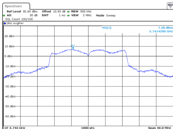
802.11ac20_5745MHz_Chain 3
