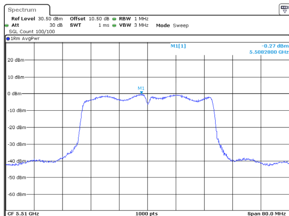
802.11ax40_5510MHz_RU_Full_Chain 2
