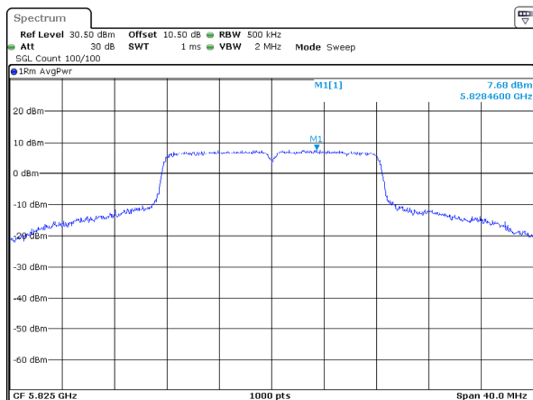
802.11a_5825MHz_Chain 3
