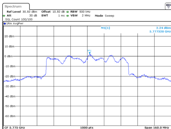
802.11ax80_5775MHz_RU_Full_Chain 2
