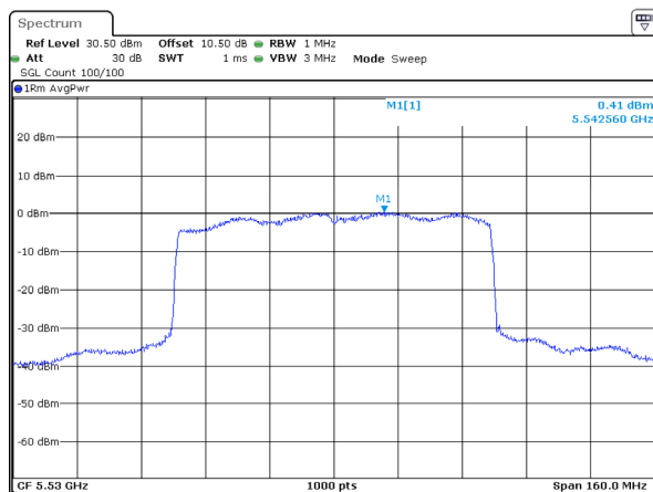
802.11ax80_5530MHz_RU_Full_Chain 1
