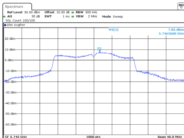
802.11ac20_5745MHz_Chain 2
