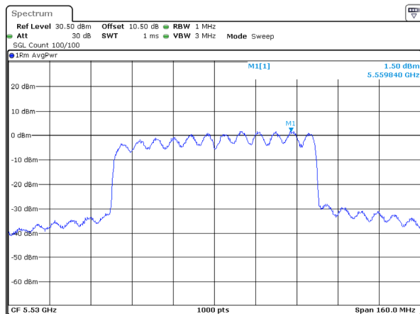
802.11ax80_5530MHz_RU_Full_Chain 3
