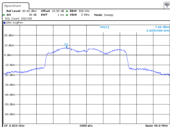
802.11ax20_5825MHz_RU_Full_Chain 3
