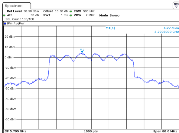
802.11ax40_5795MHz_RU_Full_Chain 3
