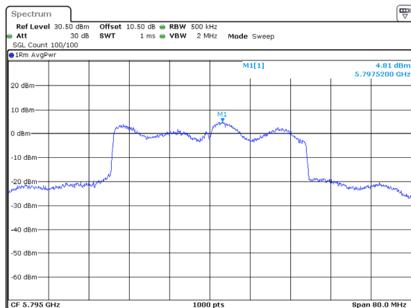
802.11ax40_5795MHz_RU_Full_Chain 2
