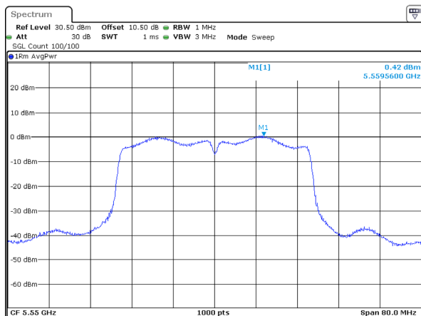
802.11ax40_5550MHz_RU_Full_Chain 2
