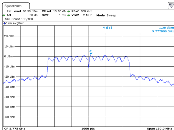
802.11ac80_5775MHz_Chain 3
