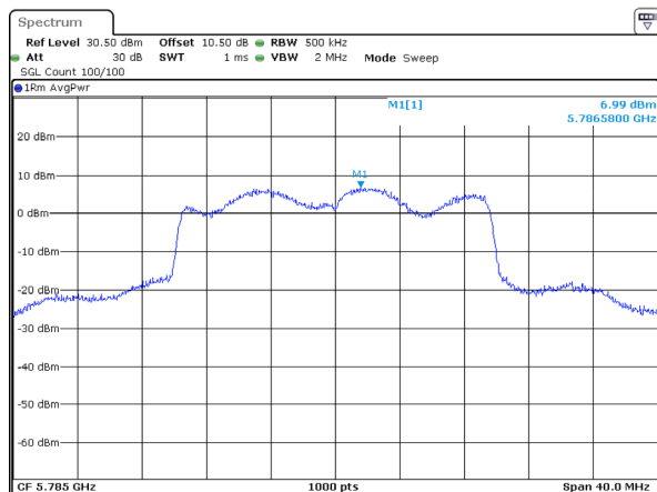
802.11ax20_5785MHz_RU_Full_Chain 3
