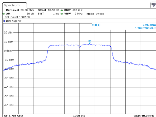
802.11a_5785MHz_Chain 3
