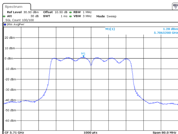
802.11ax40_5710MHz_RU_Full_Chain 3
