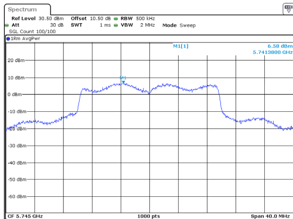
802.11ax20_5745MHz_RU_Full_Chain 3
