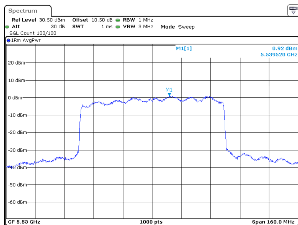
802.11ax80_5530MHz_RU_Full_Chain 0
