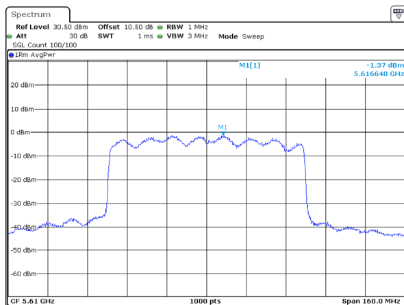
802.11ax80_5610MHz_RU_Full_Chain 0
