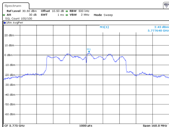
802.11ac80_5775MHz_Chain 2
