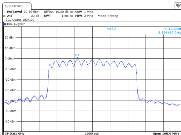
802.11ax80_5610MHz_RU_Full_Chain 3
