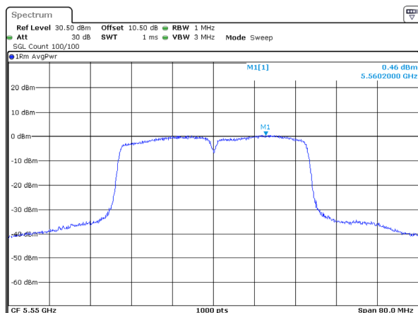
802.11ax40_5550MHz_RU_Full_Chain 1
