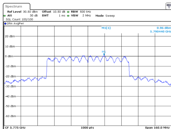
802.11ax80_5775MHz_RU_Full_Chain 3
