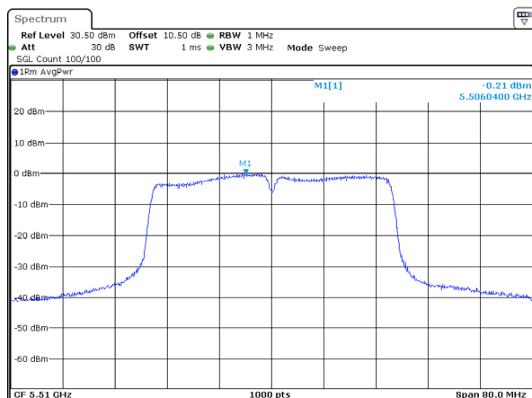
802.11ax40_5510MHz_RU_Full_Chain 1
