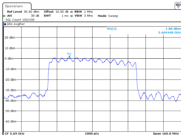
802.11ax80_5690MHz_RU_Full_Chain 3
