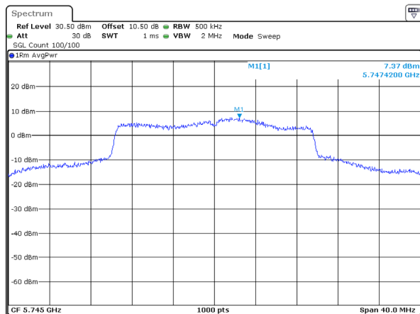
802.11ax20_5745MHz_RU_Full_Chain 2
