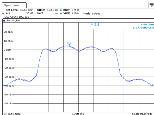
802.11ax20_5580MHz_RU_Full_Chain 3
