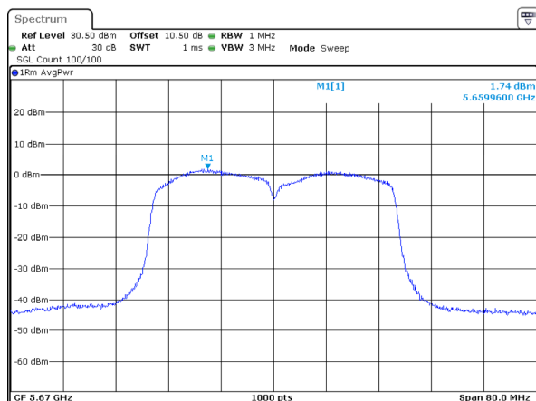
802.11ax40_5670MHz_RU_Full_Chain 1
