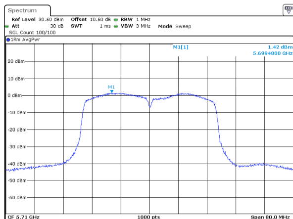
802.11ax40_5710MHz_RU_Full_Chain 1
