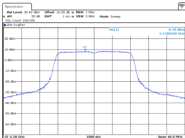
802.11a_5280MHz_Chain 0
