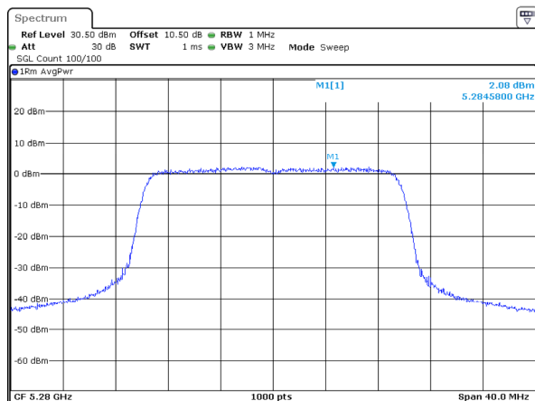
802.11ax20_5280MHz_RU_Full_Chain 0
