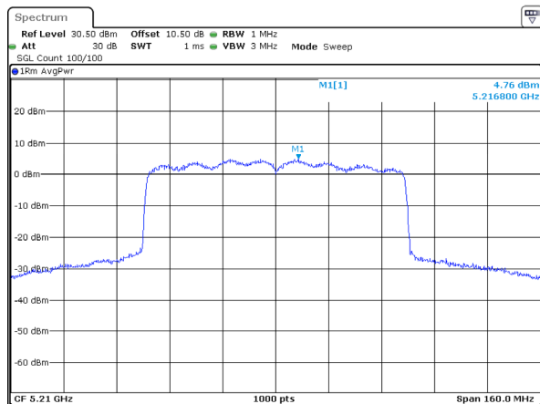
802.11ax80_5210MHz_RU_Full_Chain 2
