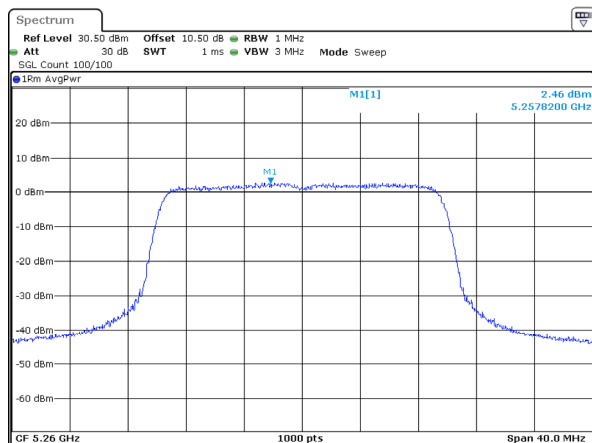
802.11ax20_5260MHz_RU_Full_Chain 0
