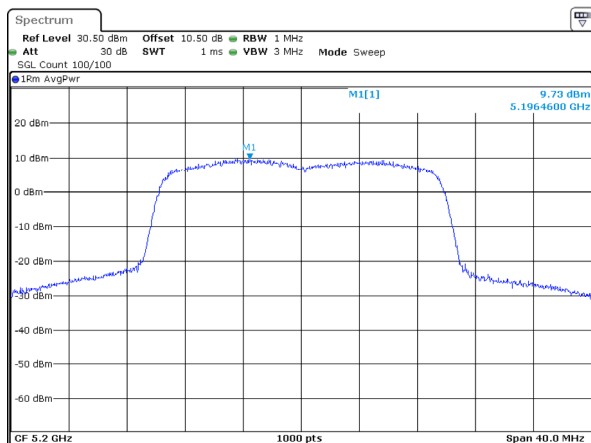
802.11ax20_5200MHz_RU_Full_Chain 2
