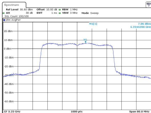
802.11ax40_5230MHz_RU_Full_Chain 2
