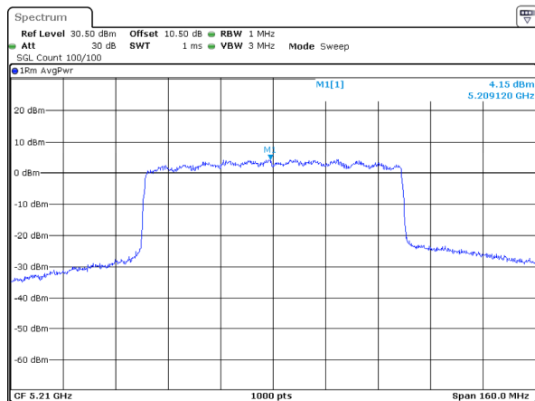
802.11ax80_5210MHz_RU_Full_Chain 3
