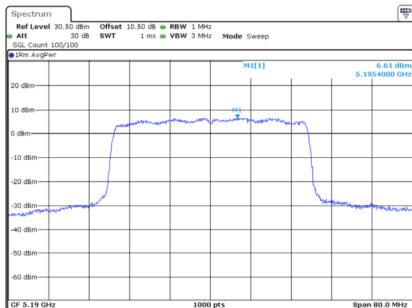
802.11ax40_5190MHz_RU_Full_Chain 3
