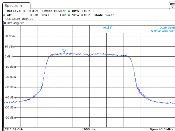
802.11ax20_5320MHz_RU_Full_Chain 1
