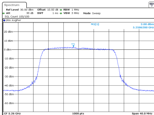
802.11ax20_5260MHz_RU_Full_Chain 1
