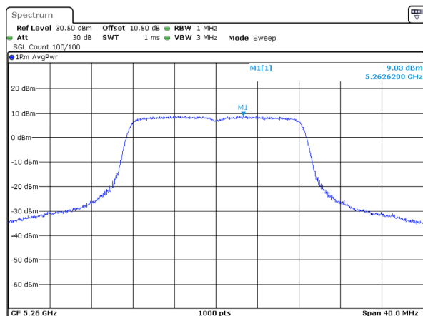
802.11a_5260MHz_Chain 0
