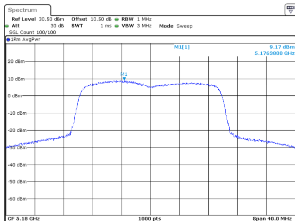
802.11ax20_5180MHz_RU_Full_Chain 2
