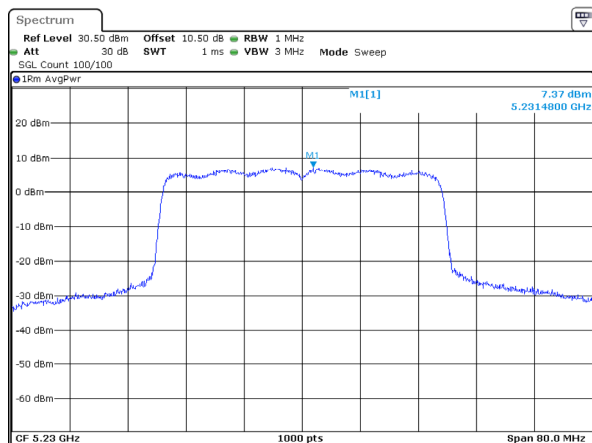
802.11ax40_5230MHz_RU_Full_Chain 3
