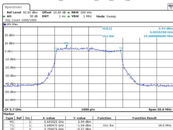
802.11ax20_5700MHz_RU_Full_Chain 2
