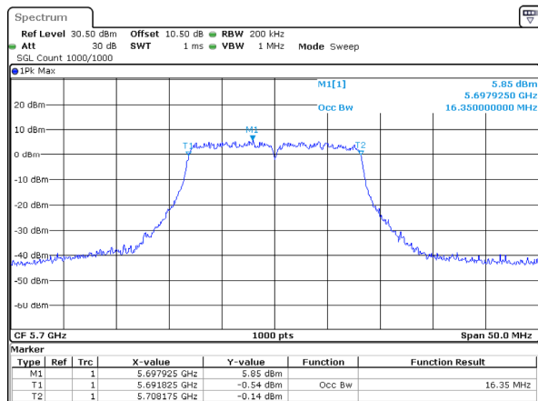
802.11a_5700MHz_Chain 3
