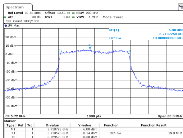
802.11ax20_5720MHz_RU_Full_Chain 0
