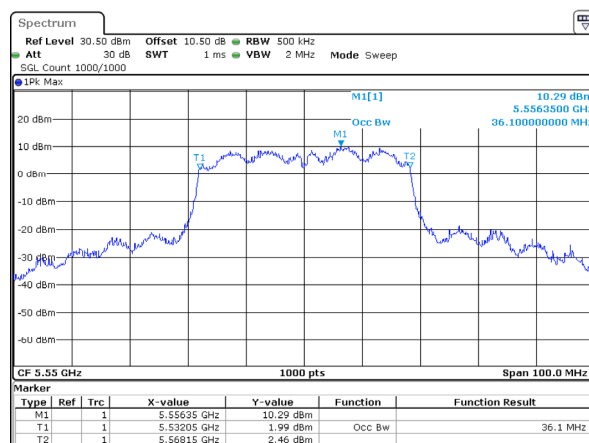
802.11ac40_5550MHz_Chain 3
