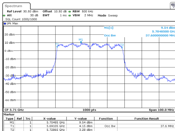
802.11ax40_5710MHz_RU_Full_Chain 3
