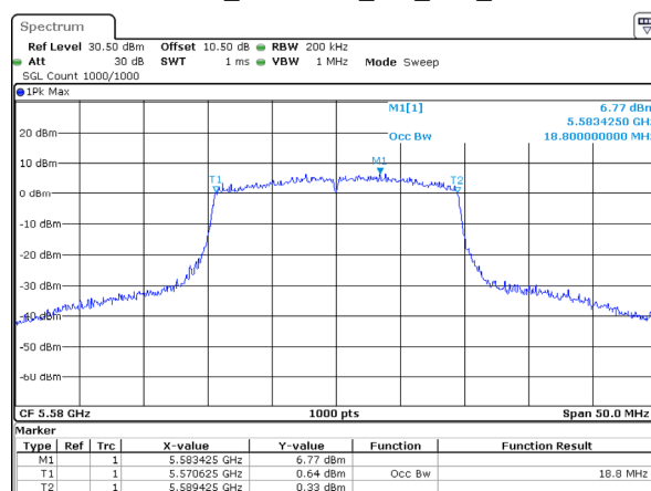
802.11ax20_5580MHz_RU_Full_Chain 1
