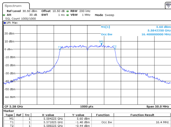
802.11a_5580MHz_Chain 3
