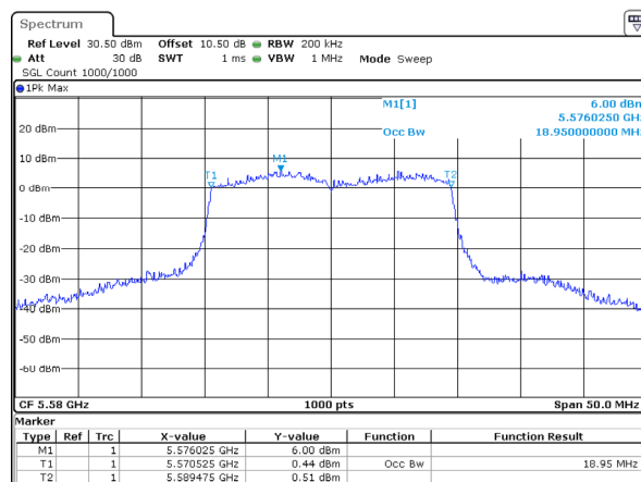
802.11ax20_5580MHz_RU_Full_Chain 0
