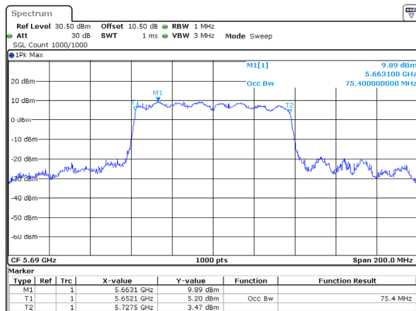
802.11ac80_5690MHz_Chain 0
