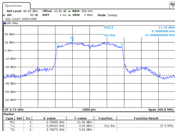
802.11ax40_5710MHz_RU_Full_Chain 1
