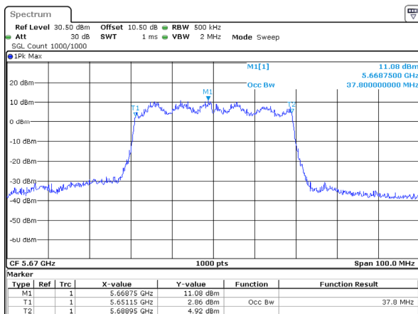
802.11ax40_5670MHz_RU_Full_Chain 3
