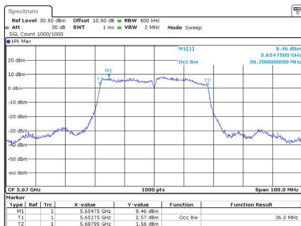
802.11ac40_5670MHz_Chain 2
