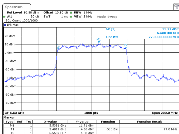
802.11ax80_5530MHz_RU_Full_Chain 2
