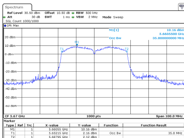
802.11ac40_5670MHz_Chain 1
