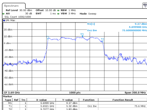
802.11ac80_5690MHz_Chain 2
