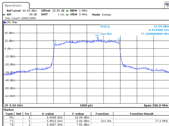
802.11ax80_5530MHz_RU_Full_Chain 1
