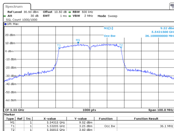
802.11ac40_5550MHz_Chain 1
