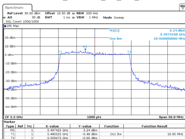
802.11ax20_5500MHz_RU_Full_Chain 1
