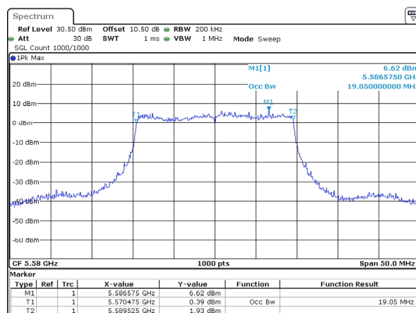
802.11ax20_5580MHz_RU_Full_Chain 2
