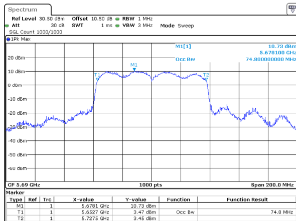
802.11ac80_5690MHz_Chain 1
