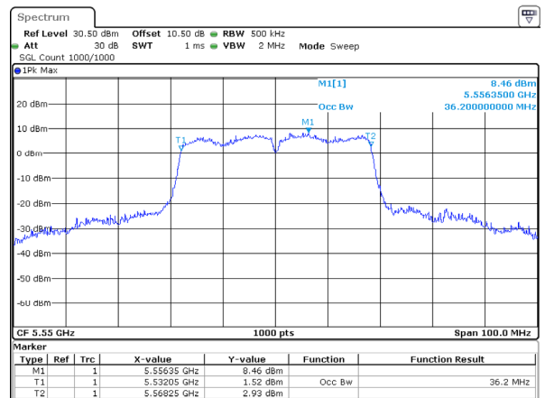
802.11ac40_5550MHz_Chain 0
