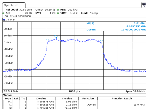
802.11ax20_5700MHz_RU_Full_Chain 3
