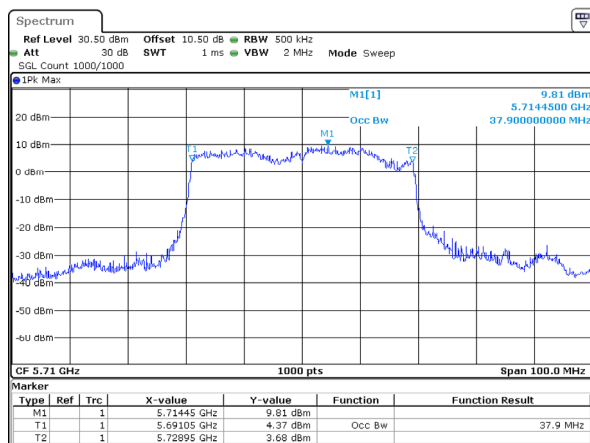
802.11ax40_5710MHz_RU_Full_Chain 2
