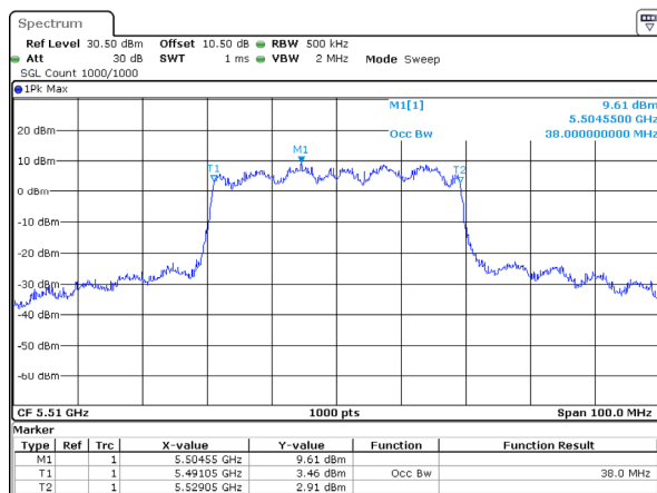
802.11ax40_5510MHz_RU_Full_Chain 3
