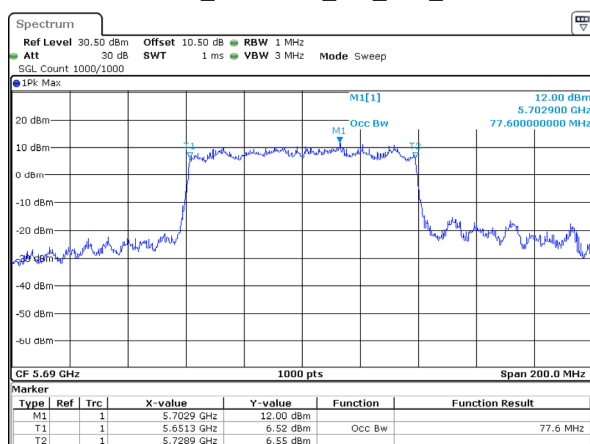
802.11ax80_5690MHz_RU_Full_Chain 2
