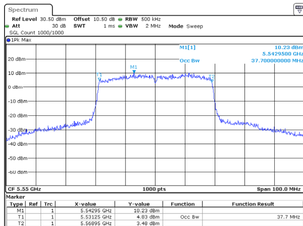
802.11ax40_5550MHz_RU_Full_Chain 1
