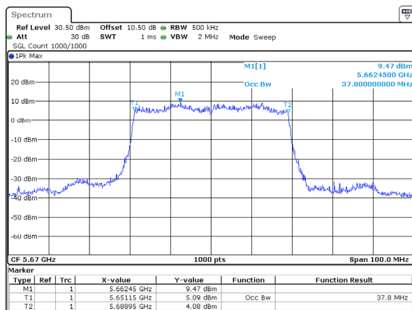
802.11ax40_5670MHz_RU_Full_Chain 2
