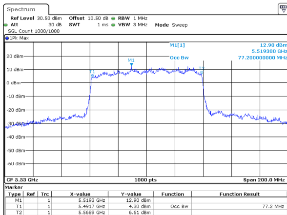
802.11ax80_5530MHz_RU_Full_Chain 0
