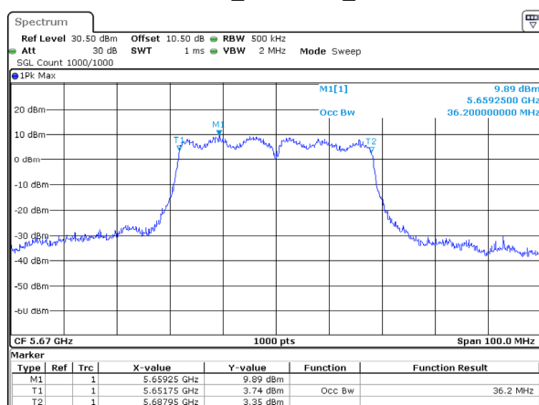
802.11ac40_5670MHz_Chain 3
