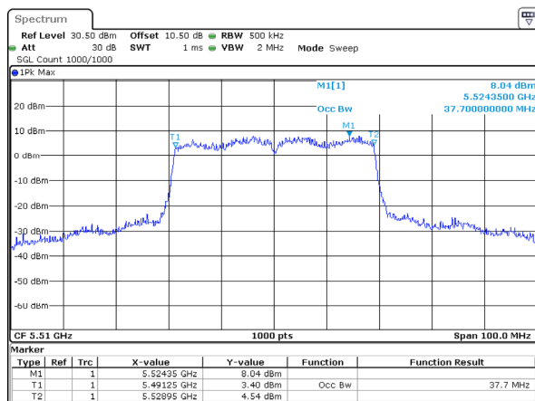
802.11ax40_5510MHz_RU_Full_Chain 0
