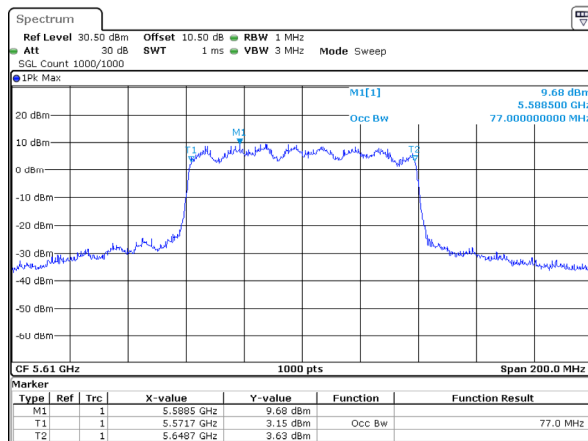
802.11ax80_5610MHz_RU_Full_Chain 0
