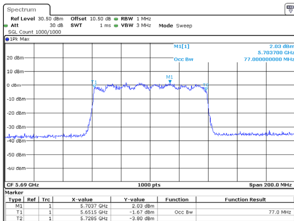
802.11ax80_5690MHz_RU_Full_Chain 0
