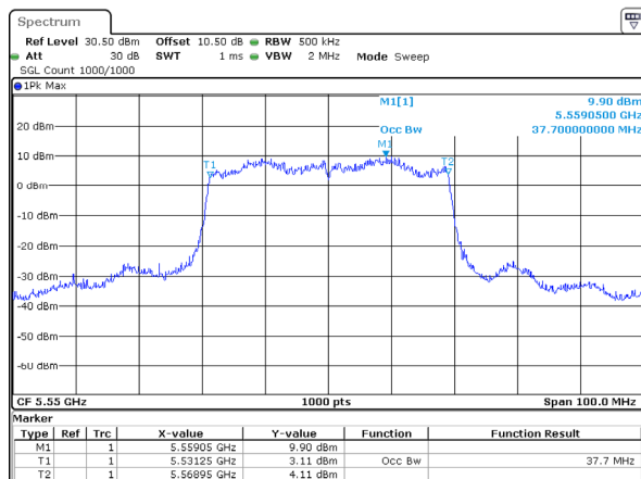
802.11ax40_5550MHz_RU_Full_Chain 2
