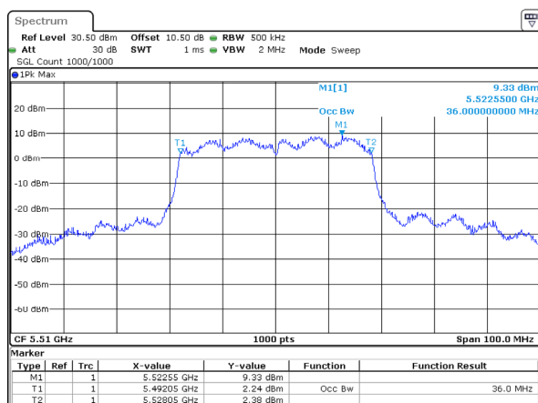
802.11ac40_5510MHz_Chain 3
