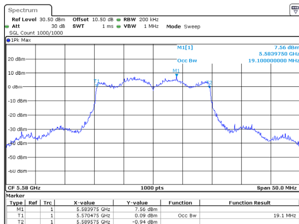
802.11ax20_5580MHz_RU_Full_Chain 3
