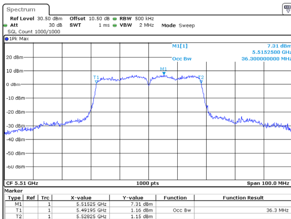
802.11ac40_5510MHz_Chain 0
