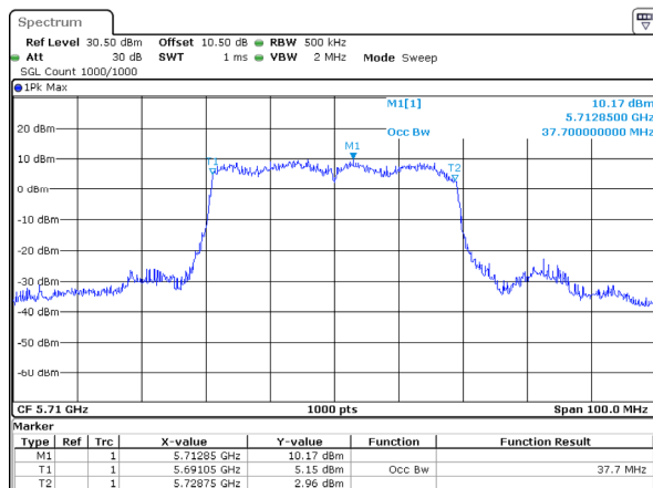
802.11ax40_5710MHz_RU_Full_Chain 0
