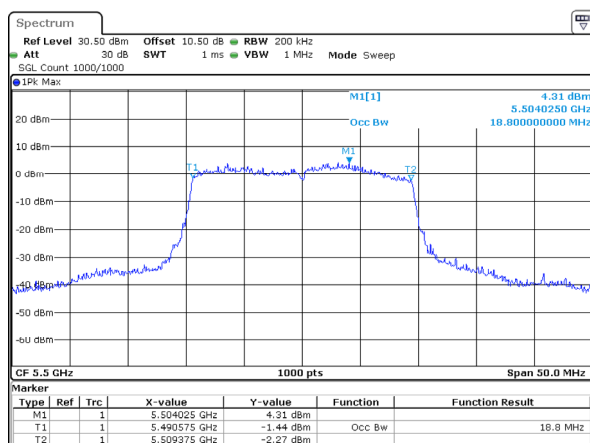
802.11ax20_5500MHz_RU_Full_Chain 2
