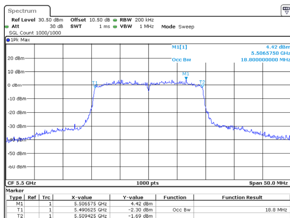
802.11ax20_5500MHz_RU_Full_Chain 0
