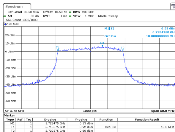
802.11ax20_5720MHz_RU_Full_Chain 1
