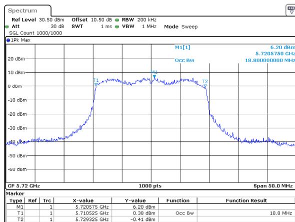
802.11ax20_5720MHz_RU_Full_Chain 3
