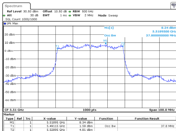
802.11ax40_5510MHz_RU_Full_Chain 2
