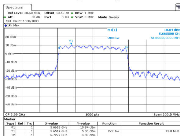
802.11ac80_5690MHz_Chain 3
