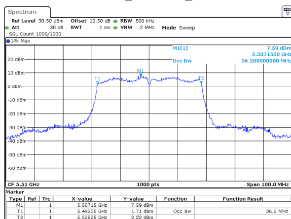
802.11ac40_5510MHz_Chain 2
