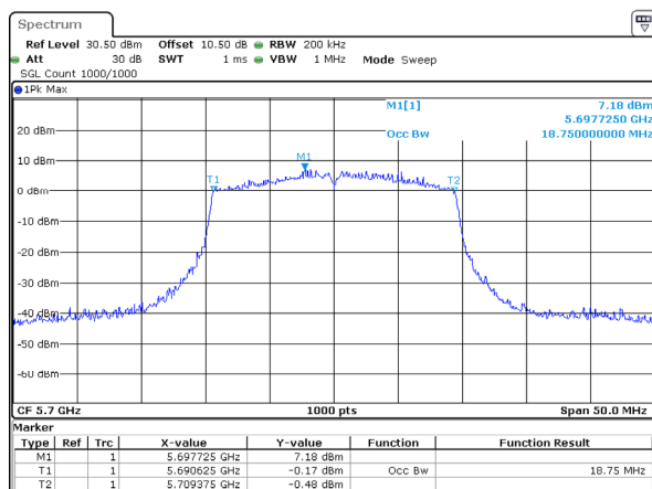
802.11ax20_5700MHz_RU_Full_Chain 1
