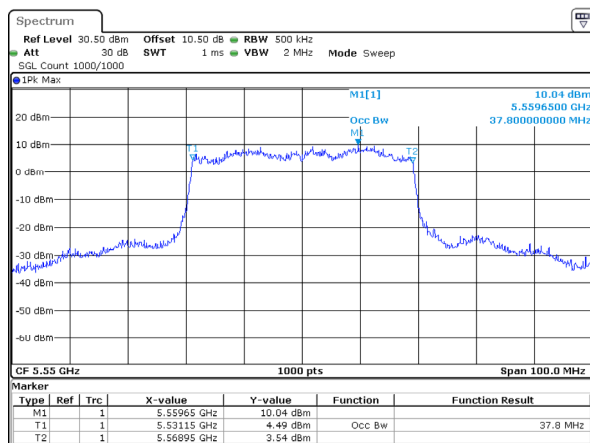
802.11ax40_5550MHz_RU_Full_Chain 0
