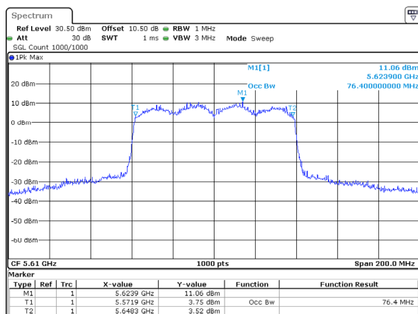
802.11ax80_5610MHz_RU_Full_Chain 1
