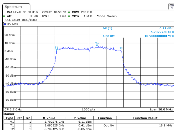
802.11ax20_5700MHz_RU_Full_Chain 0
