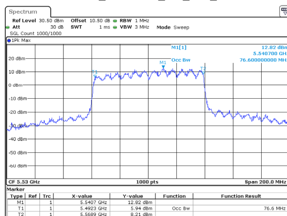
802.11ax80_5530MHz_RU_Full_Chain 3
