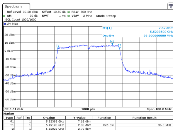
802.11ac40_5510MHz_Chain 1
