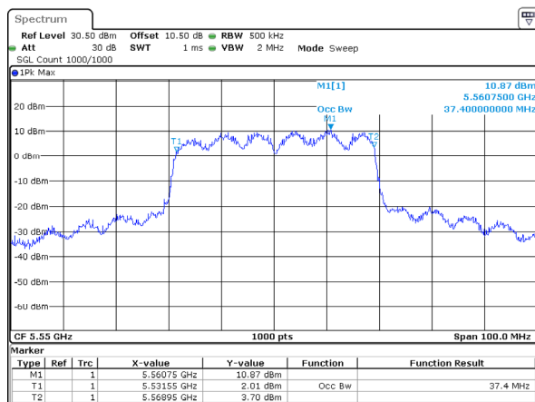
802.11ax40_5550MHz_RU_Full_Chain 3
