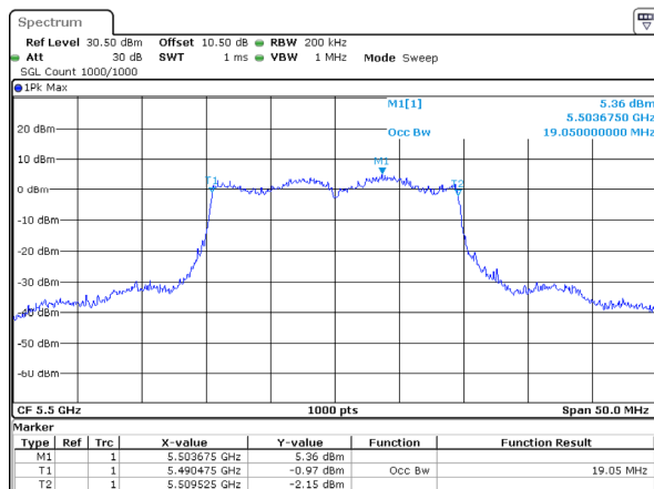
802.11ax20_5500MHz_RU_Full_Chain 3
