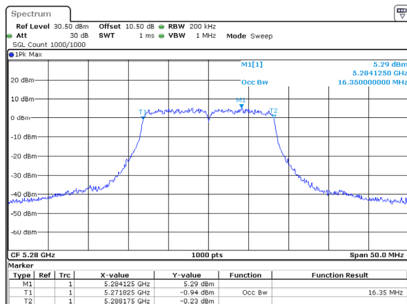
802.11a_5280MHz_Chain 2
