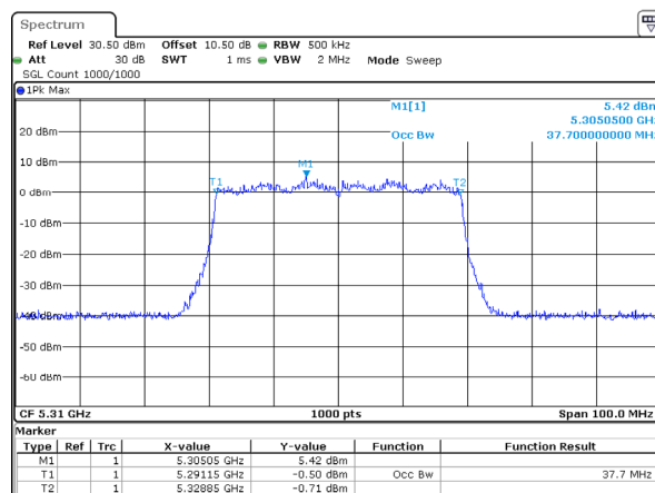
802.11ax40_5310MHz_RU_Full_Chain 3
