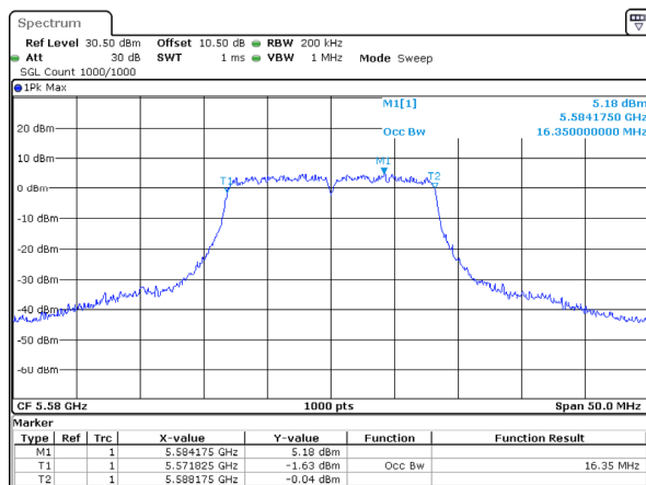
802.11a_5580MHz_Chain 2
