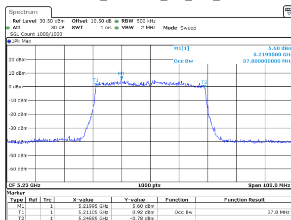
802.11ax40_5230MHz_RU_Full_Chain 2
