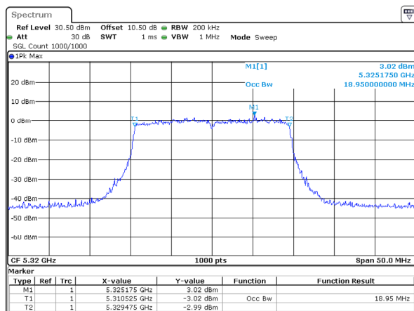
802.11ax20_5320MHz_RU_Full_Chain 0
