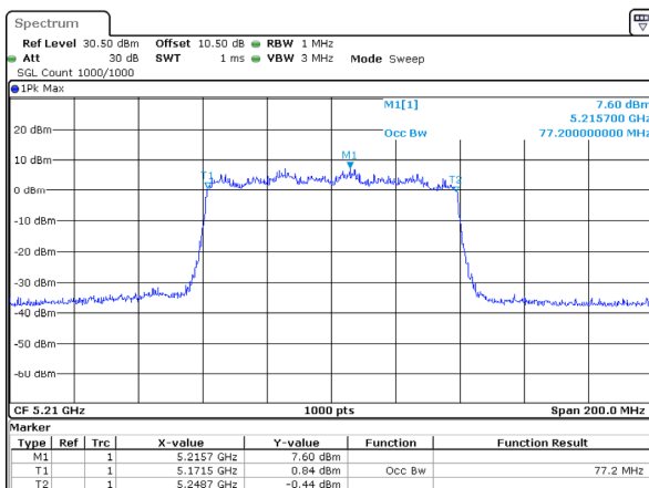
802.11ax80_5210MHz_RU_Full_Chain 2
