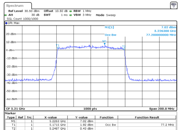
802.11ax80_5210MHz_RU_Full_Chain 1
