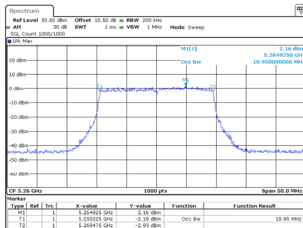
802.11ax20_5260MHz_RU_Full_Chain 1
