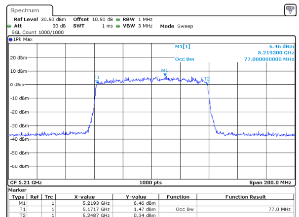
802.11ax80_5210MHz_RU_Full_Chain 3
