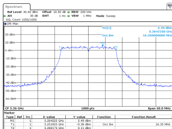
802.11a_5260MHz_Chain 1
