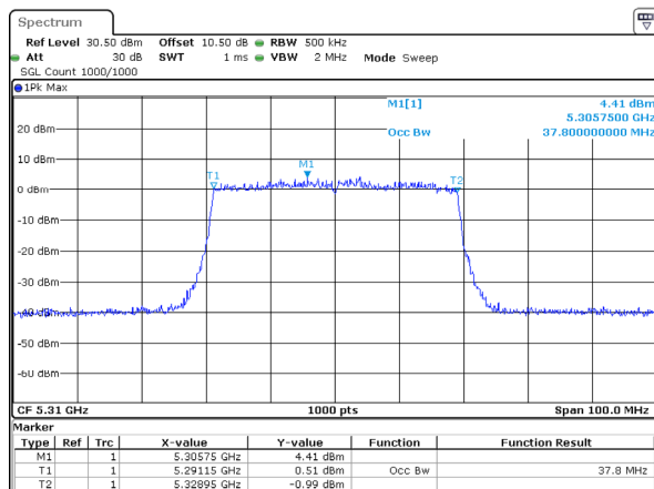
802.11ax40_5310MHz_RU_Full_Chain 0
