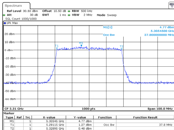
802.11ax40_5310MHz_RU_Full_Chain 1
