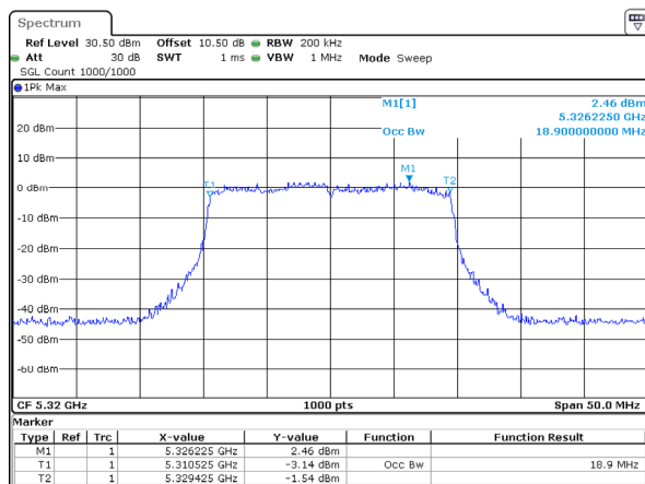
802.11ax20_5320MHz_RU_Full_Chain 3
