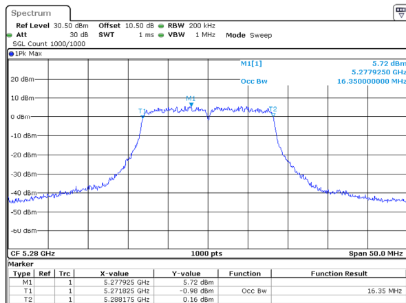
802.11a_5280MHz_Chain 3
