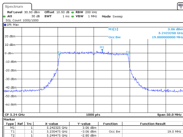
802.11ax20_5240MHz_RU_Full_Chain 2
