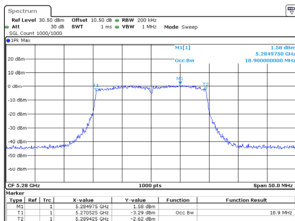
802.11ax20_5280MHz_RU_Full_Chain 2
