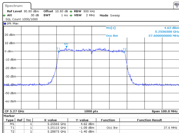
802.11ax40_5270MHz_RU_Full_Chain 2
