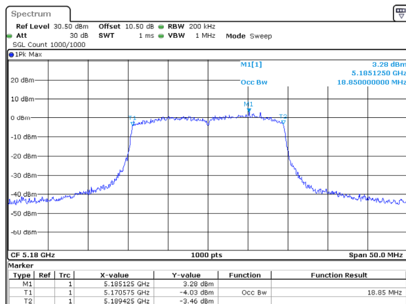
802.11ax20_5180MHz_RU_Full_Chain 2
