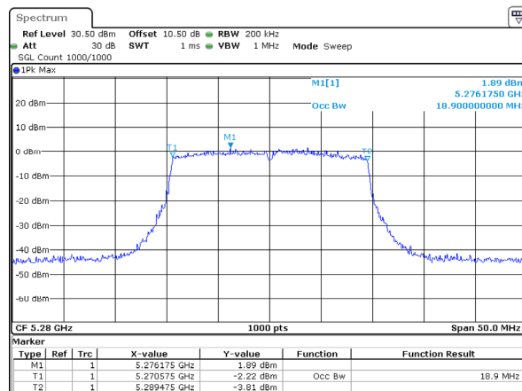
802.11ax20_5280MHz_RU_Full_Chain 0
