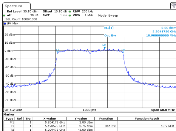
802.11ax20_5200MHz_RU_Full_Chain 2
