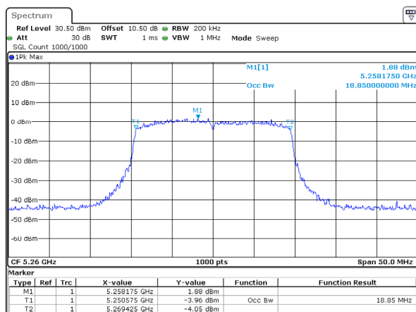
802.11ax20_5260MHz_RU_Full_Chain 2
