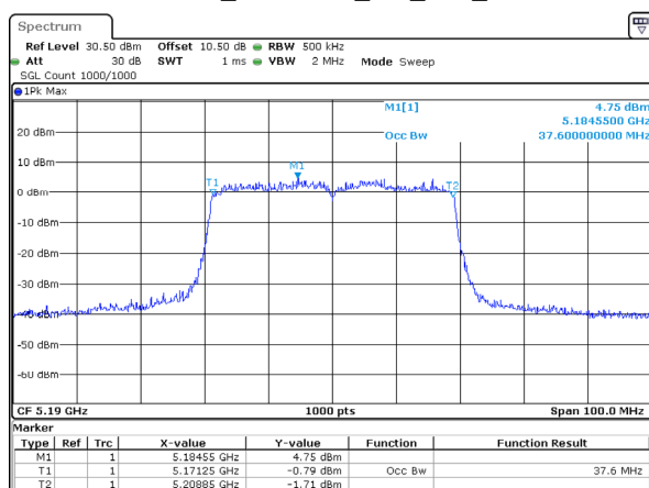
802.11ax40_5190MHz_RU_Full_Chain 2
