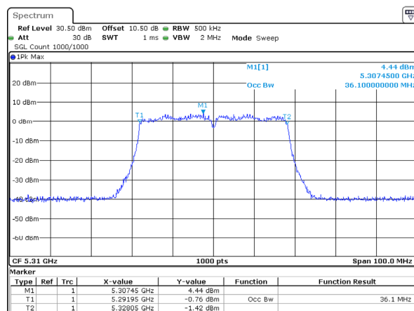
802.11ac40_5310MHz_Chain 3
