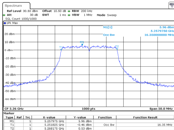
802.11a_5260MHz_Chain 3
