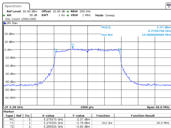
802.11ax20_5280MHz_RU_Full_Chain 3
