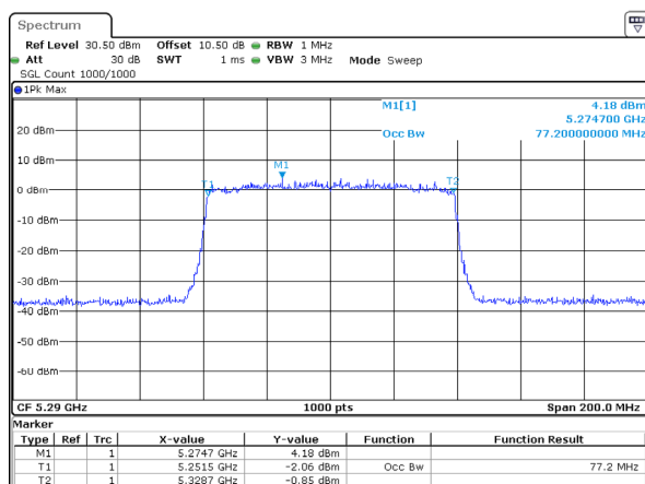
802.11ax80_5290MHz_RU_Full_Chain 0
