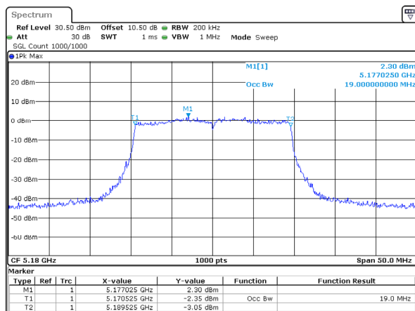
802.11ax20_5180MHz_RU_Full_Chain 3
