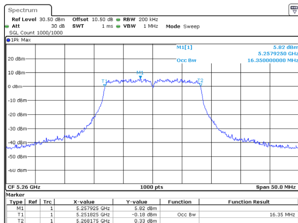
802.11a_5260MHz_Chain 2
