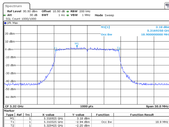
802.11ax20_5320MHz_RU_Full_Chain 1
