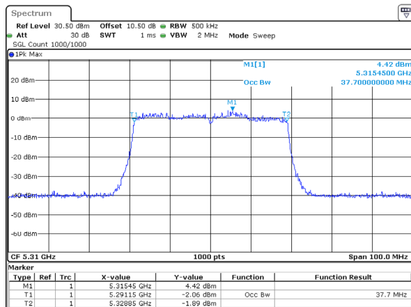
802.11ax40_5310MHz_RU_Full_Chain 2
