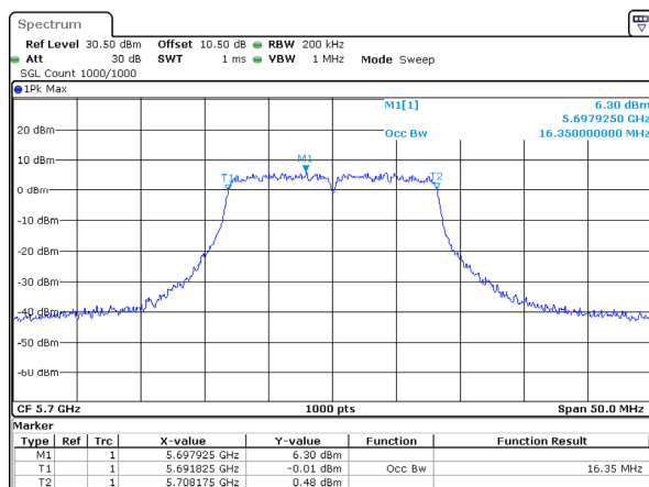
802.11a_5700MHz_Chain 1
