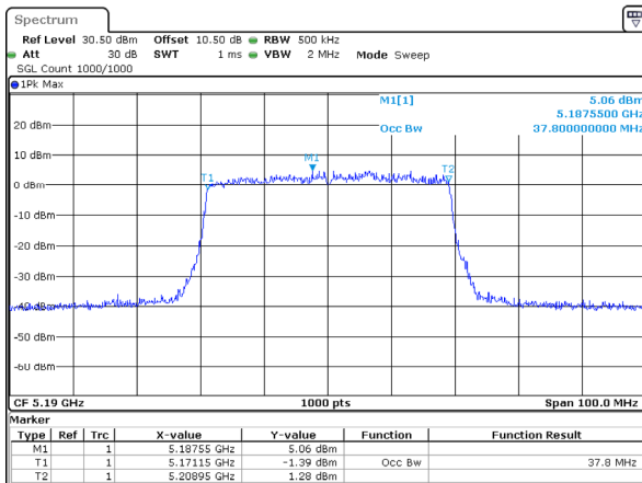
802.11ax40_5190MHz_RU_Full_Chain 3
