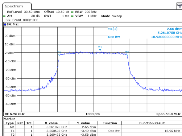
802.11ax20_5260MHz_RU_Full_Chain 0
