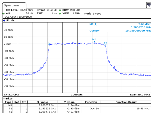
802.11ax20_5200MHz_RU_Full_Chain 3
