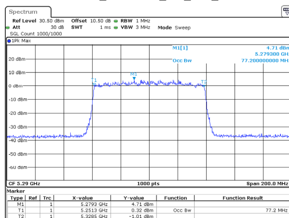
802.11ax80_5290MHz_RU_Full_Chain 3
