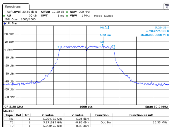
802.11a_5280MHz_Chain 1
