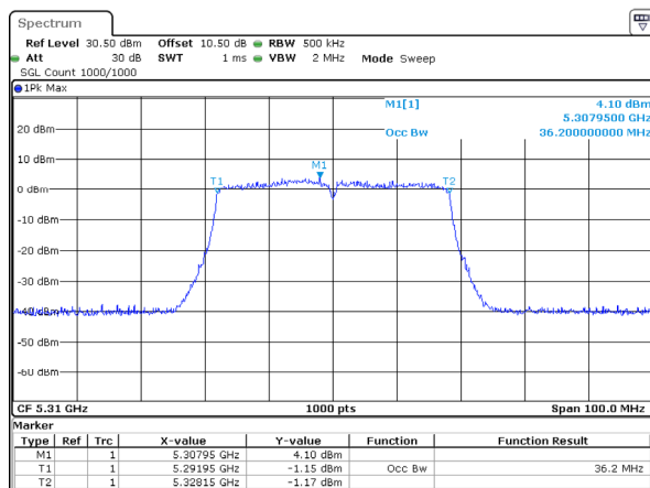
802.11ac40_5310MHz_Chain 1
