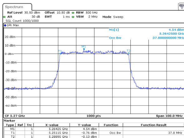
802.11ax40_5270MHz_RU_Full_Chain 3
