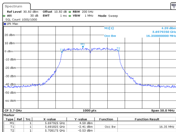
802.11a_5700MHz_Chain 2
