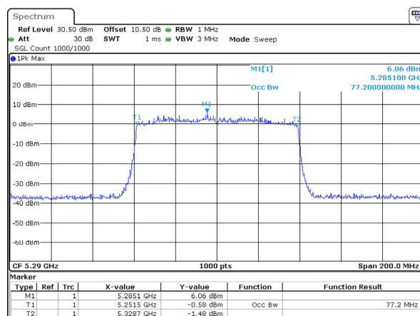
802.11ax80_5290MHz_RU_Full_Chain 1
