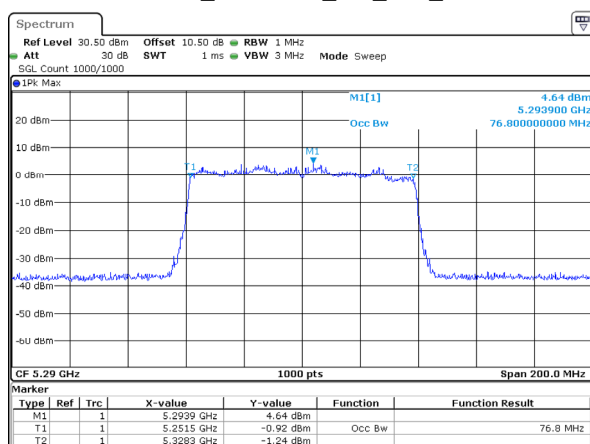
802.11ax80_5290MHz_RU_Full_Chain 2
