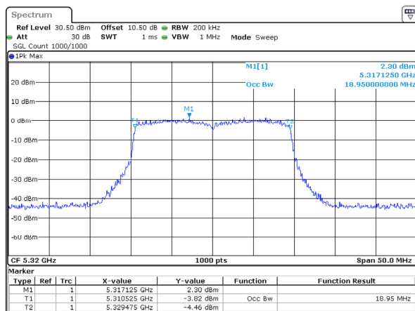
802.11ax20_5320MHz_RU_Full_Chain 2
