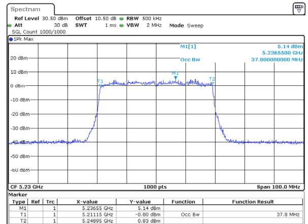
802.11ax40_5230MHz_RU_Full_Chain 3
