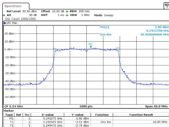
802.11ax20_5240MHz_RU_Full_Chain 3
