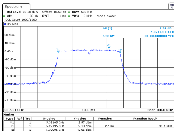
802.11ac40_5310MHz_Chain 0
