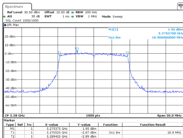
802.11ax20_5280MHz_RU_Full_Chain 1
