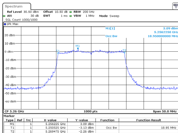
802.11ax20_5260MHz_RU_Full_Chain 3
