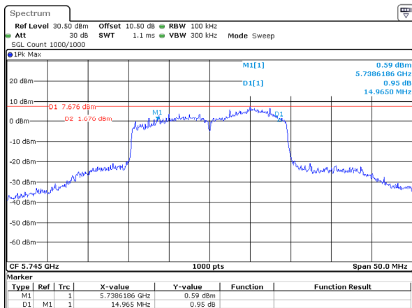
802.11ax20_5745MHz_RU_Full_Chain 2
