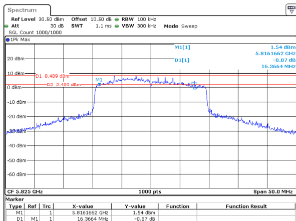
802.11ax20_5825MHz_RU_Full_Chain 1
