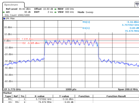
802.11ax80_5775MHz_RU_Full_Chain 3
