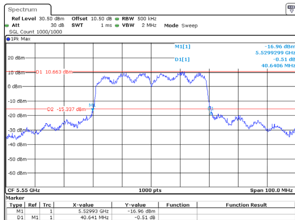
802.11ax40_5550MHz_RU_Full_Chain 3
