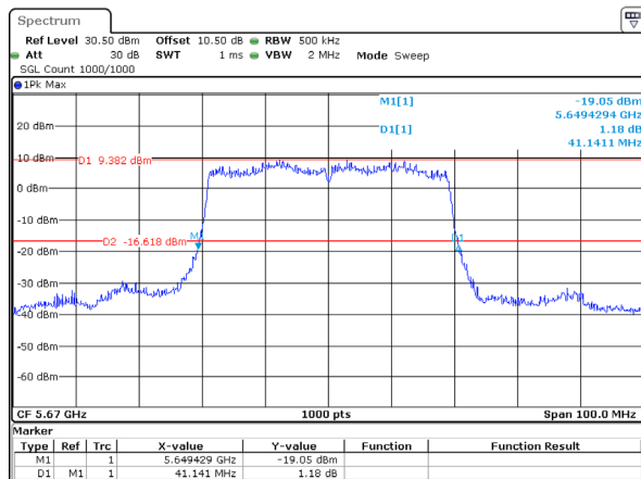
802.11ax40_5670MHz_RU_Full_Chain 2
