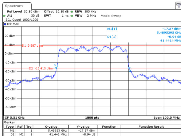
802.11ax40_5510MHz_RU_Full_Chain 3
