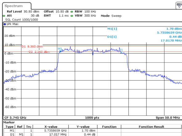
802.11ax20_5745MHz_RU_Full_Chain 3
