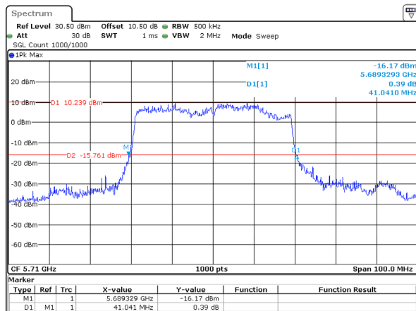
802.11ax40_5710MHz_RU_Full_Chain 2
