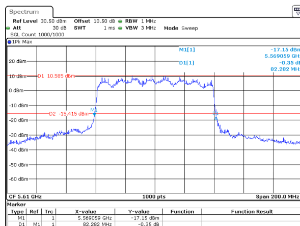
802.11ax80_5610MHz_RU_Full_Chain 0
