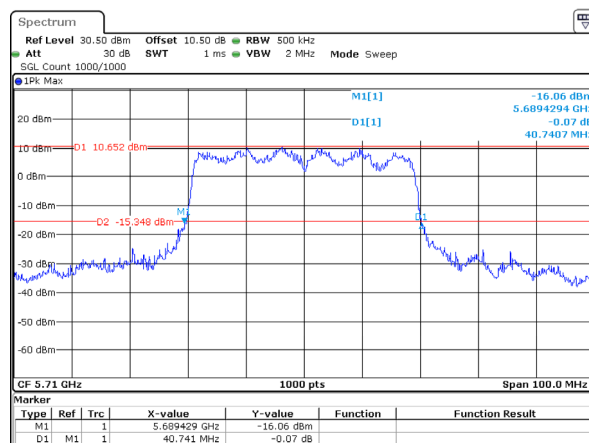
802.11ax40_5710MHz_RU_Full_Chain 3
