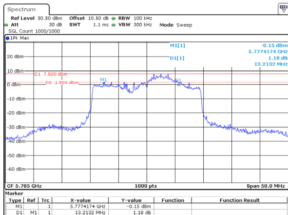
802.11ax20_5785MHz_RU_Full_Chain 2
