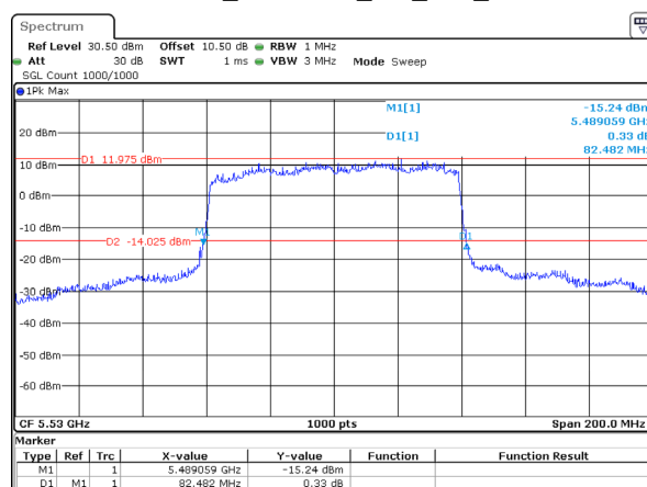
802.11ax80_5530MHz_RU_Full_Chain 1
