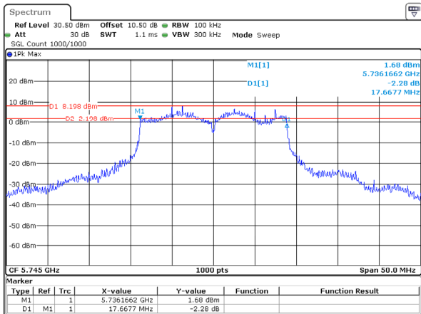
802.11ac20_5745MHz_Chain 3
