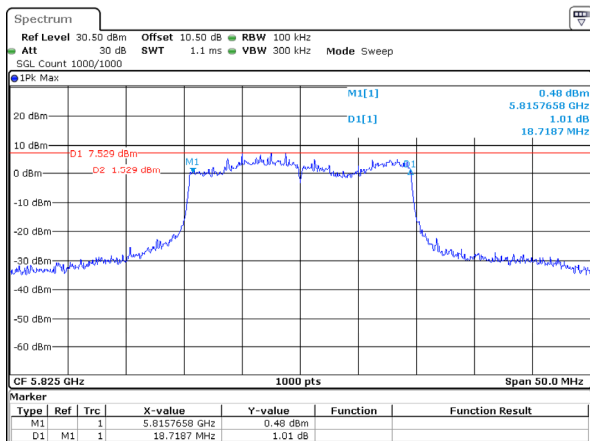
802.11ax20_5825MHz_RU_Full_Chain 2
