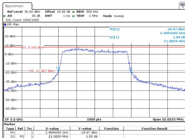
802.11ax20_5500MHz_RU_Full_Chain 1
