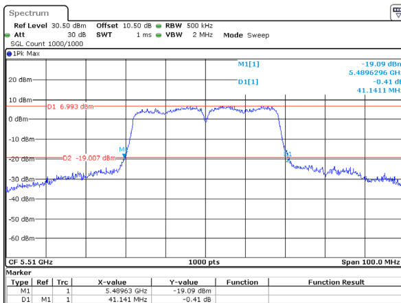
802.11ac40_5510MHz_Chain 0
