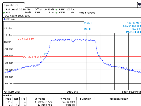
802.11a_5580MHz_Chain 2
