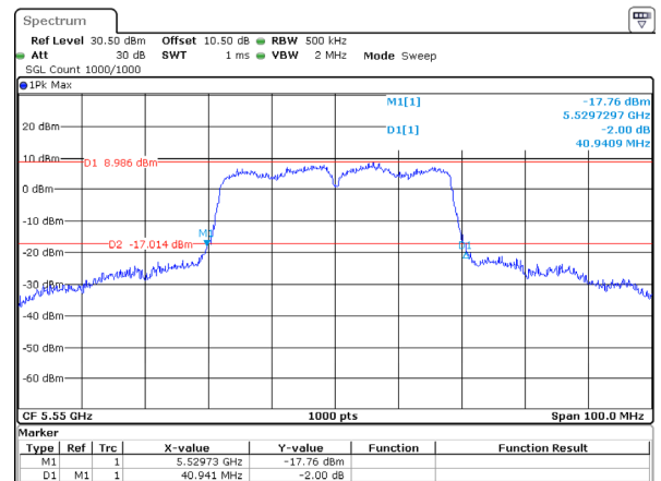
802.11ac40_5550MHz_Chain 0
