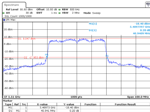
802.11ax40_5510MHz_RU_Full_Chain 0
