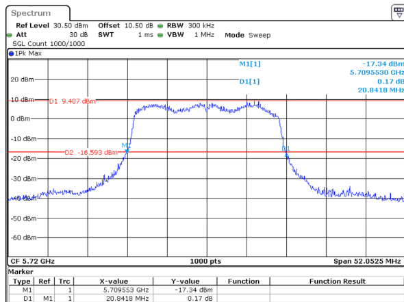
802.11ax20_5720MHz_RU_Full_Chain 3
