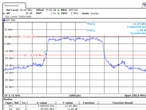
802.11ax40_5710MHz_RU_Full_Chain 0
