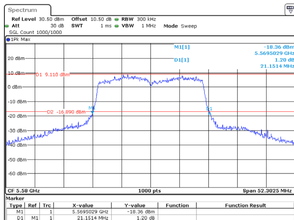
802.11ax20_5580MHz_RU_Full_Chain 0
