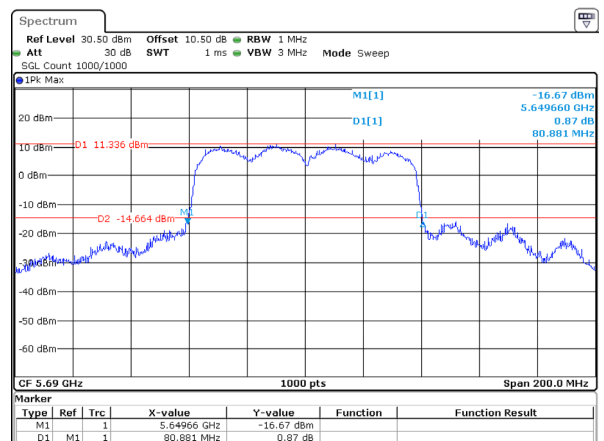
802.11ac80_5690MHz_Chain 1
