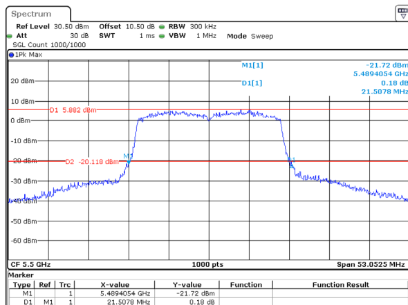
802.11ax20_5500MHz_RU_Full_Chain 0
