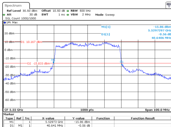
802.11ax40_5550MHz_RU_Full_Chain 0
