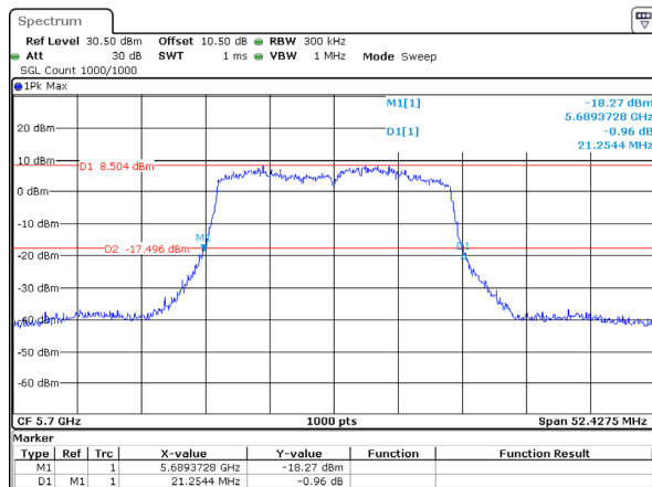
802.11ax20_5700MHz_RU_Full_Chain 0
