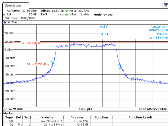
802.11ax20_5720MHz_RU_Full_Chain 0
