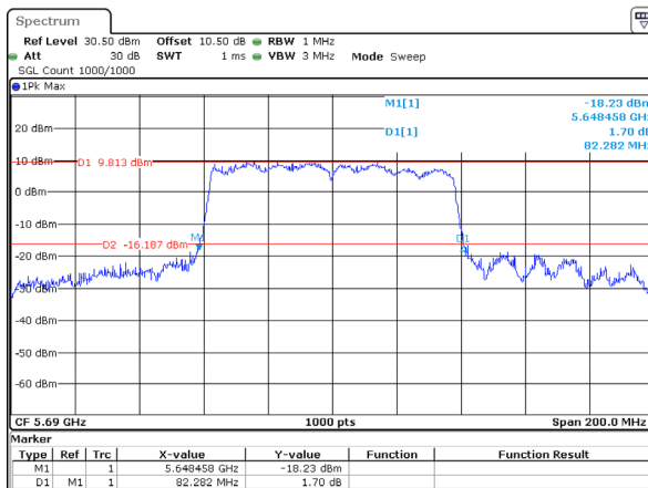
802.11ac80_5690MHz_Chain 0
