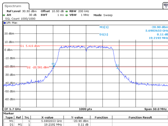
802.11a_5700MHz_Chain 3
