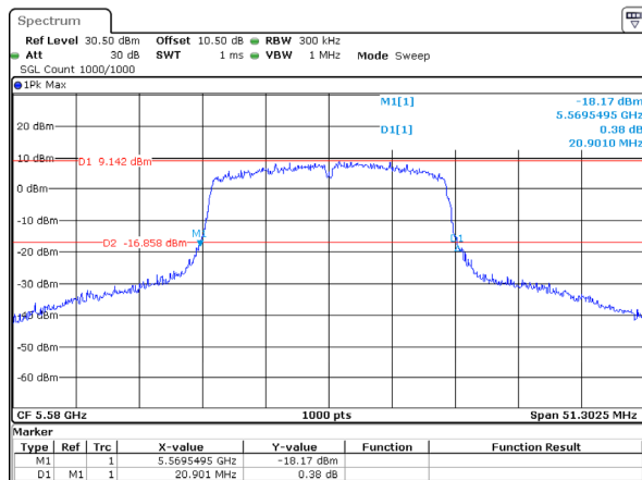
802.11ax20_5580MHz_RU_Full_Chain 1
