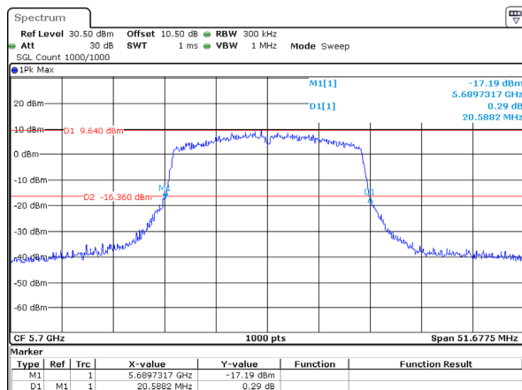
802.11ax20_5700MHz_RU_Full_Chain 1
