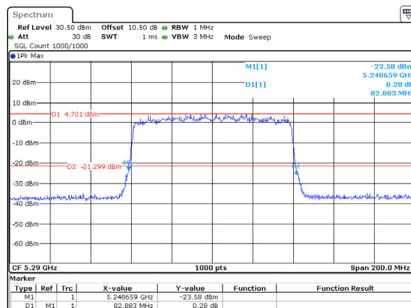
802.11ax80_5290MHz_RU_Full_Chain 3
