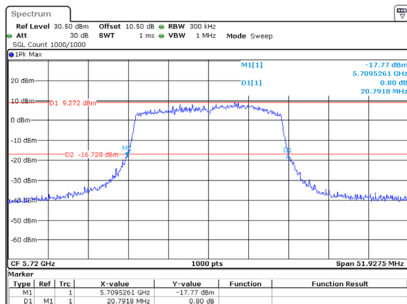
802.11ax20_5720MHz_RU_Full_Chain 1
