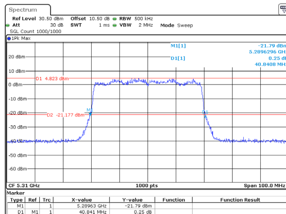
802.11ax40_5310MHz_RU_Full_Chain 3
