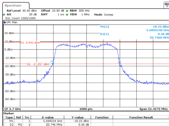
802.11ax20_5700MHz_RU_Full_Chain 3
