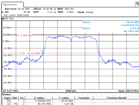
802.11ac40_5670MHz_Chain 0
